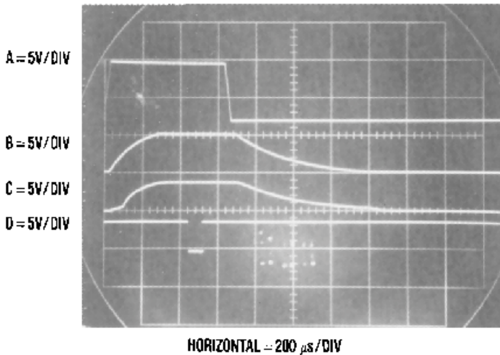
Figure 22. Low Power Strain Gauge Bridge Signal Conditioning Waveforms
