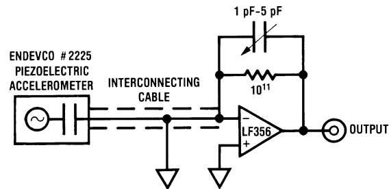
Figure 11. Piezoelectric Accelerometer
