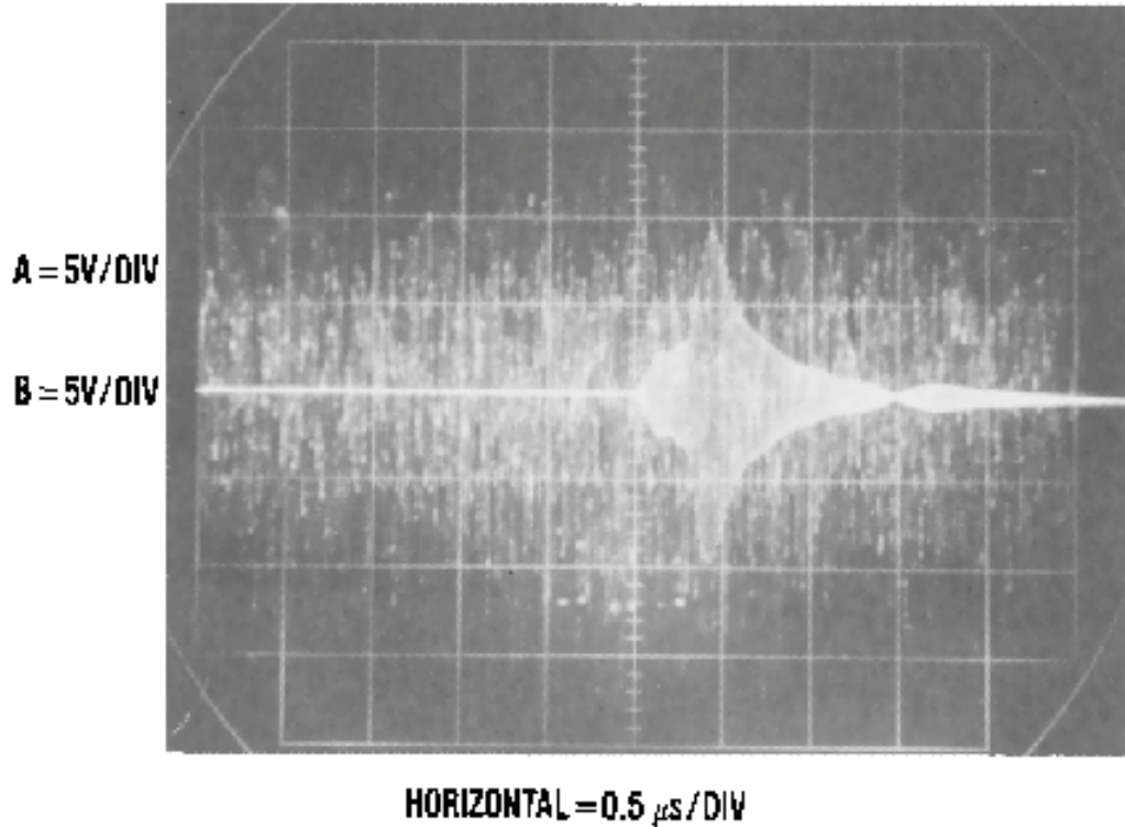
Figure 10. Amplified Output of the Received Pulse Superimposed on the Output of a Broadband Microphone Placed in the Sonic Path
