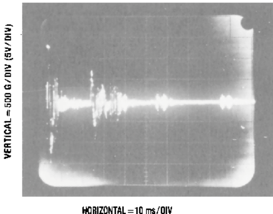
Figure 12. Accelerometer is Mounted on a HandHheld Voltmeter and Dropped on the Floor
