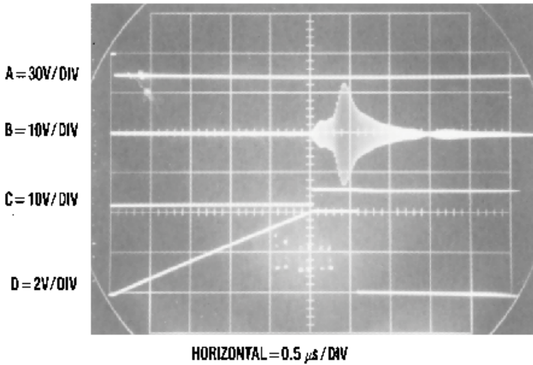
Figure 9. Waveform Pulses
