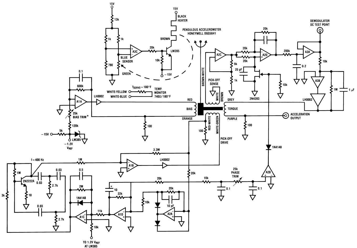
Figure 16. Force-Balanced Pendulous Accelerometer
