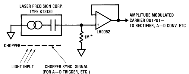
Figure 6. Slower Detector Terminates into 1 MΩ and is Unloaded by the LH0052 Low Bias FET Amplifier
