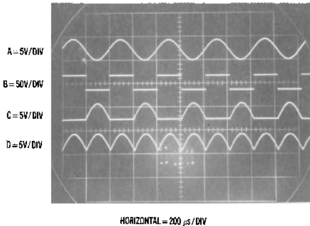
Figure 15. LVDT Waveforms
