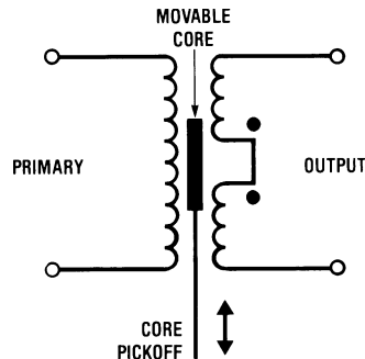
Figure 13. Transformer
