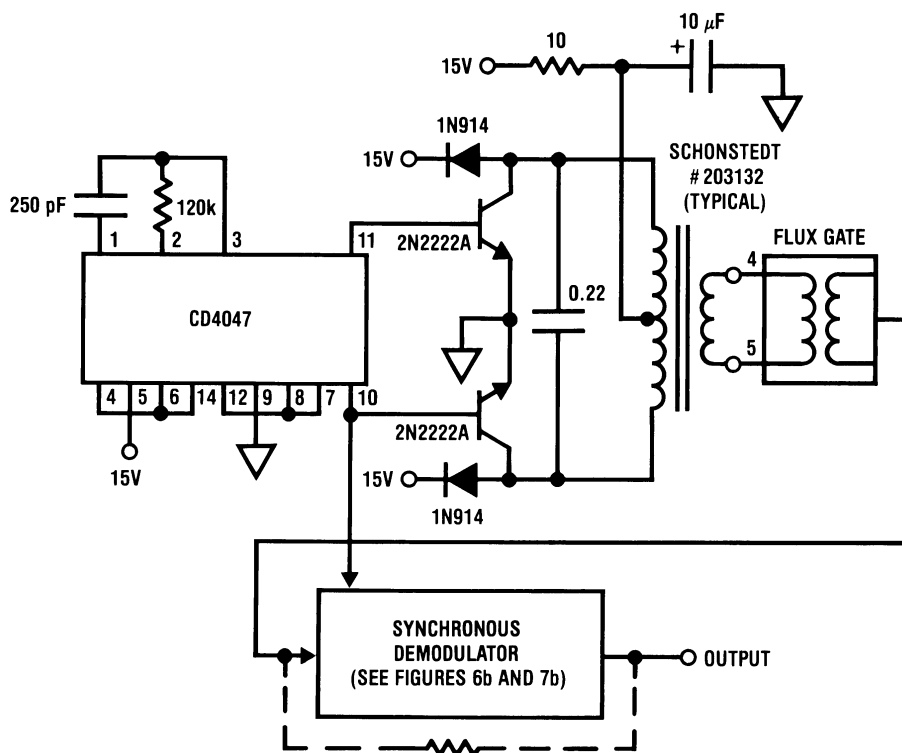
Figure 20. Simple Flux Gate and Signal Conditioning
