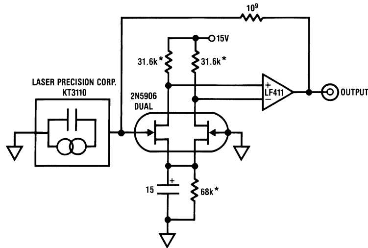
Figure 7. Current Mode Signal Conditioning Circuit
