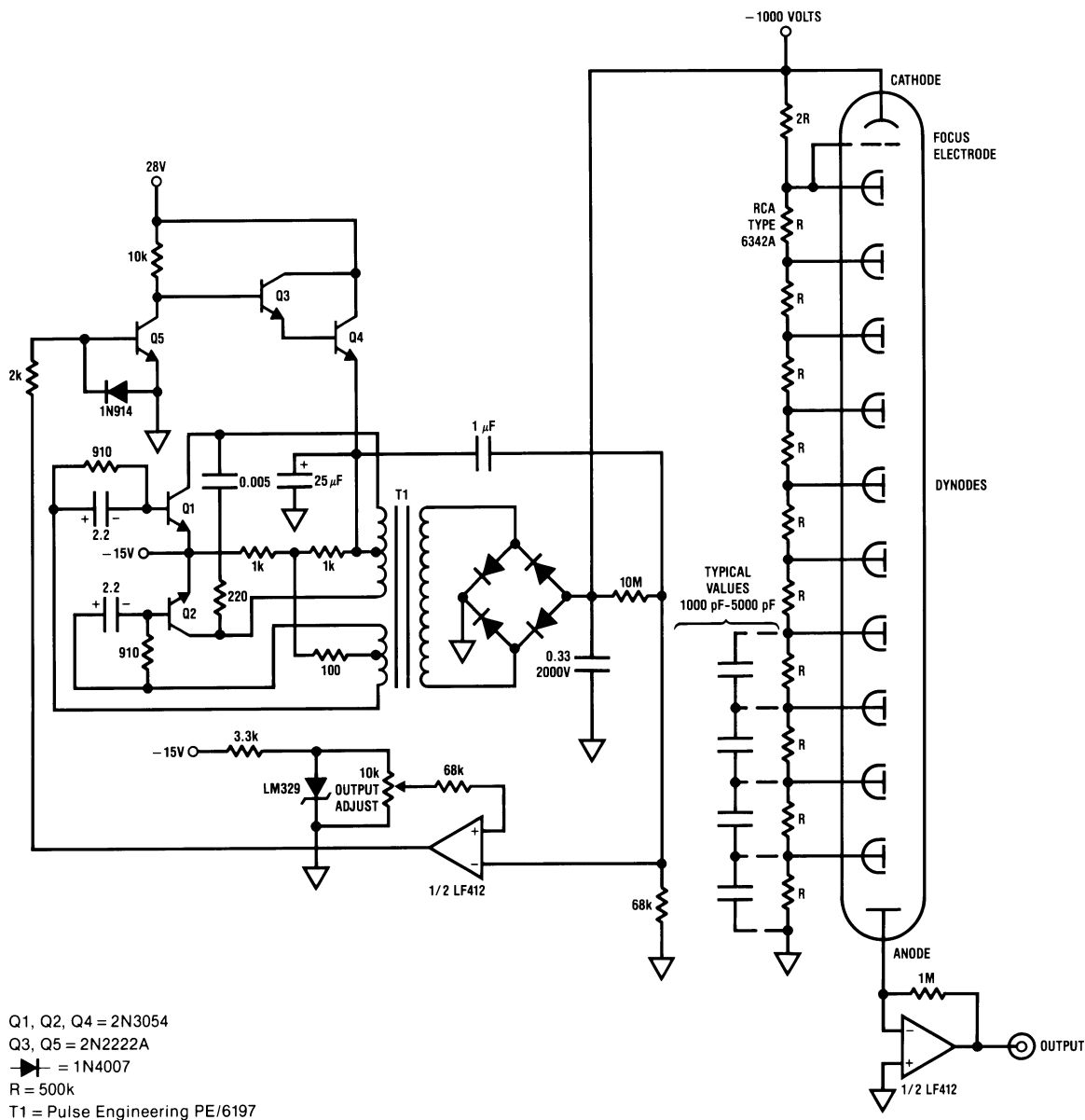
Figure 1. Typical PMT and Conditioning Circuit
