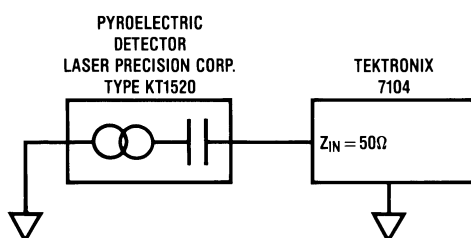
Figure 5. Simple Voltage Mode Set-Up
