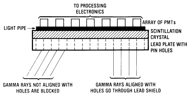
Figure 3. Lead Plate in Front of Gamma Camera
