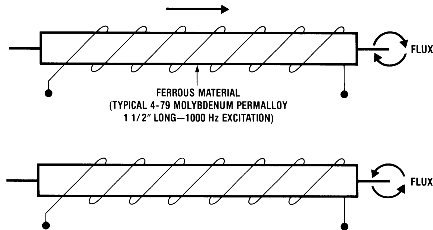
Figure 19. Flux Gate
