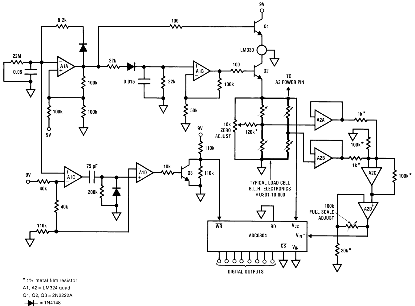
Figure 21. Complete Signal Conditioning for Strain Gauge Transducers
