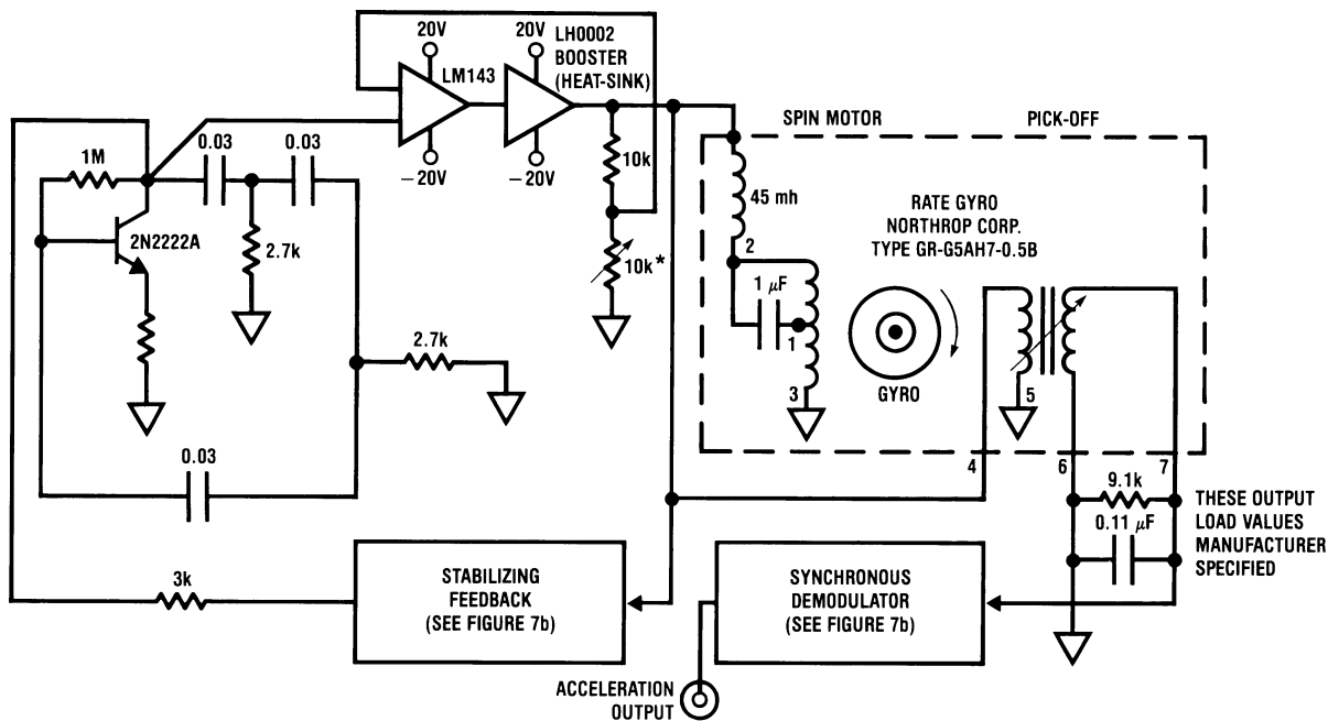
Figure 18. Signal Conditioning for a Typical Rate Gyro
