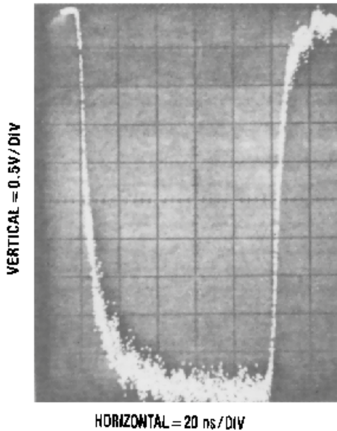
Figure 2. Actual Rise and Fall Time Characteristics (Inverted) of a Fast Pulse of Light Produced by an LED
