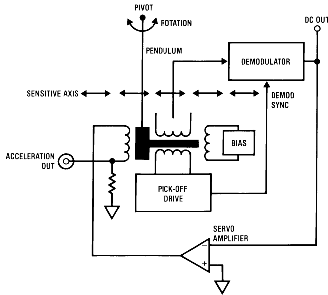
Figure 16. Force-Balanced Pendulous Accelerometer
