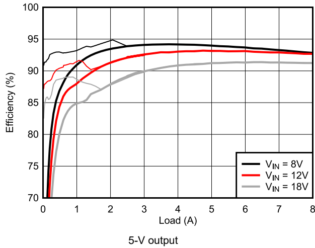
Figure 9-6. Efficiency versus I_{OUT}
