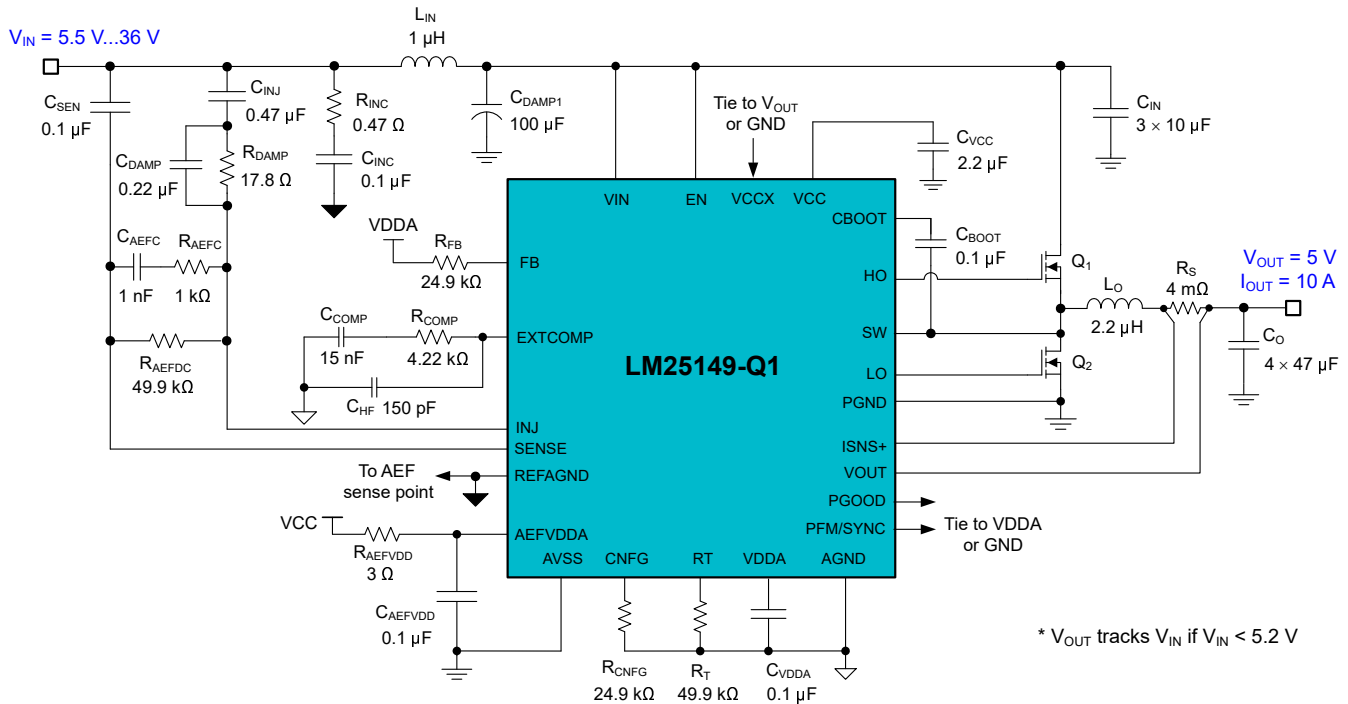
Figure 9-18. Application Circuit 1 With LM25149-Q1 Buck Regulator at 440 kHz
