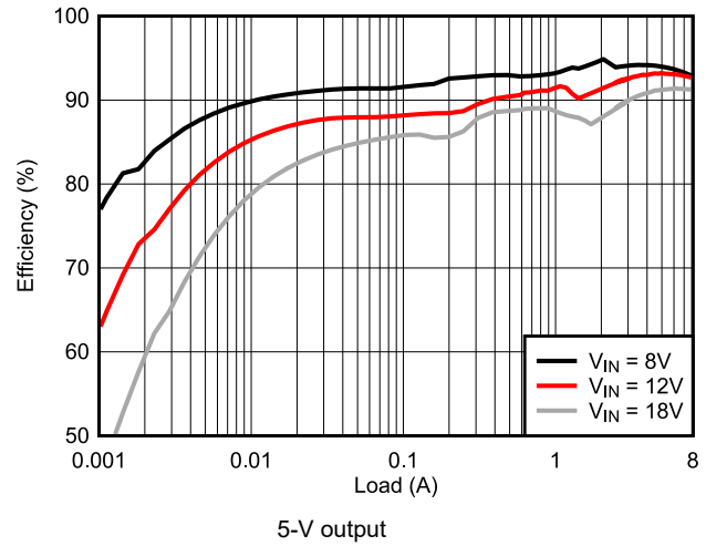
Figure 9-7. Efficiency versus I_{OUT} , Log Scale
