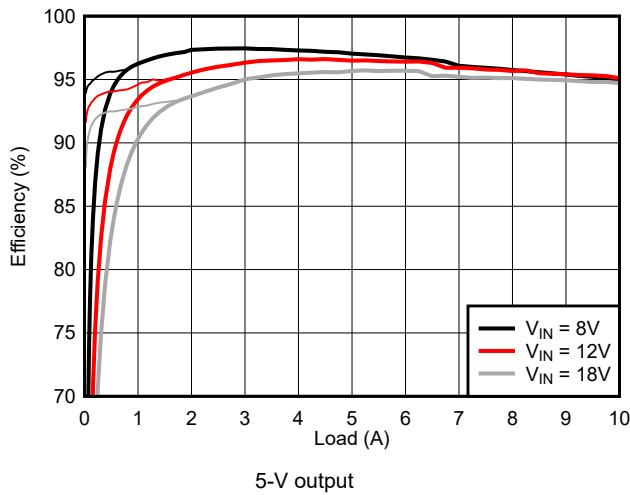
Figure 9-19. Efficiency versus I_{OUT}
