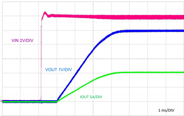
Figure 9-25. Start-Up Characteristic
