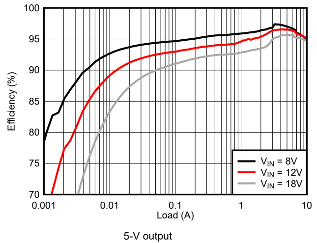
Figure 9-20. Efficiency versus I_{OUT} , Log Scale
