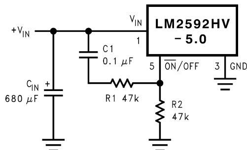
Figure 21. Delayed Start-Up
