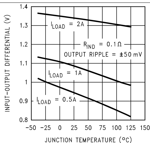
Figure 6. Dropout Voltage
