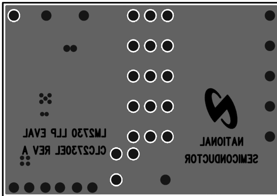
Figure 5. Bottom Layer
