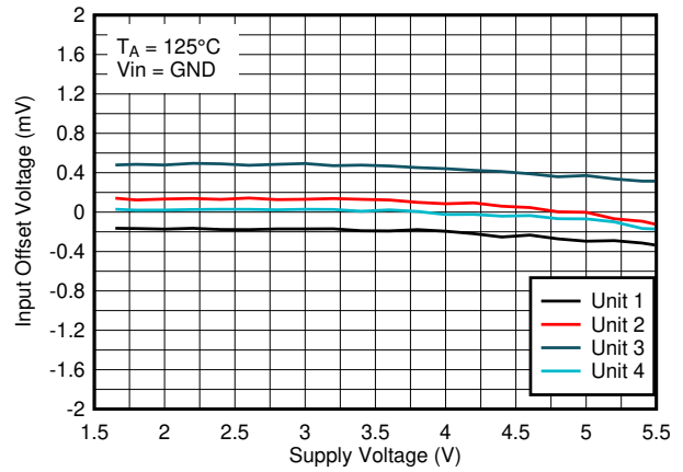
Figure 6-26. Offset Voltage vs. Supply Voltage at 125°C, VIN=0V
