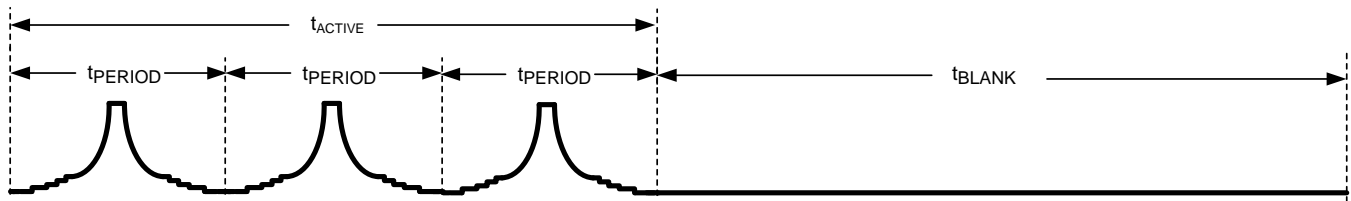
Figure 13. Multiple Pulse with Dead Time
