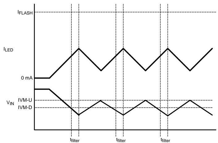
Figure 9. Adjust Up and Down Mode
