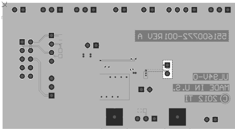
Figure 5. Bottom Layer (unmirrored)
