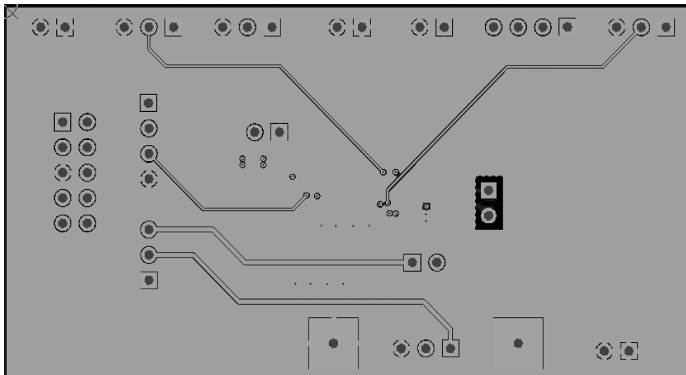
Figure 4. Mid-Layer 2
