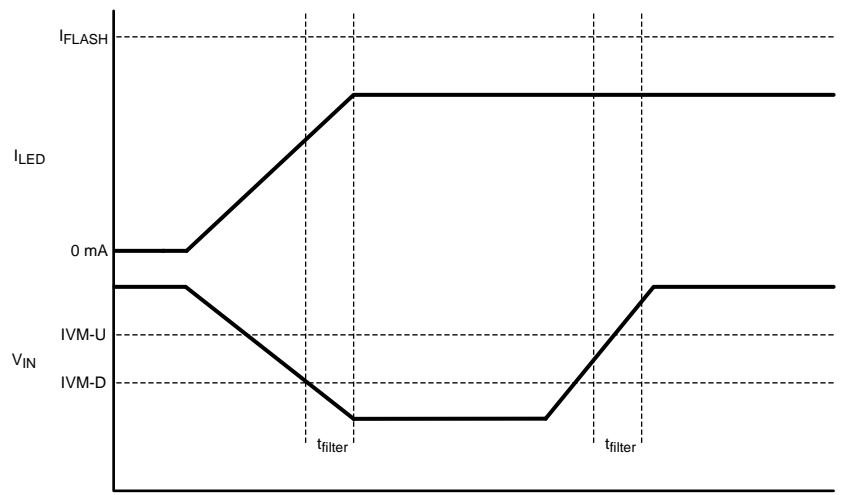
Figure 7. Stop and Hold Mode
