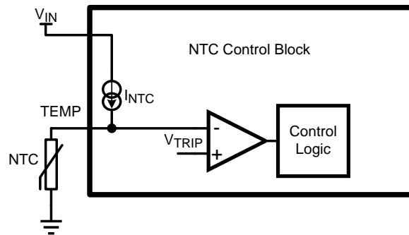
Figure 10. NTC Control Block
