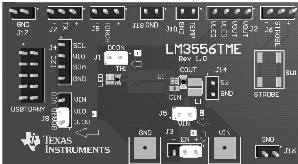
Figure 1. LM3556 Evaluation Board
