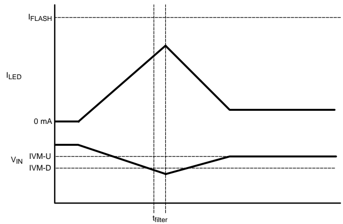
Figure 8. Adjust Down Only Mode
