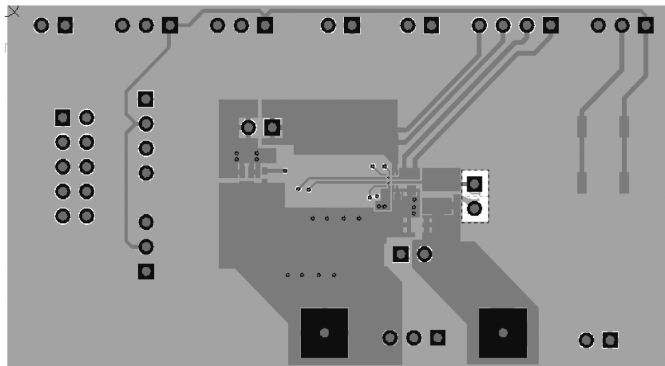
Figure 2. Top Layer
