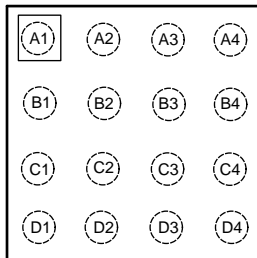
YFQ Package 16-Pin DSBGA Top View
