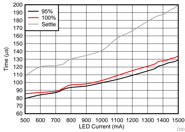
Figure 5. Boost-Mode Rise and Settling Times
