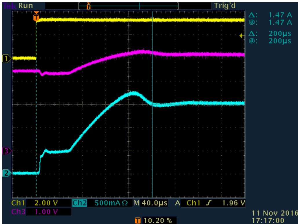
Figure 2. Boost-Mode Behavior
