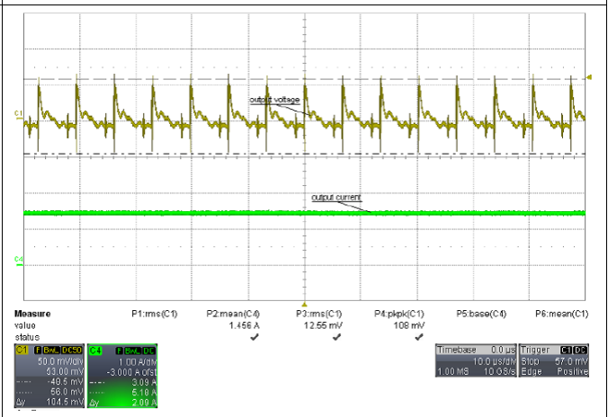
Figure 18. Output Ripple: 108 mVpp
