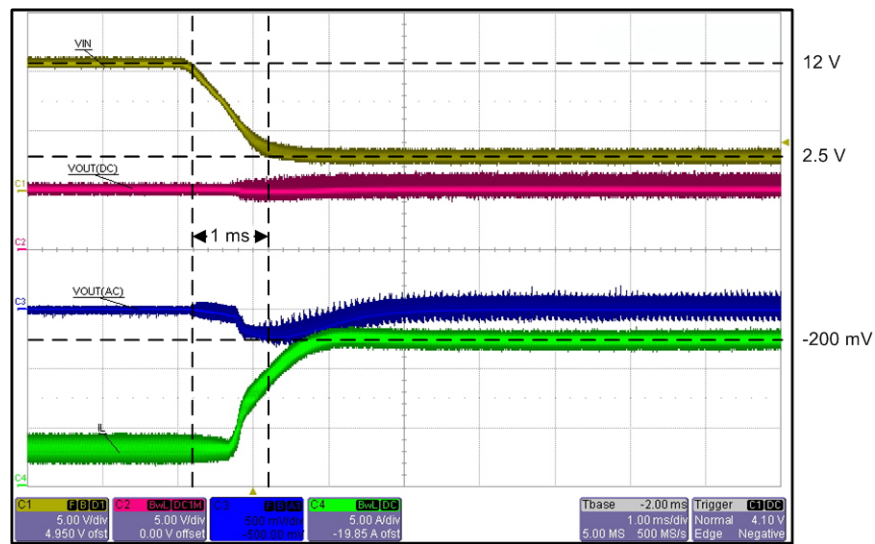
Figure 2. Cold Crank Waveform: ( \Delta V_{OUT\_MAX} = 200 \text{ mV} )
