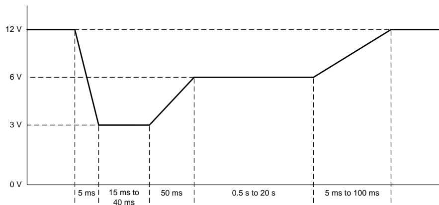
Figure 1. Example Cold-Crank Waveform
