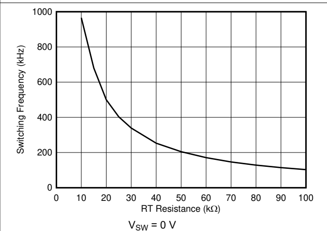
Figure 7-18. Oscillator Frequency vs RT Resistance V_{sw} = 0V
