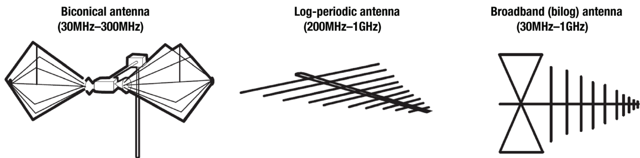
Figure 3. Measurement antennas referenced in the CISPR 25 specification.
