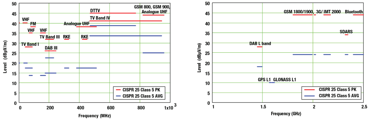
Figure 2. CISPR 25 Class 5 radiated limits for components/modules using the Absorber-Lined Shielded Enclosure (ALSE) test method with an antenna distance of 1m.
