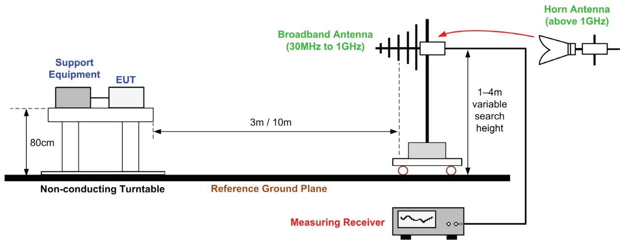
Figure 8. Radiated emissions measurement setup for FCC Part 15 and CISPR 22/32.
