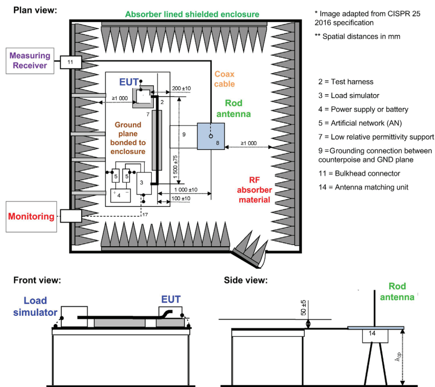
Figure 4. CISPR 25 radiated emissions measurement setup with active rod antenna (150kHz to 30MHz).
