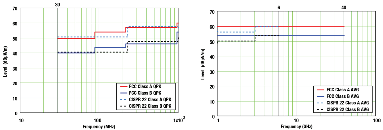
Figure 7. FCC Part 15 and CISPR 22/32 radiated limits for Class A and Class B using QPK and AVG detectors below and above 1GHz, respectively.
