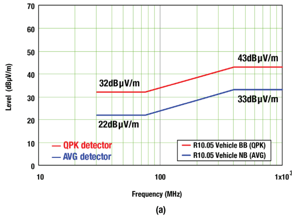
Figure 1. UNECE Regulation 10 radiated EMI limits for vehicles at 10m (a); and ESAs/components at 1m (b).
