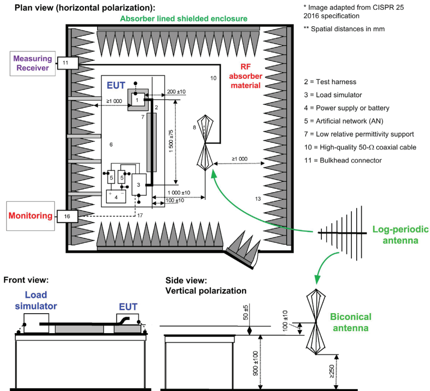
Figure 5. CISPR 25 radiated emissions measurement setup with biconical antenna (30MHz to 300MHz) or log-periodic antenna (200MHz to 1GHz).
