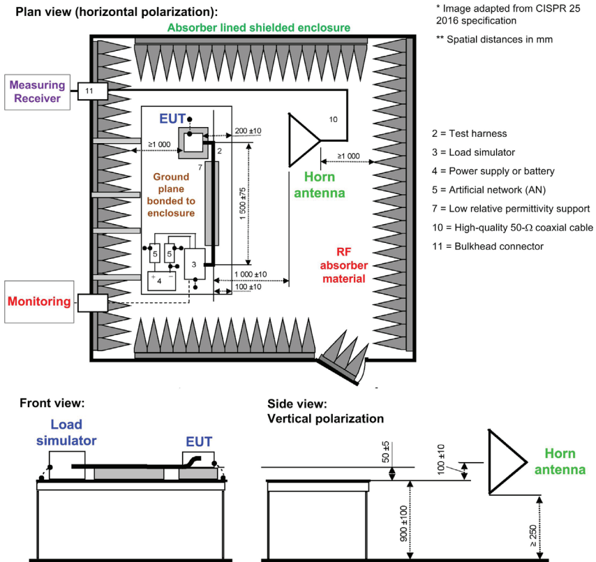
Figure 6. CISPR 25 radiated emissions measurement setup with horn antenna (above 1GHz).
