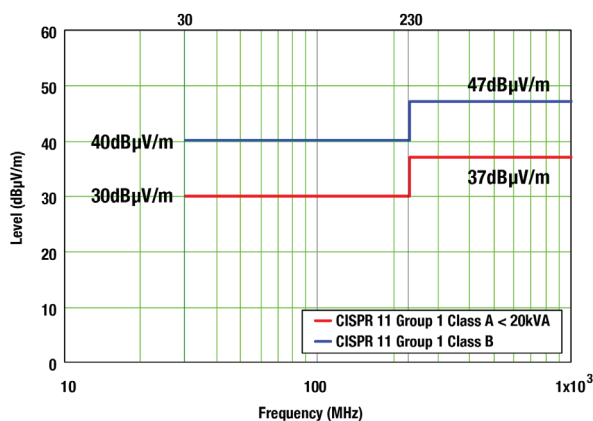
Figure 9. CISPR 11/EN 55011 Group 1 radiated emission limits, QPK detector, measured on a test site with 10m antenna distance.
