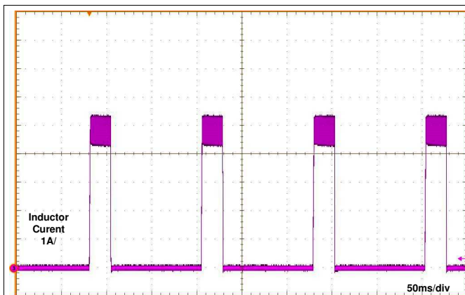
Figure 5. LM60440 Inductor Current Burst in Short-Circuit Mode
