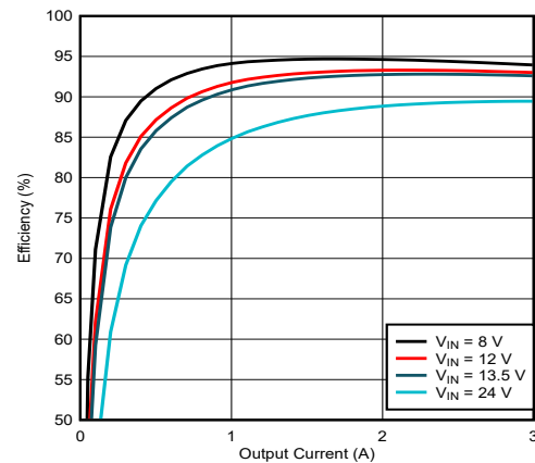
Figure 9-11. LM61430-Q1 Efficiency
