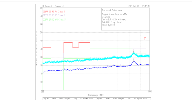
V_{OUT} = 5\text{ V} F_{SW} = 400\text{ kHz} I_{OUT} = 5\text{ A} Frequency tested: 300 MHz to 1 GHz Tested on 6-A variant with LM61460EVM
