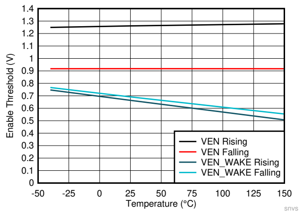
Figure 7-6. Enable Thresholds
