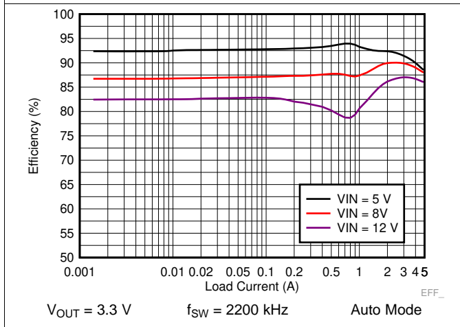
Figure 29. LM73605 Efficiency
