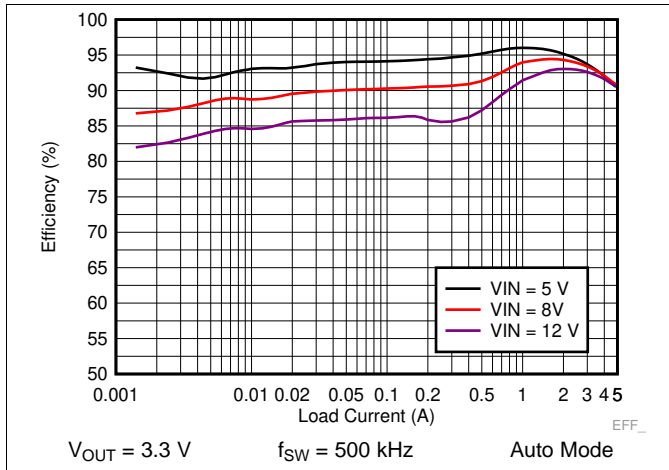
Figure 27. LM73605 Efficiency
