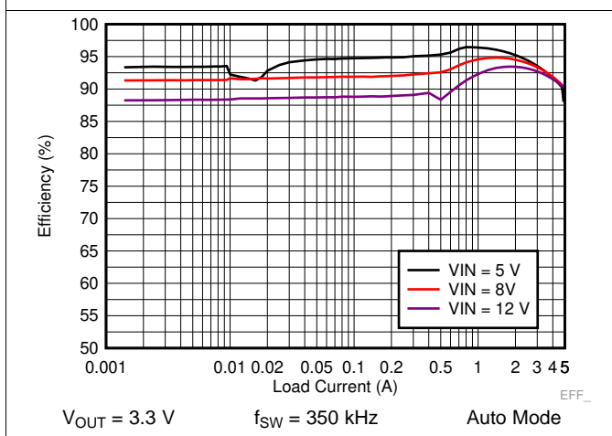
Figure 31. LM73605 Efficiency
