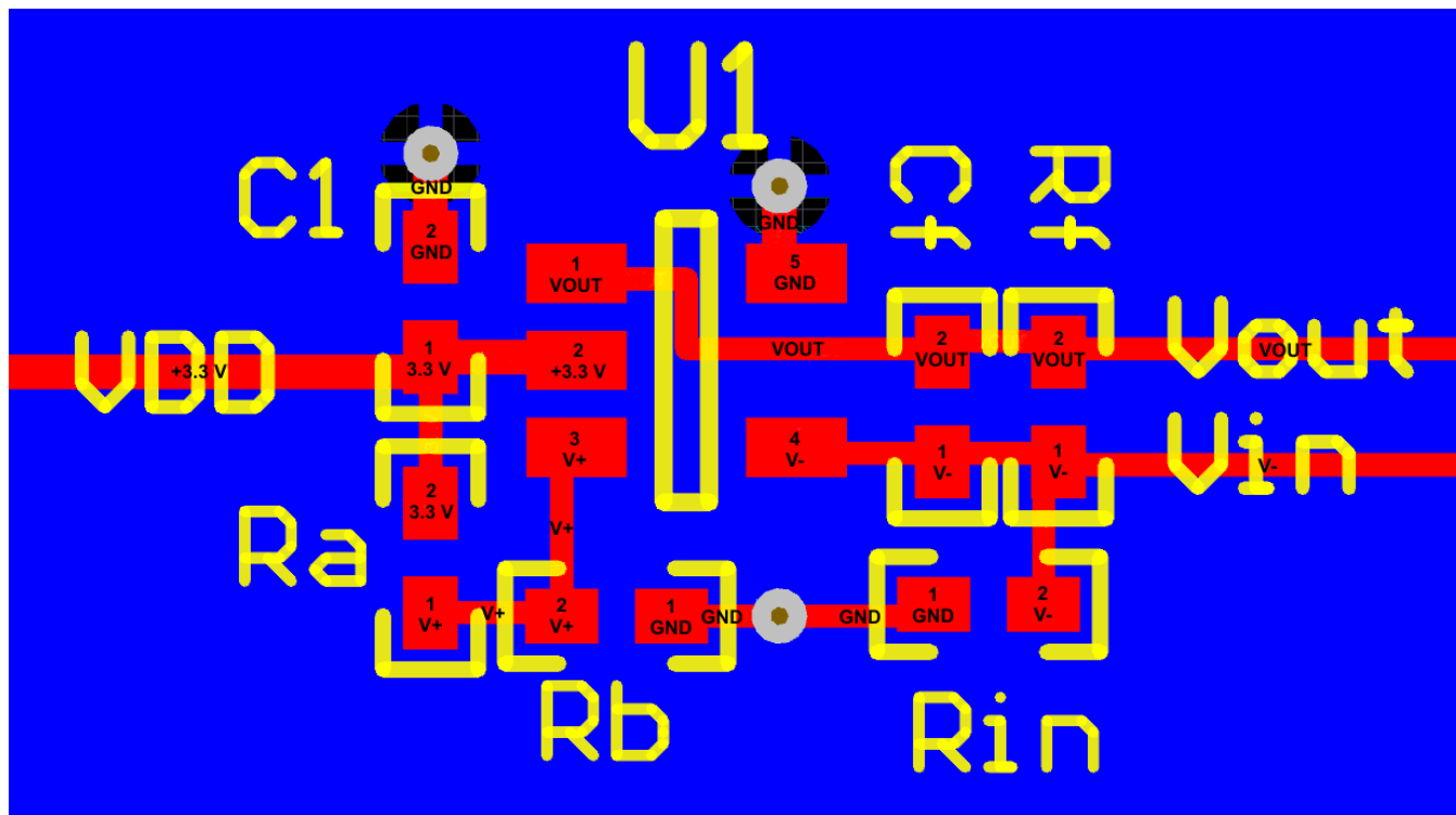
Figure 68. LMC7101 Example Layout
