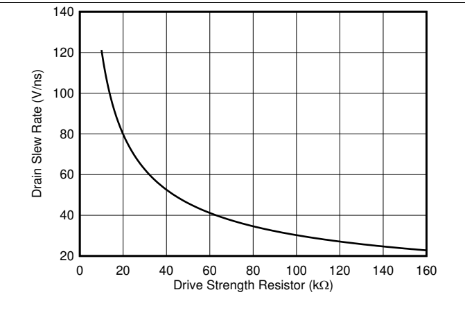
Figure 2. Drain Slew Rate vs Drive-Strength Resistor
