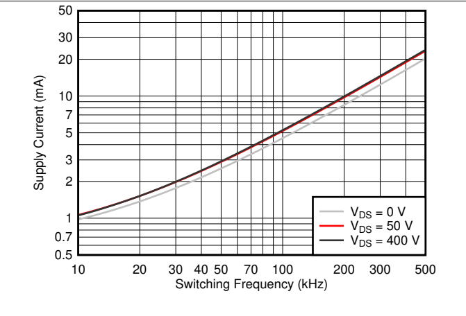
Figure 6. V DD Supply Current vs Switching Frequency
