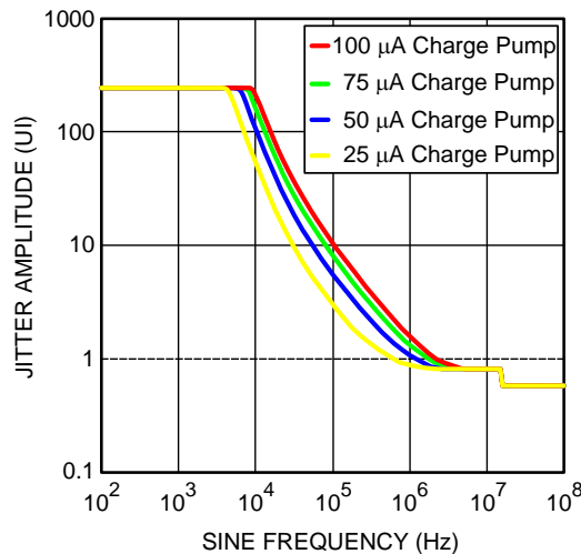
Figure 7. LMH0346 2.97 Gbps Jitter Tolerance with Different Charge Pump Current Settings
