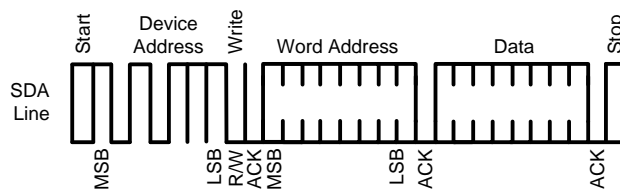
Figure 2. SMBus Register Write
