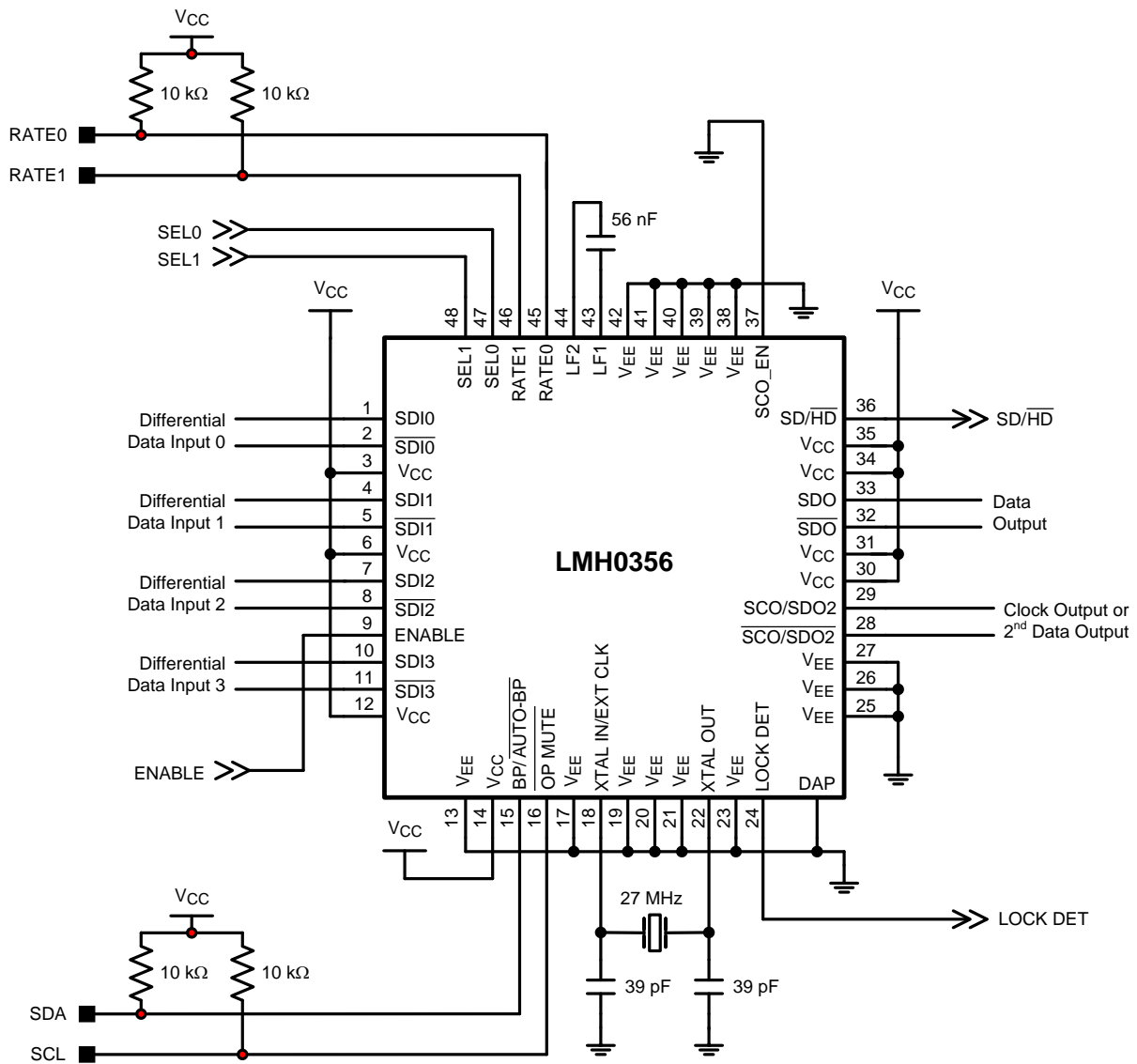
Figure 4. LMH0356 SMBus Implementation
