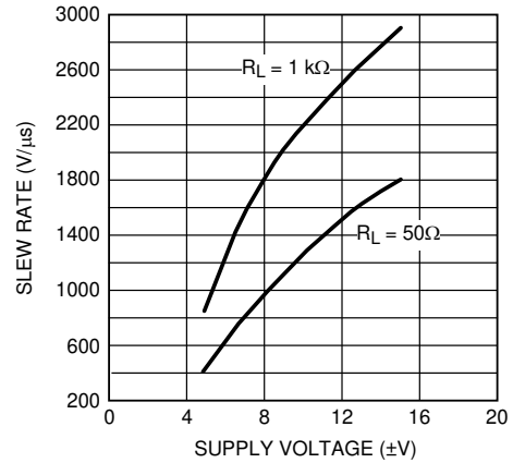
Figure 5-2. Slew Rate
