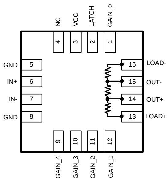
Figure 2. Internal Load Resistors
