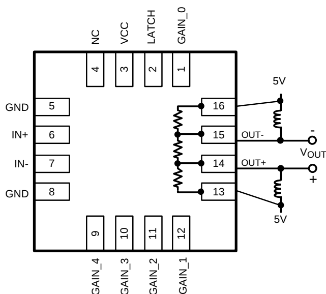
Figure 4. Using Low-Gain Mode (200Ω Load)
