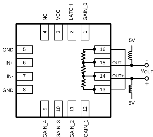
Figure 5. Alternate Connection for Low-Gain Mode (200Ω Load)
