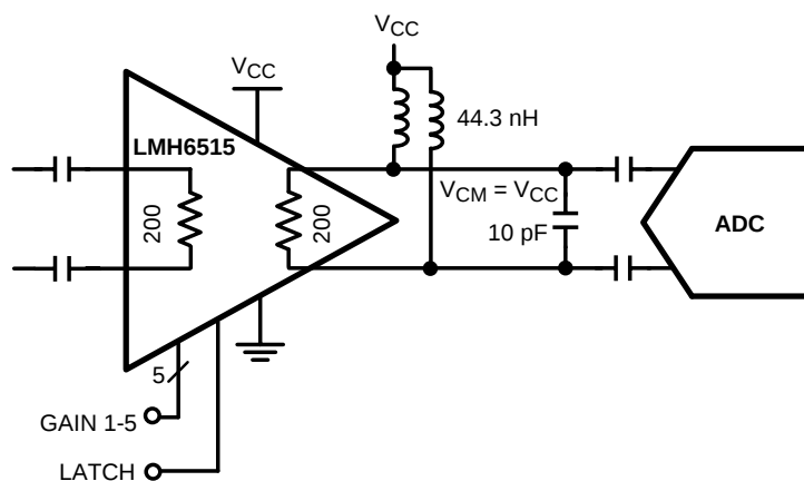
Figure 1. LMH6515 With Output Pull-Up Inductors
