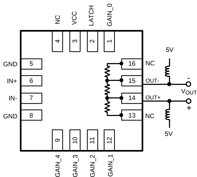
Figure 3. Using High-Gain Mode (400Ω Load)
