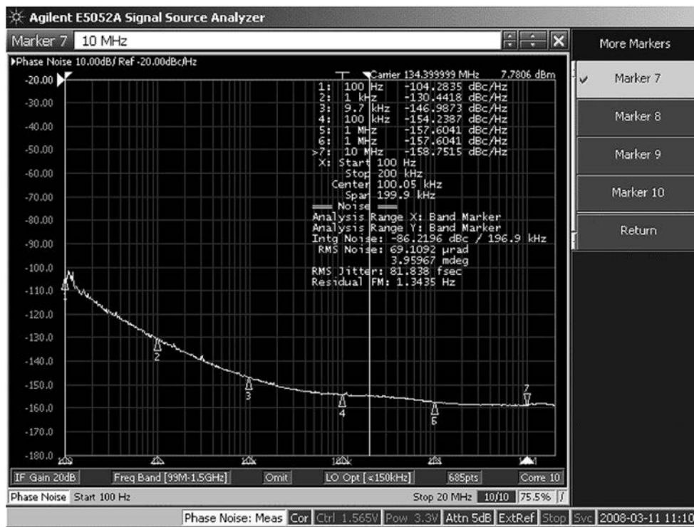
Figure 60. Vectron Model 5310 VCXO, 134.4 MHz, Open Loop Phase Noise
