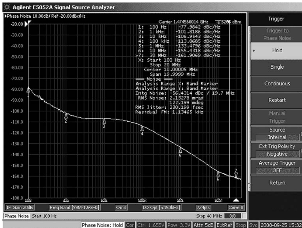
Figure 26. LMK04031 Fout Phase Noise, Epson Toyocom VG-4501 VCXO
