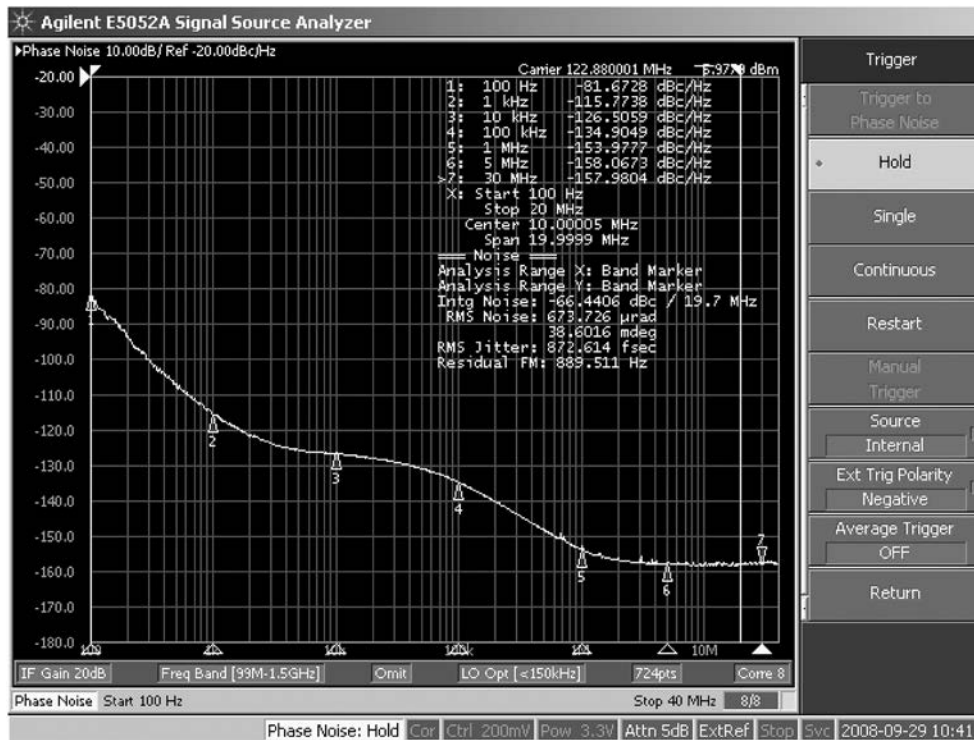
Figure 53. LMK04031 LVPECL Phase Noise, Suntsu SVD Series VCXO, 30.72 MHz
