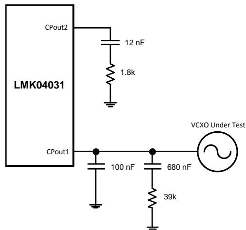
Figure 3. PLL1 and PLL2 Loop Filter Components
