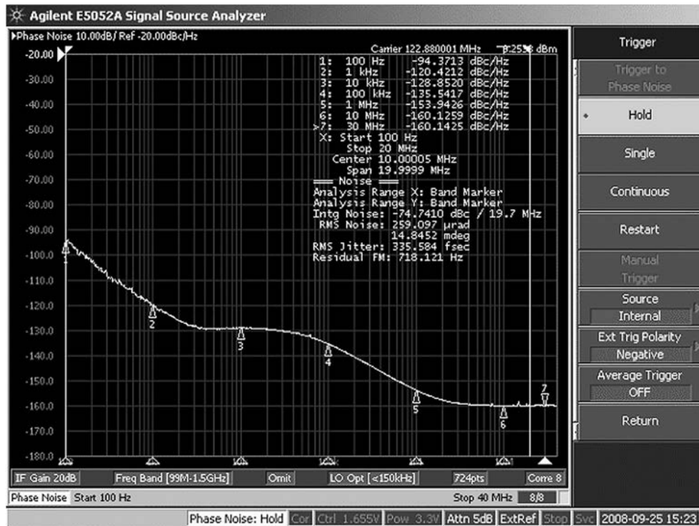
Figure 23. LMK04031 LVCMOS Phase Noise, Crystek CVPD-920-61.44 VCXO
