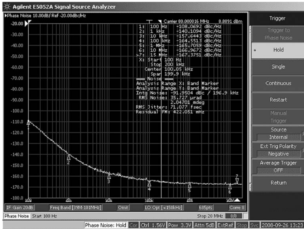
Figure 15. Crystek CVHD-950-80 VCXO Open Loop Phase Noise
