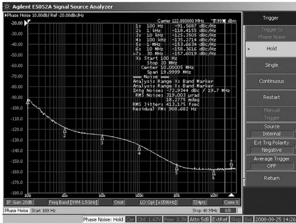
Figure 9. LMK04031 LVPECL Phase Noise, CTS model 357 VCXO
