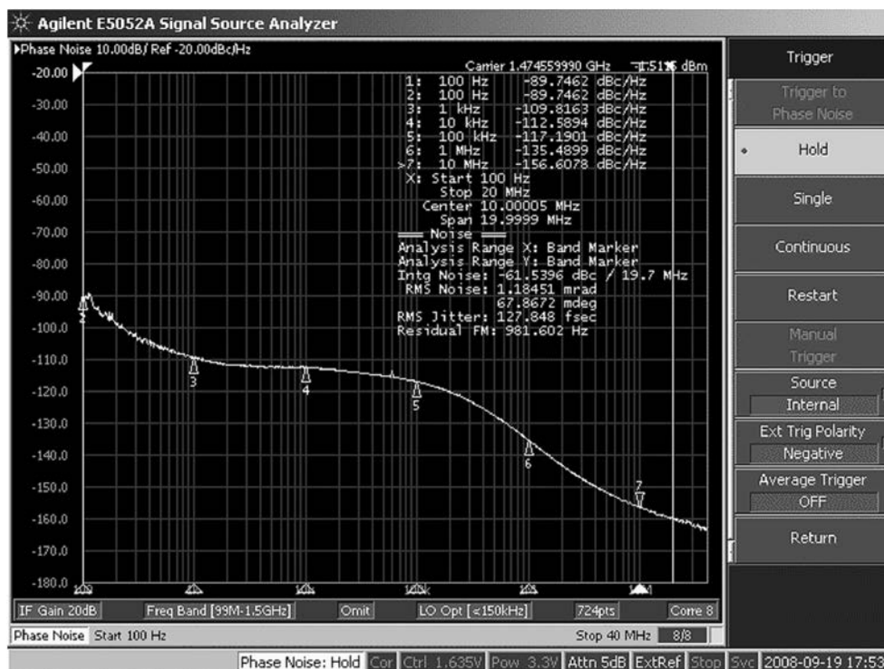
Figure 11. LMK04031 Fout Phase Noise, Crystek CVHD-950-122.88 VCXO
