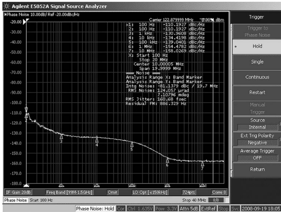
Figure 12. LMK04031 LVDS Phase Noise, Crystek CVHD-950-122.88 VCXO
