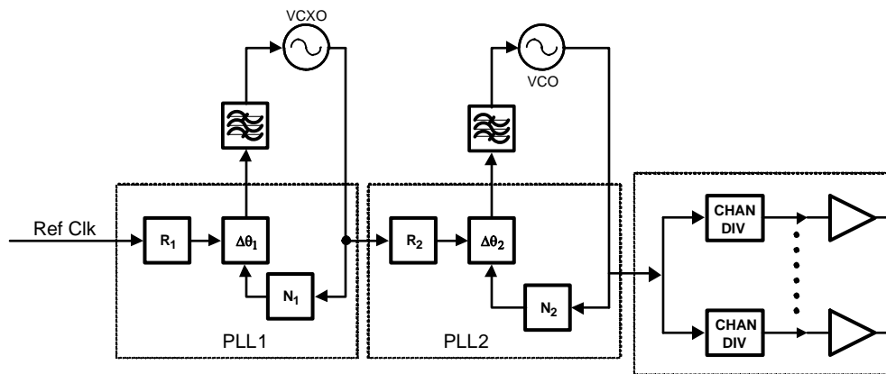
Figure 1. Dual-PLL Jitter Cleaning Clock Synthesizer Architecture
