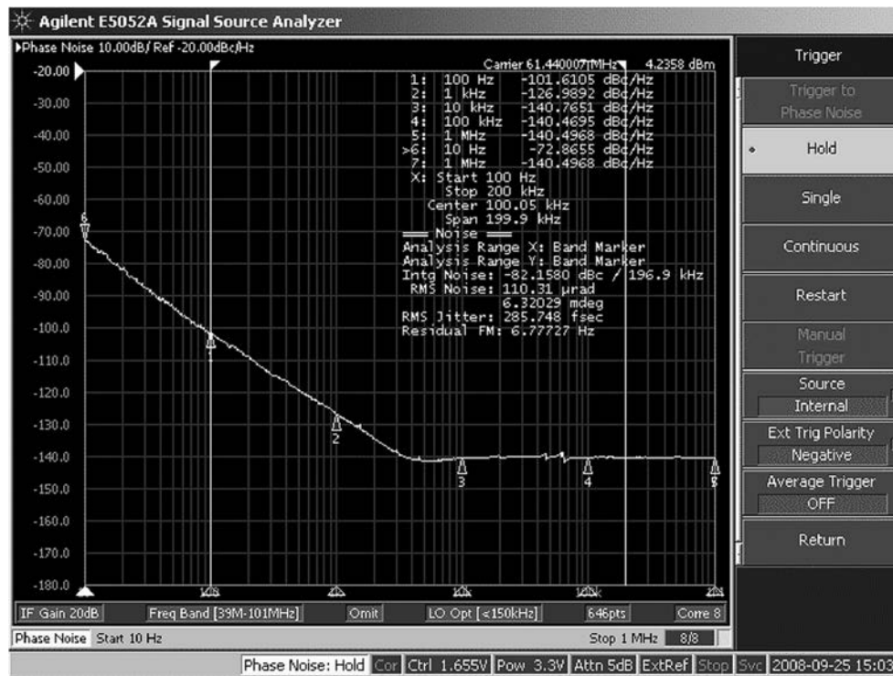
Figure 20. Crystek CVPD-920-61.44 VCXO Open Loop Phase Noise
