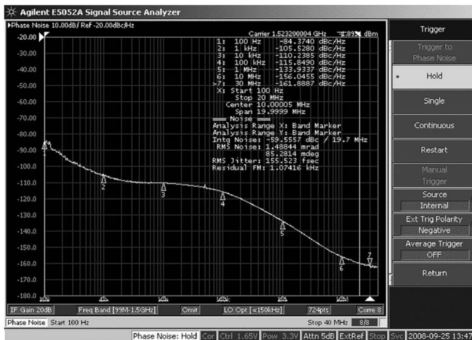
Figure 61. LMK04031 Fout Phase Noise, Vectron Model 5310 VCXO, 134.4 MHz
