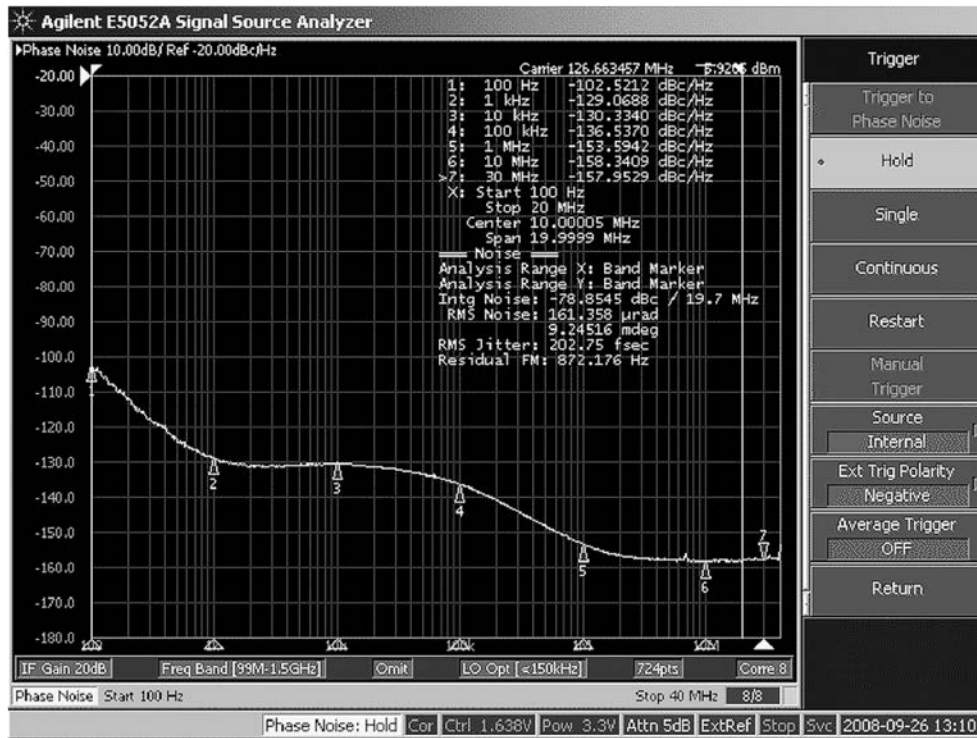
Figure 19. LMK04031 LVPECL Phase Noise, Crystek CVHD-950-80 VCXO
