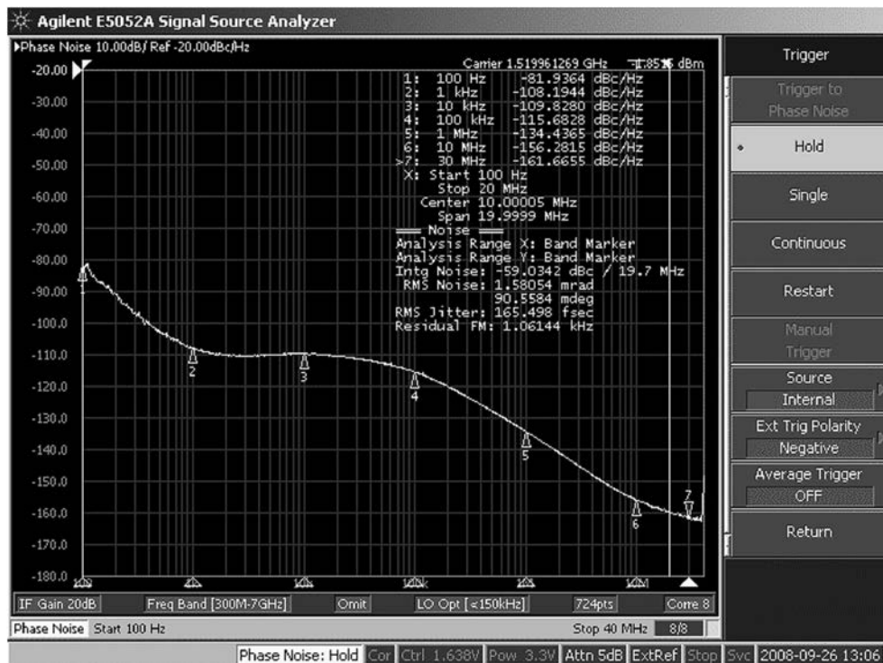
Figure 16. LMK04031 Fout Phase Noise, Crystek CVHD-950-80 VCXO
