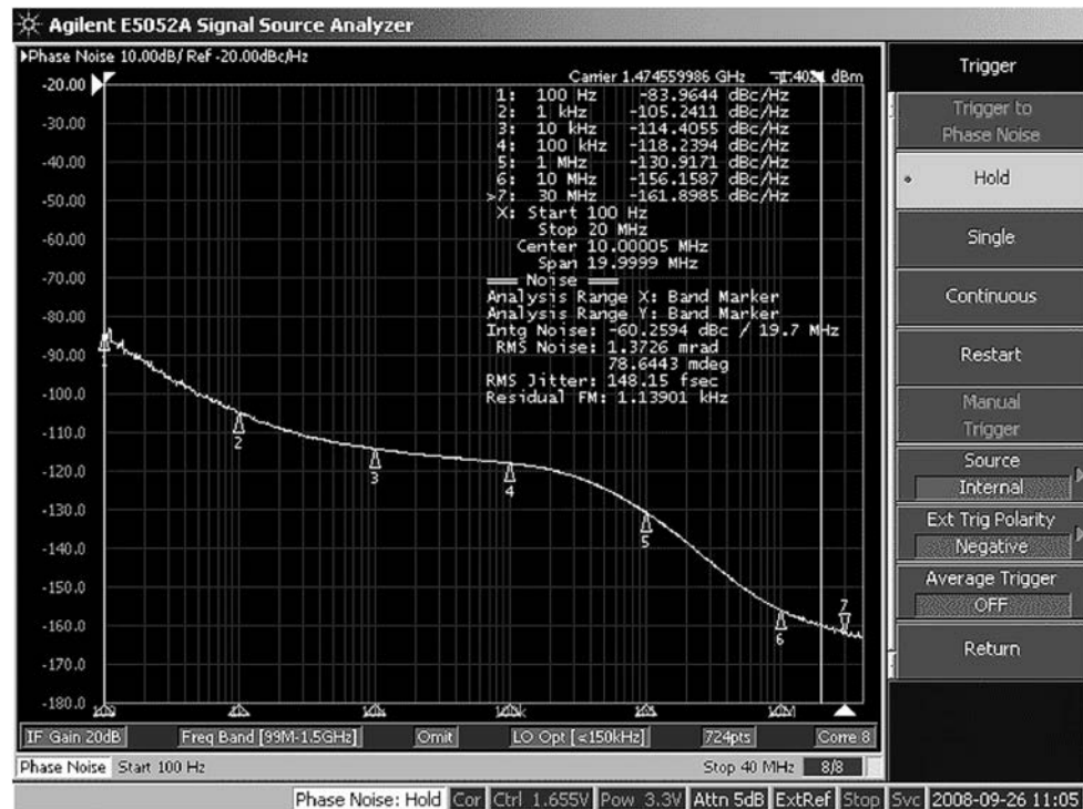
Figure 36. LMK04031 Fout Phase Noise, Epson Toyocom TCO-2111-AA VCXO
