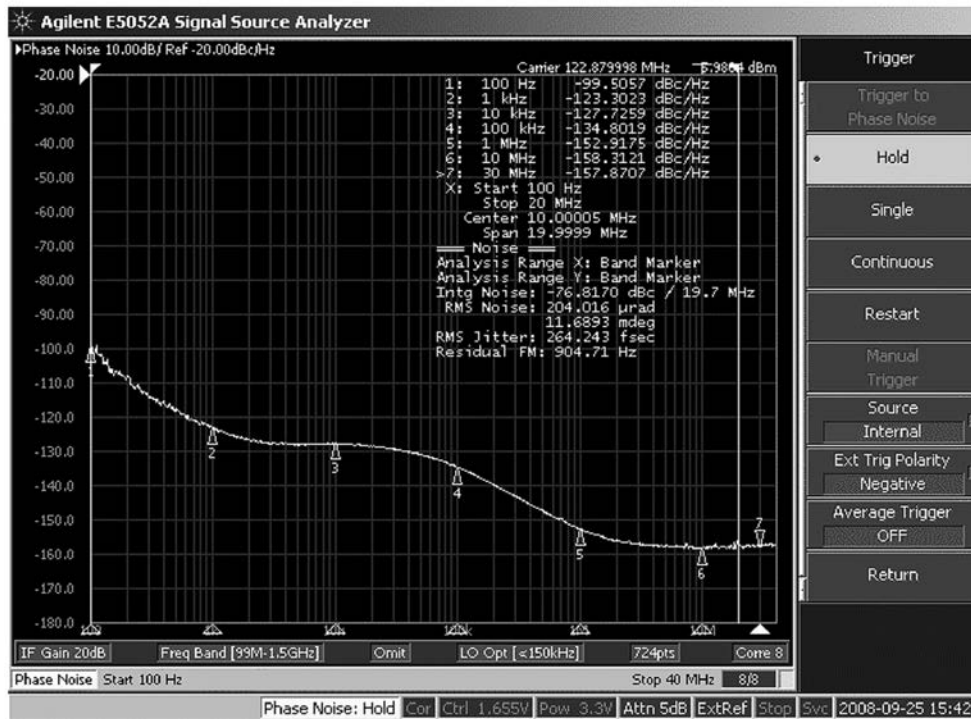
Figure 29. LMK04031 LVPECL Phase Noise, Epson Toyocom VG-4501 VCXO
