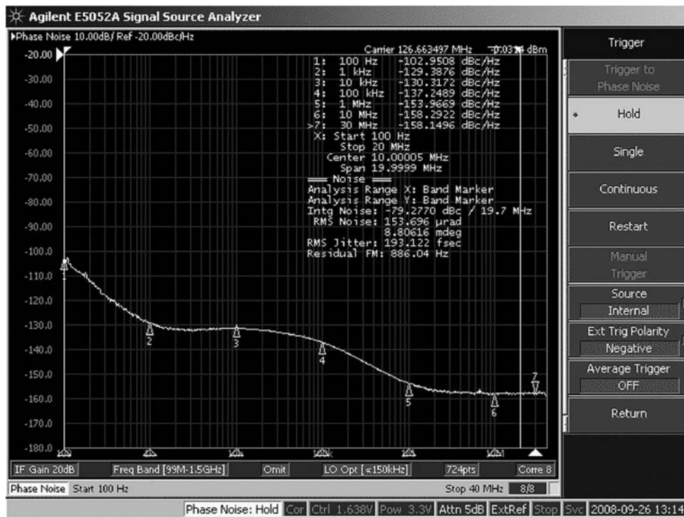
Figure 17. LMK04031 LVDS Phase Noise, Crystek CVHD-950-80 VCXO
