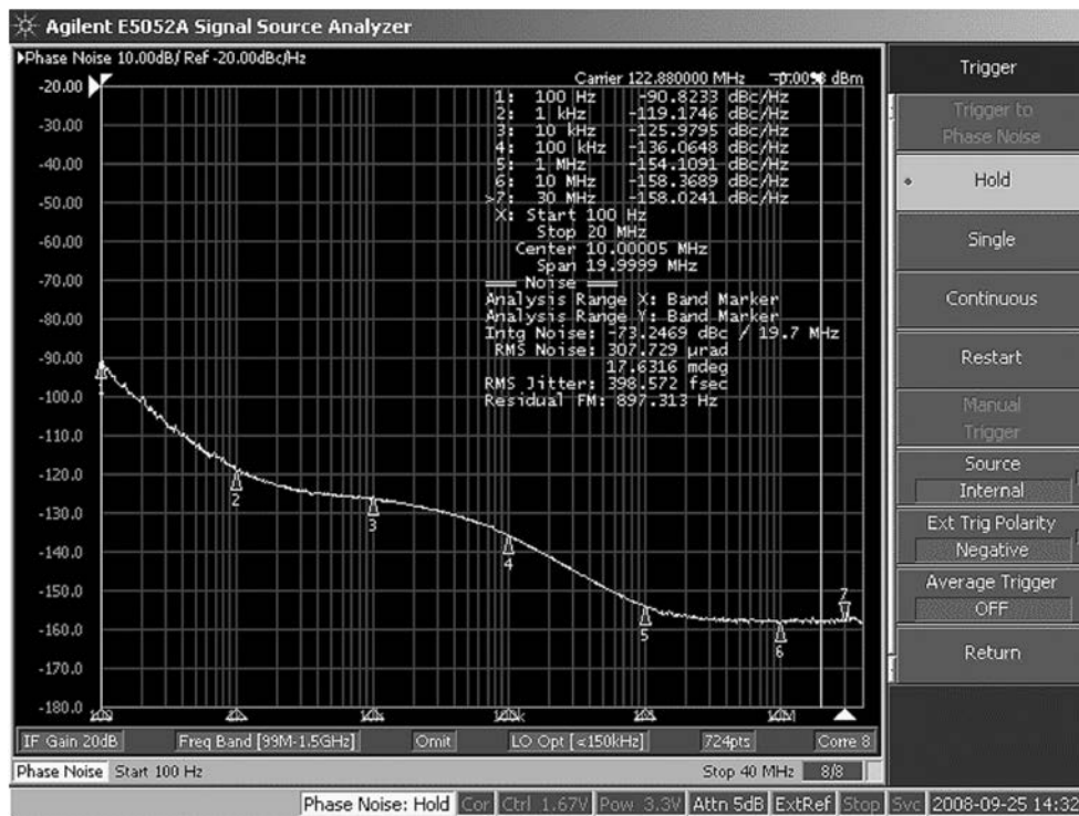
Figure 7. LMK04031 LVDS Phase Noise, CTS model 357 VCXO
