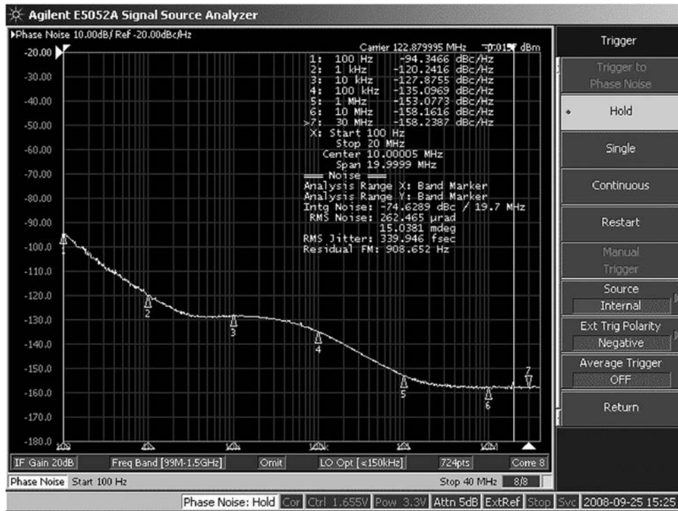
Figure 22. LMK04031 LVDS Phase Noise, Crystek CVPD-920-61.44 VCXO
