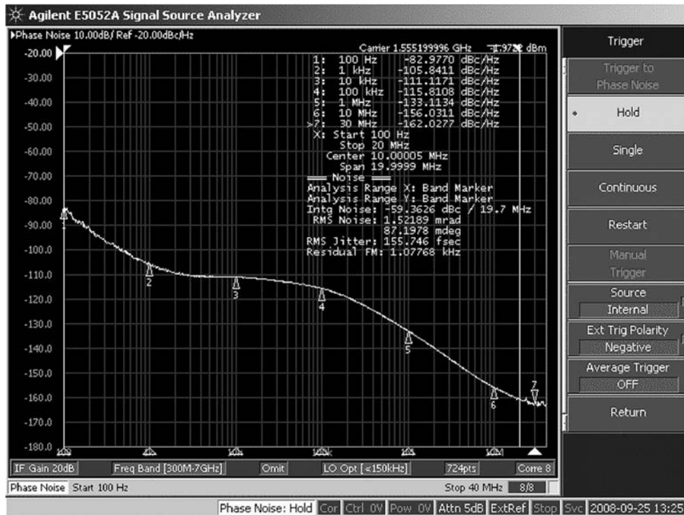
Figure 56. LMK04031 Fout Phase Noise, Vectron Model 5310 VCXO, 155.52 MHz
