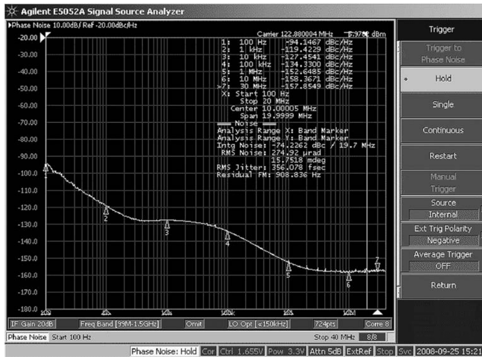
Figure 24. LMK04031 LVPECL Phase Noise, Crystek CVPD-920-61.44 VCXO
