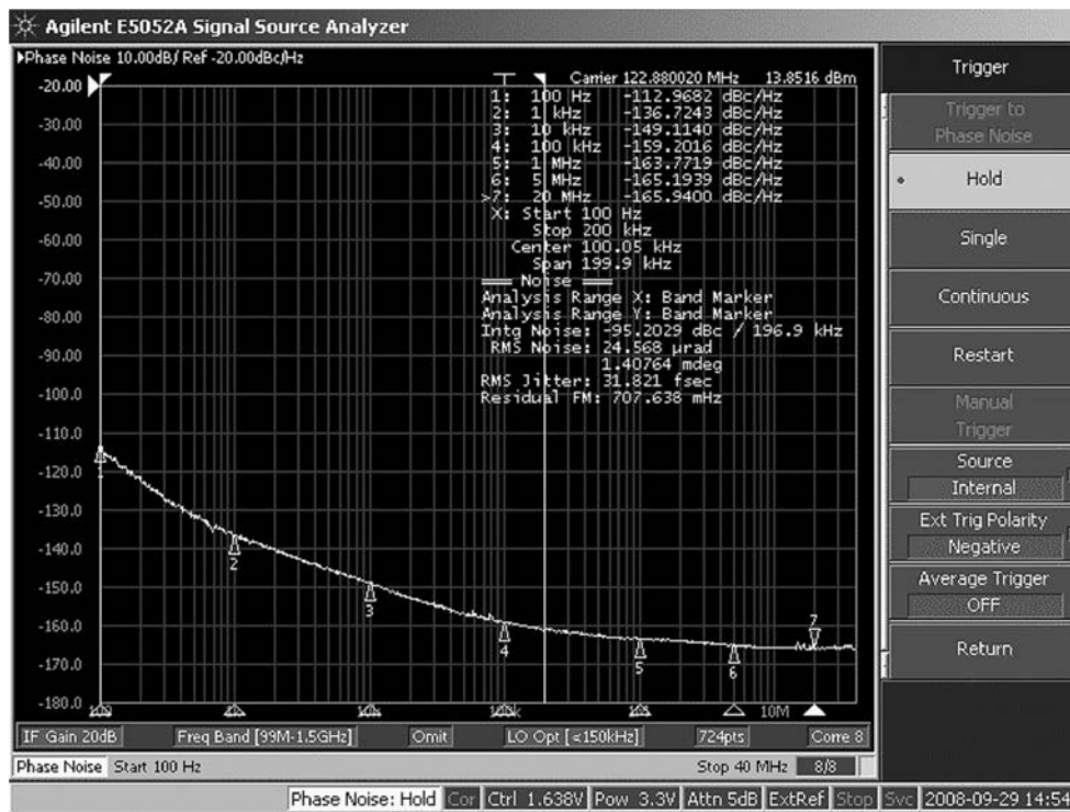
Figure 10. Crystek CVHD-950-122.88 VCXO Open Loop Phase Noise
