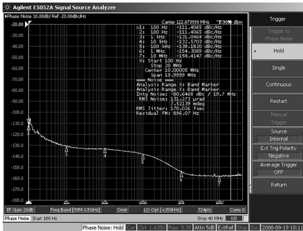
Figure 14. LMK04031 LVPECL Phase Noise, Crystek CVHD-950-122.88 VCXO
