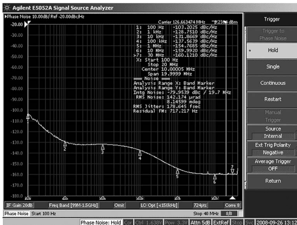
Figure 18. LMK04031 LVCMOS Phase Noise, Crystek CVHD-950-80 VCXO
