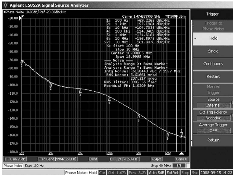
Figure 6. LMK04031 Fout Phase Noise, CTS model 357 VCXO
