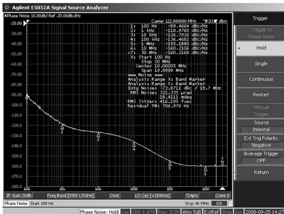
Figure 8. LMK04031 LVC MOS Phase Noise, CTS model 357 VCXO
