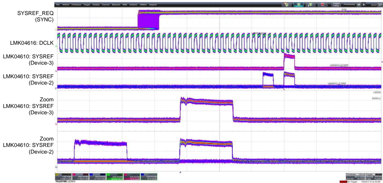
Figure 32. Configuration 5 Measurement
