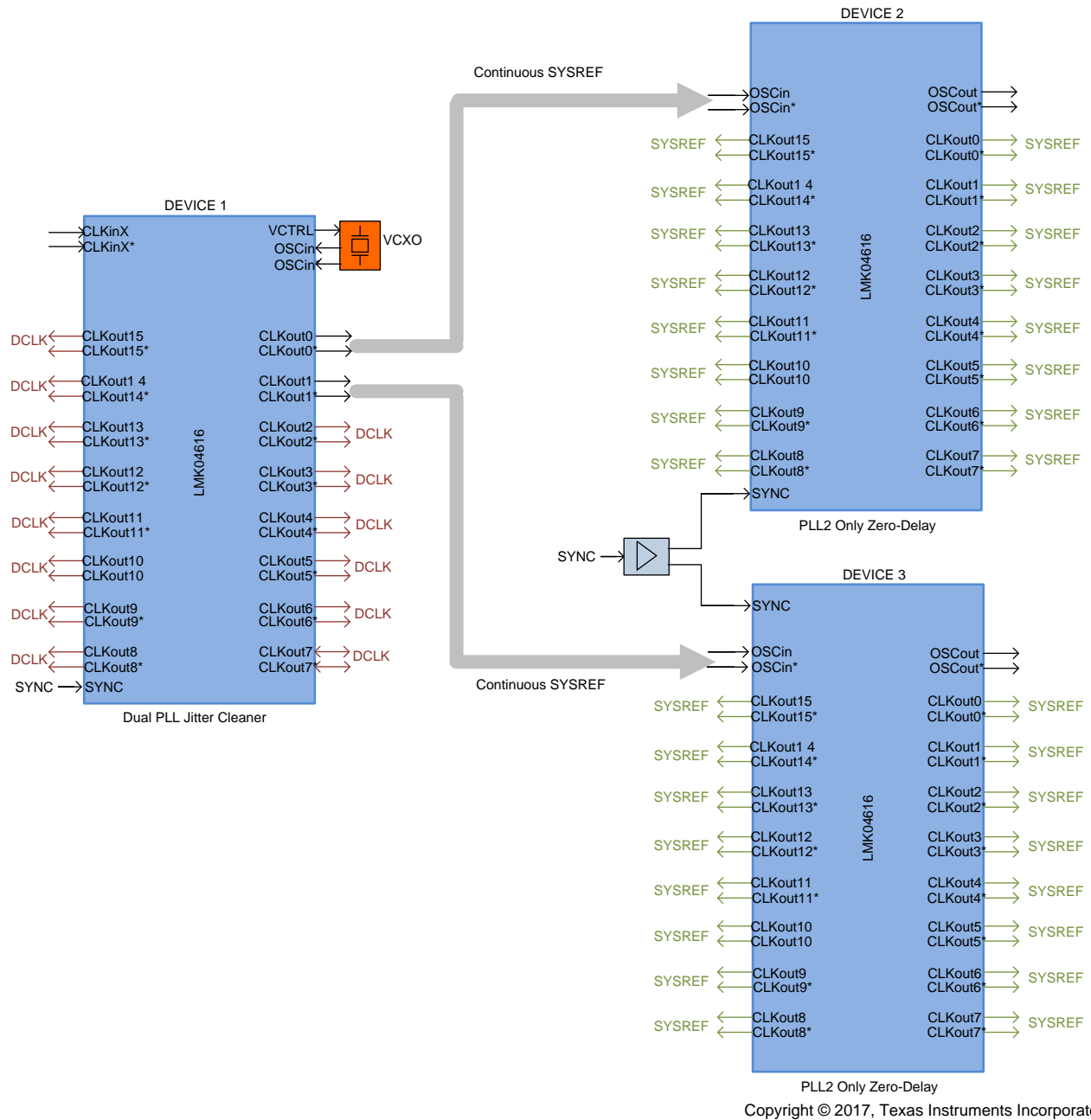
Figure 25. LMK0461x Device Configuration 5
