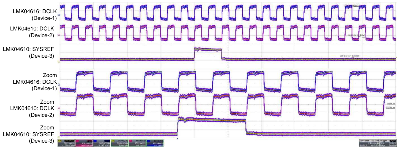
Figure 29. Configuration 2 Measurement
