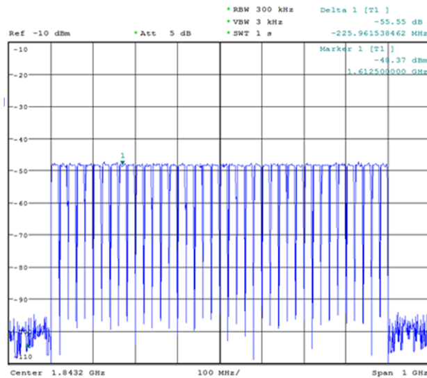
Figure 3. 800MHz of IBW at 1.8432GHz captured from Spectrum Analyzer
