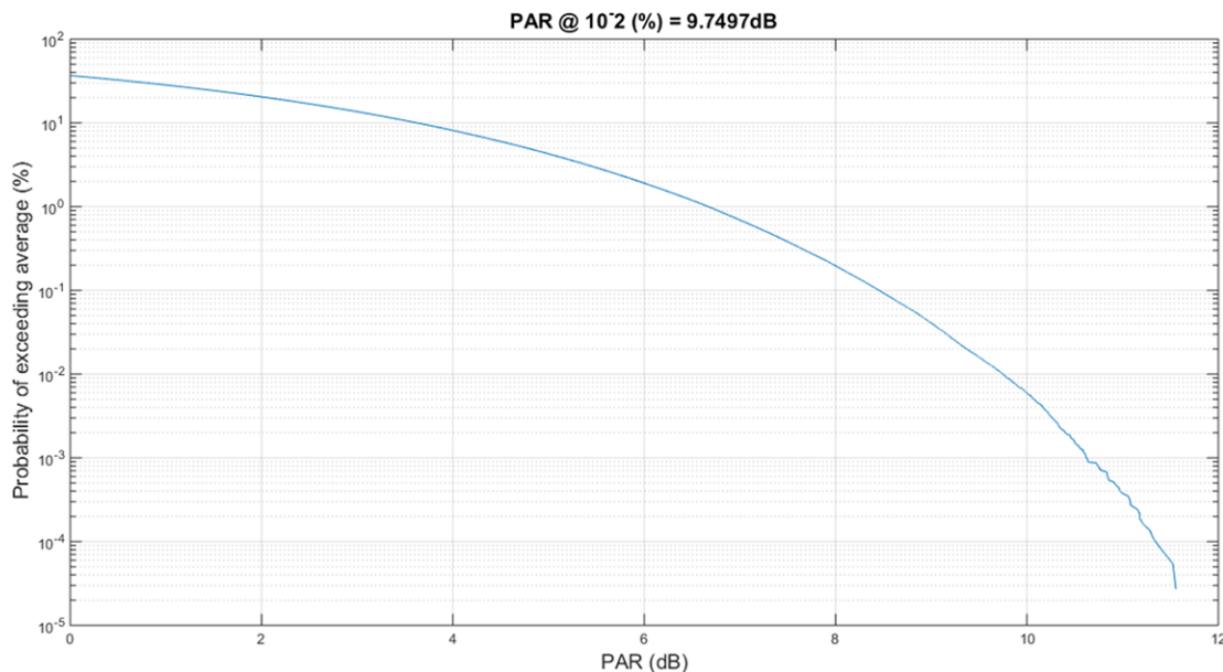
Figure 1. 9.75dB of PAR at 0.01% from CCDF Curve
