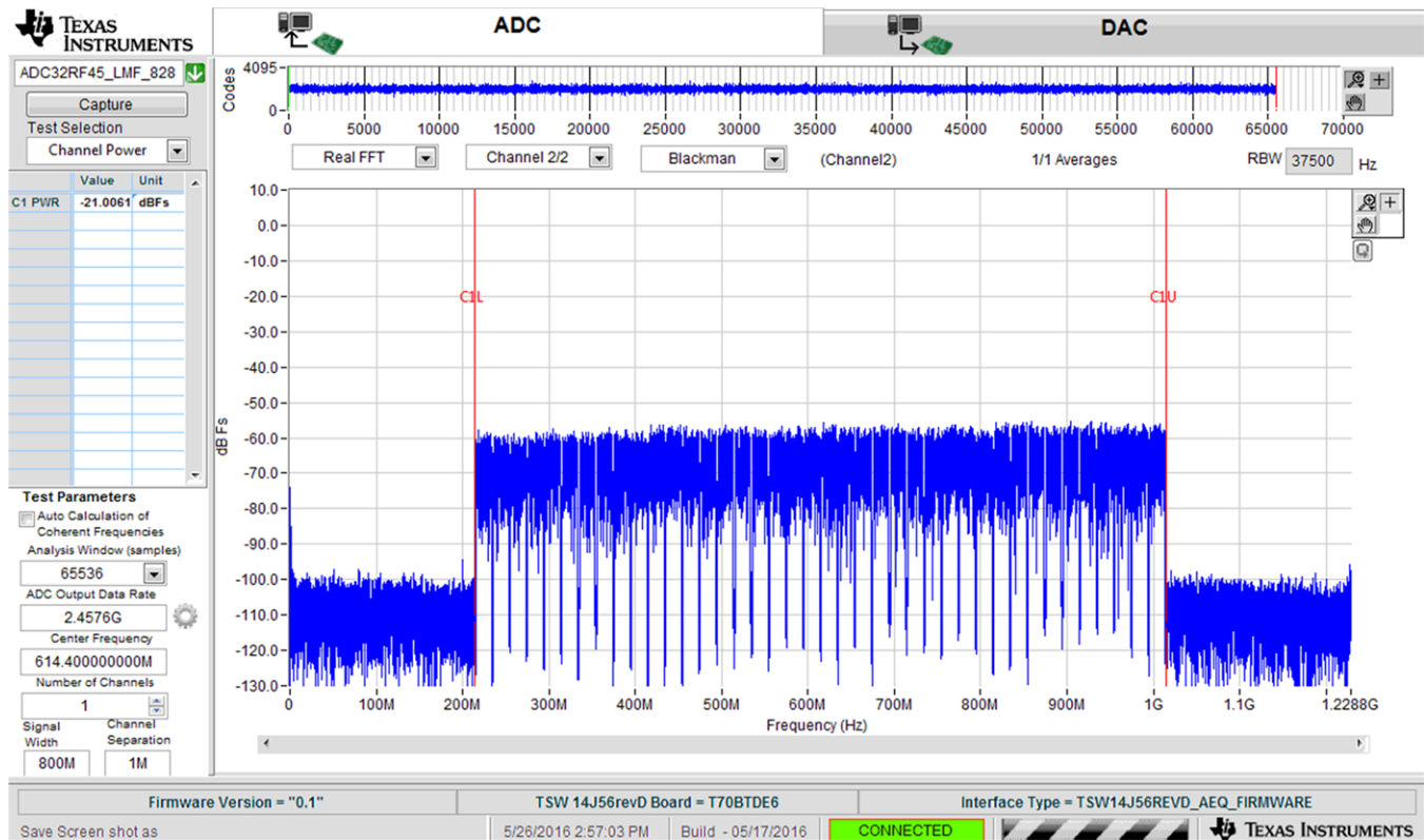
Figure 5. 800MHz of IBW captured from HSDC Pro
