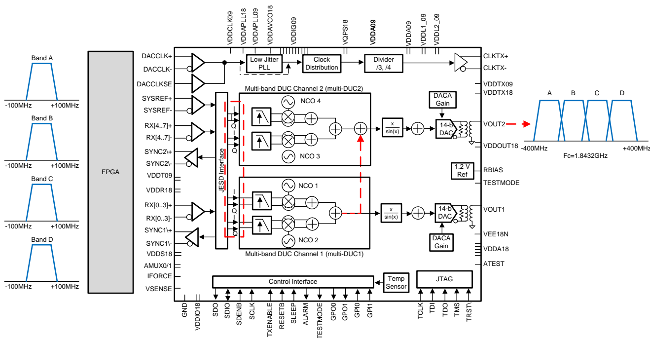
Figure 2. Block Diagram of DAC38RF8xEVM Operation
