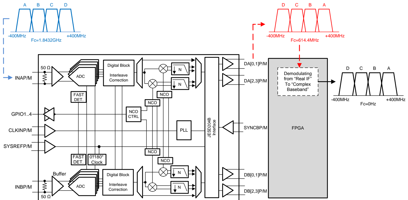
Figure 6. Example of Commercial Application Diagram
