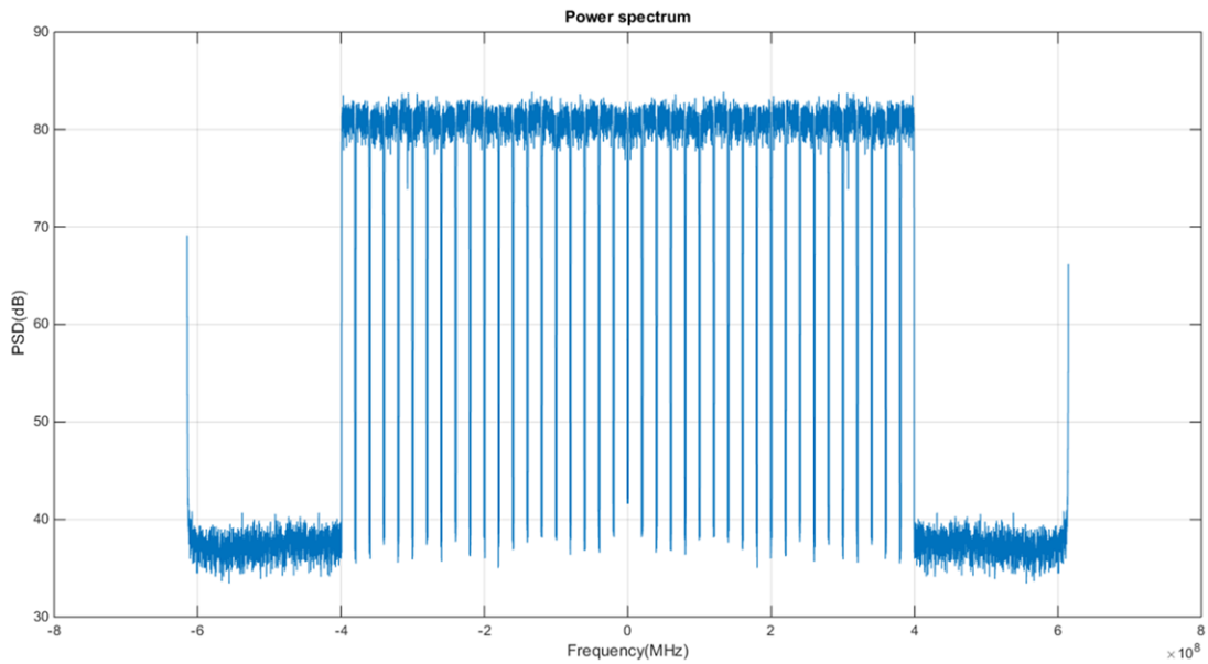
Figure 7. Demodulated 800MHz Pattern with Real-to-Complex from MATLAB
