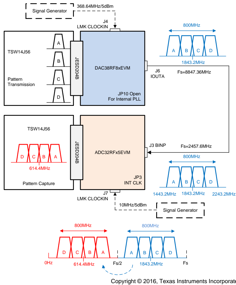
Figure 4. Hardware Setup for ADC32RFx5EVM
