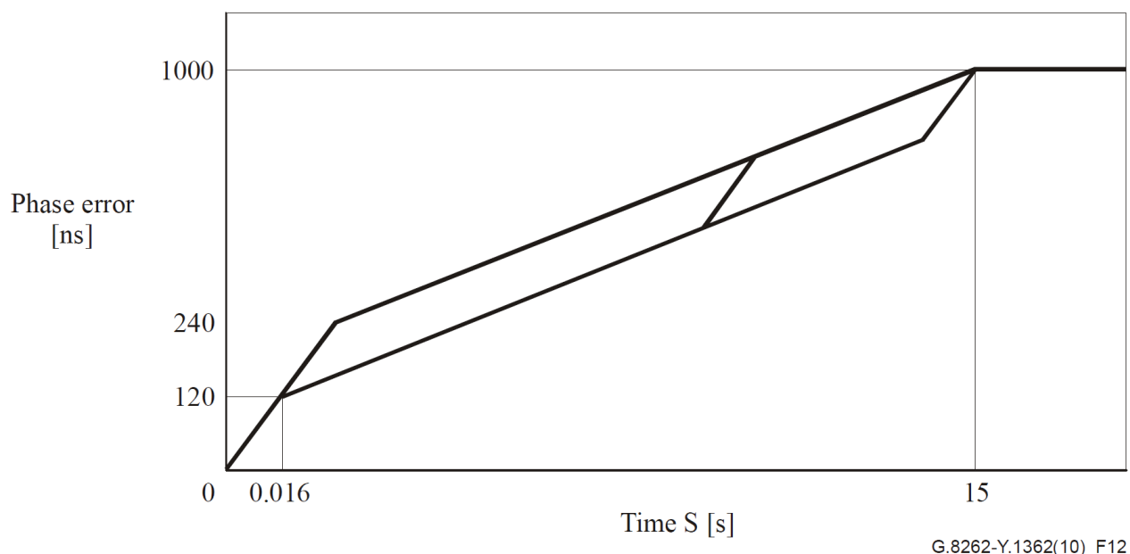
Figure 24. Maximum Phase Transient at the Output Due to Reference Switching for EEC-Option 1
