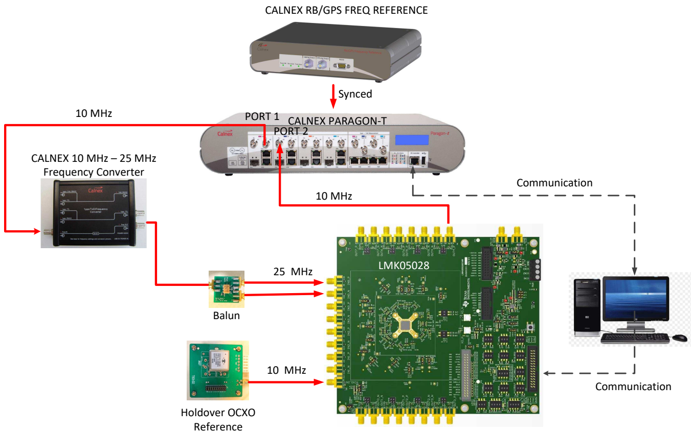
Figure 1. Test Setup for Wander Generation
