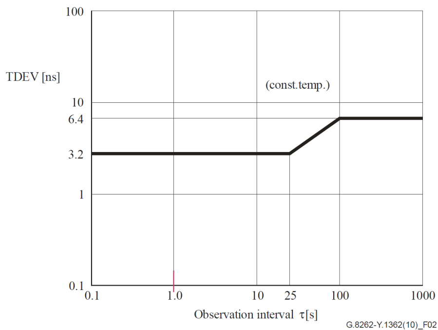
Figure 5. Wander Generation (TDEV) for EEC-Option 1 With Constant Temperature
