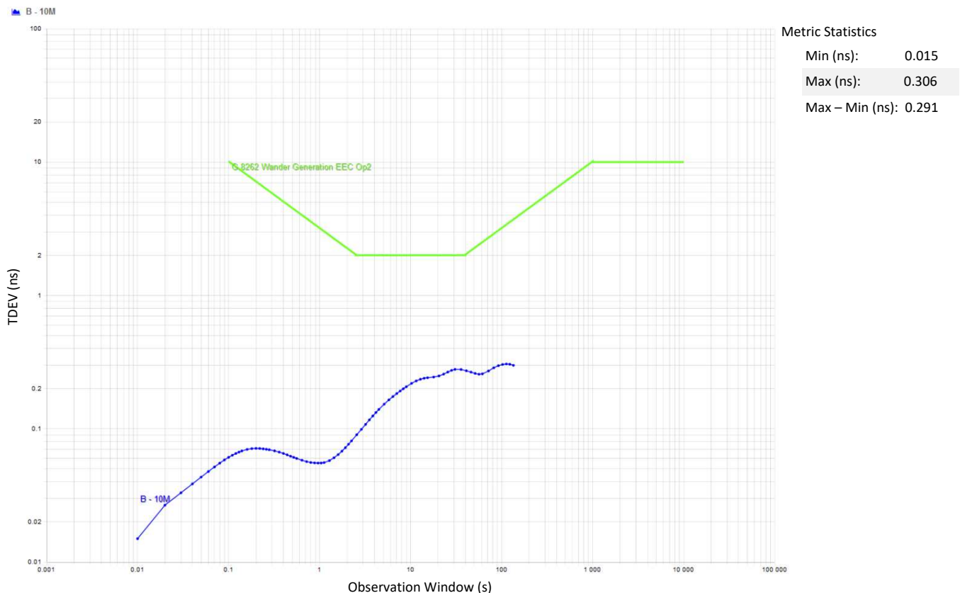
Figure 10. Wander Generation TDEV G.8262 EEC Option 2 Results, Tested at Constant Room Temperature With DPLL Bandwidth of 0.1 Hz
