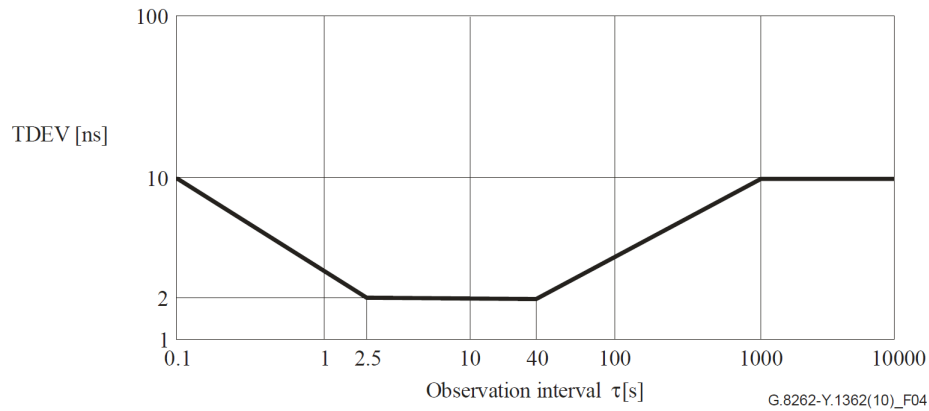
Figure 9. Wander Generation (TDEV) for EEC-Option 2 With Constant Temperature
