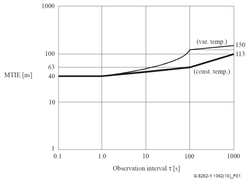
Figure 2. Wander Generation (MTIE) for EEC-Option 1
