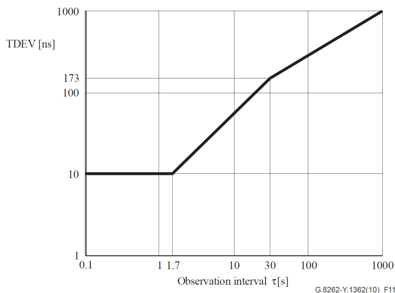
Figure 15. Wander Transfer for EEC-Option 2 (Maximum Output Wander When Input Wander Meets Figure 14)
