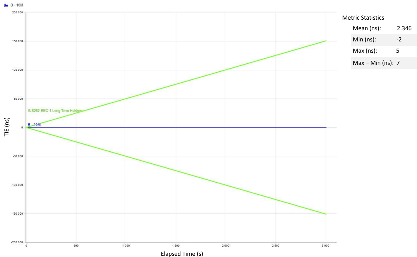
Figure 34. Holdover Option 1 Result
