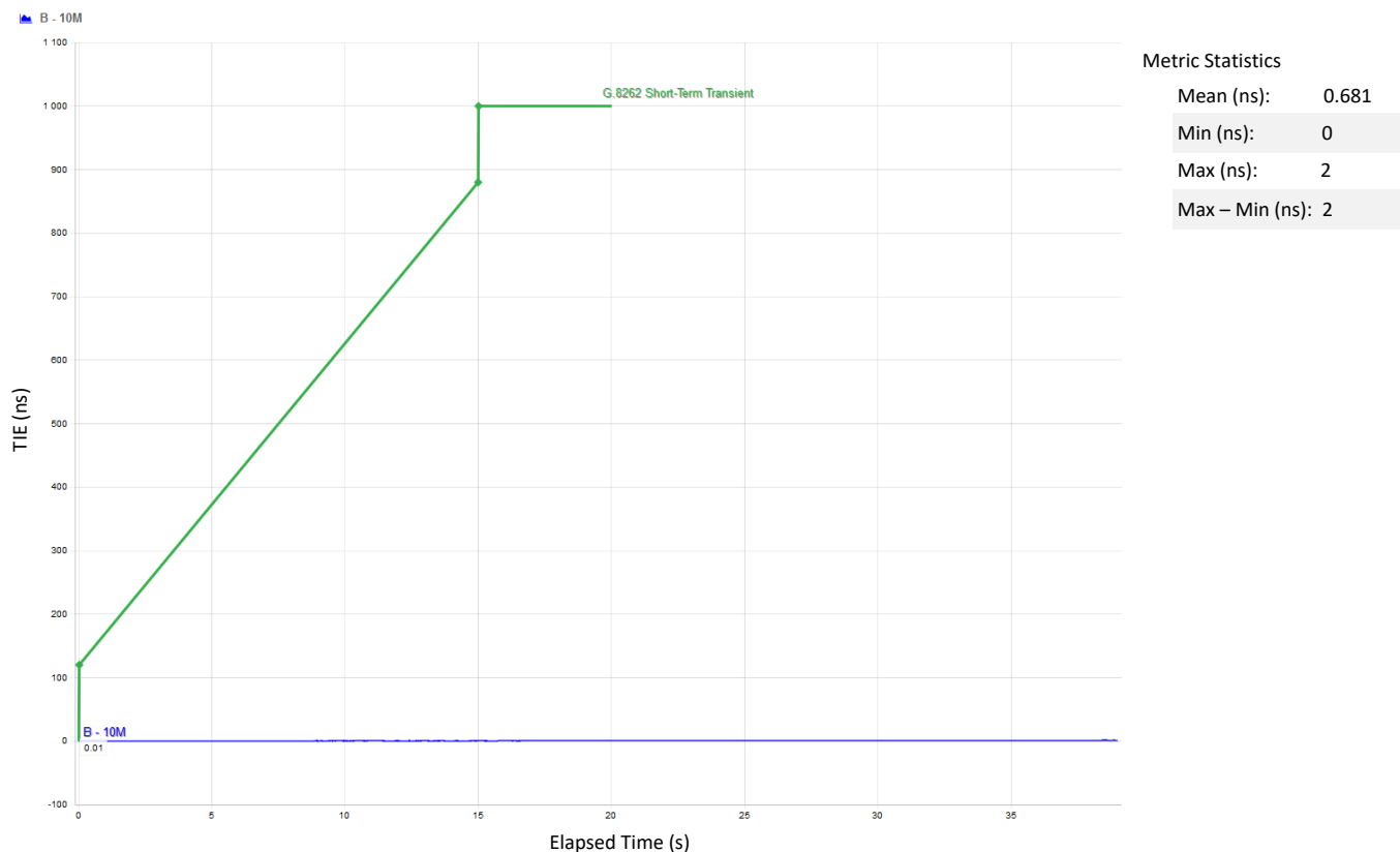
Figure 29. Phase Transient With Signal Interruptions Results
