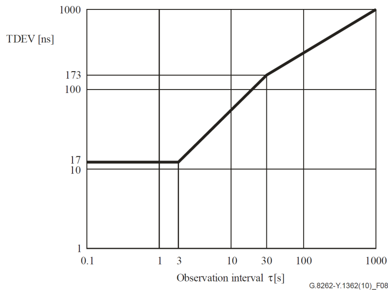
Figure 19. Input Wander Tolerance (TDEV) for EEC-Option 2
