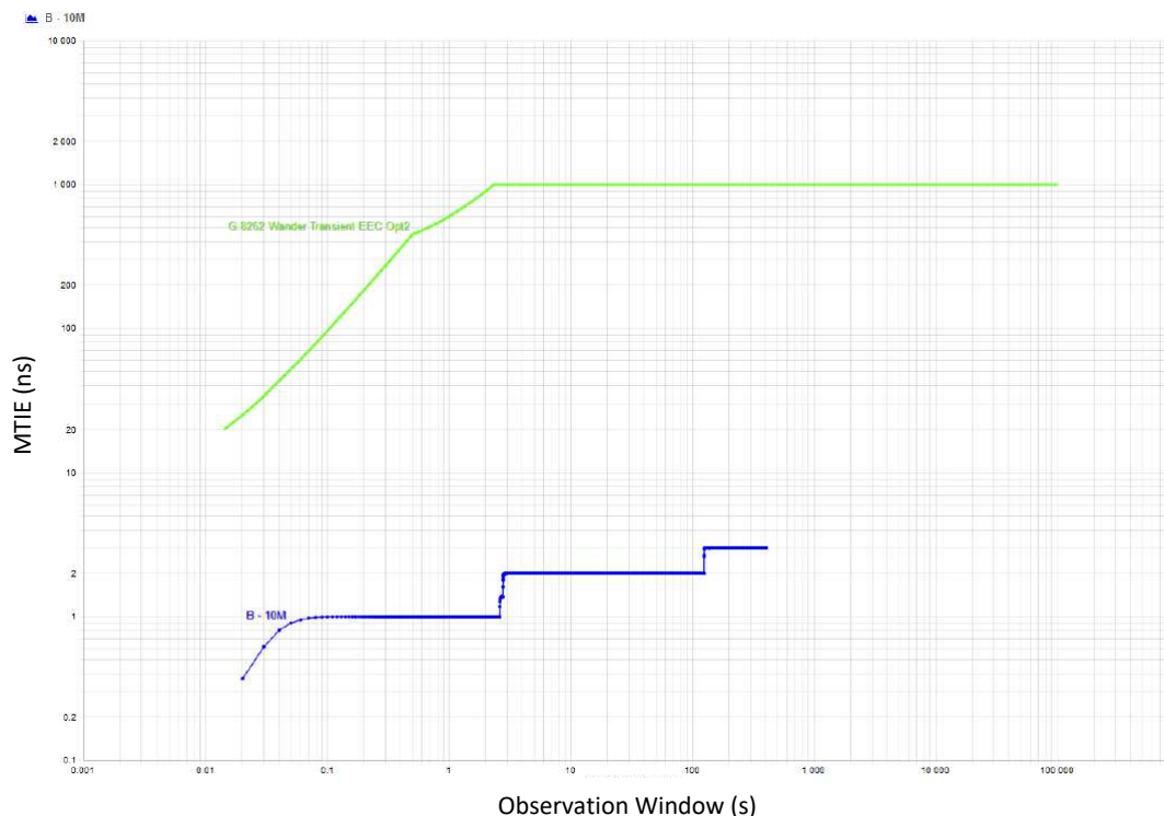
Figure 27. Short-Term Phase Transient Option 2
