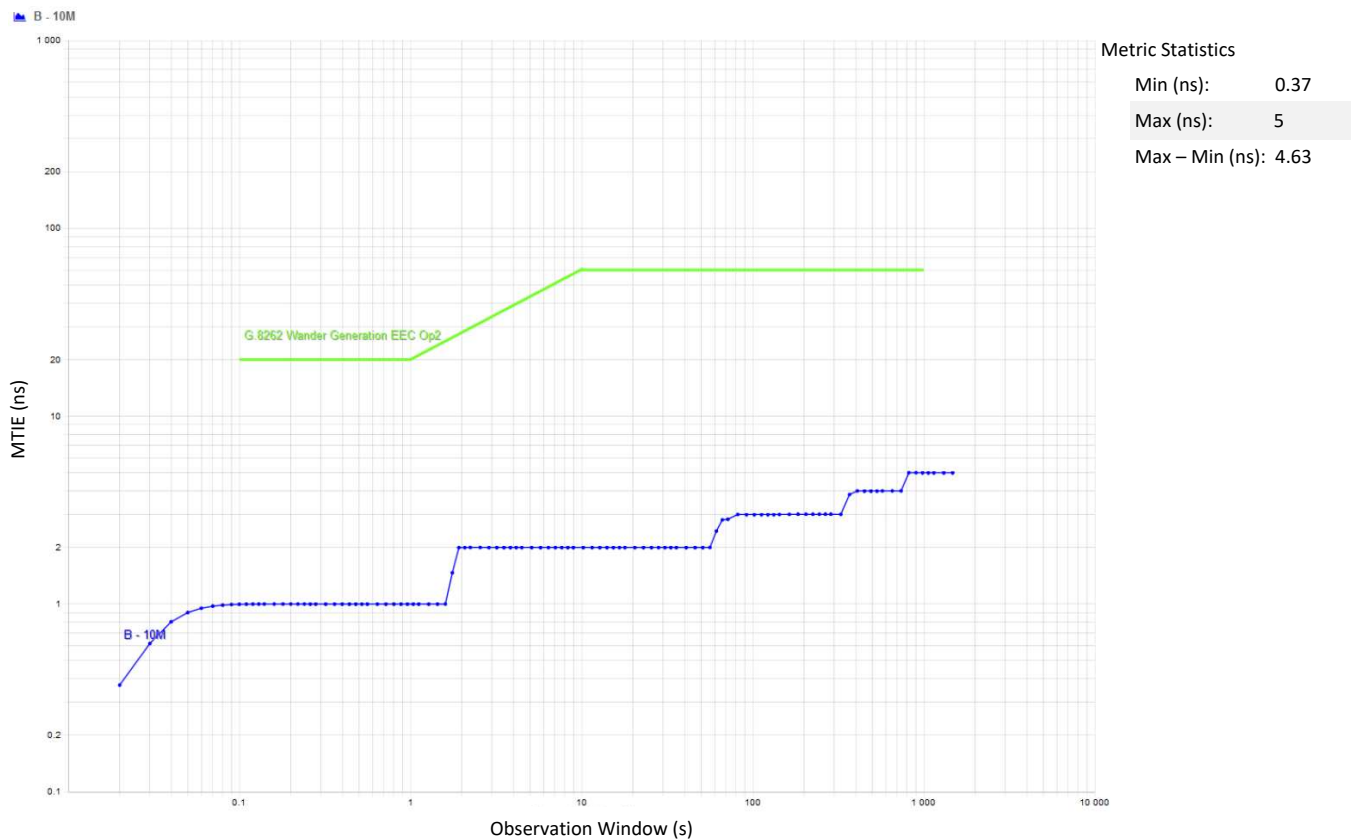
Figure 8. Wander Generation MTIE ITU-T G.8262 EEC Option 2 Results, Tested at Constant Room Temperature With DPLL Bandwidth of 0.1 Hz
