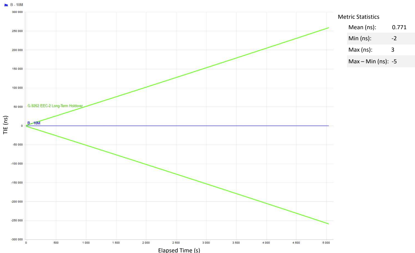
Figure 35. Holdover Option 2 Result
