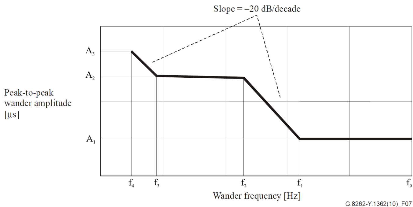
Figure 18. Lower Limit of Maximum Tolerable Sinusoidal Input Wander for EEC-Option 1
