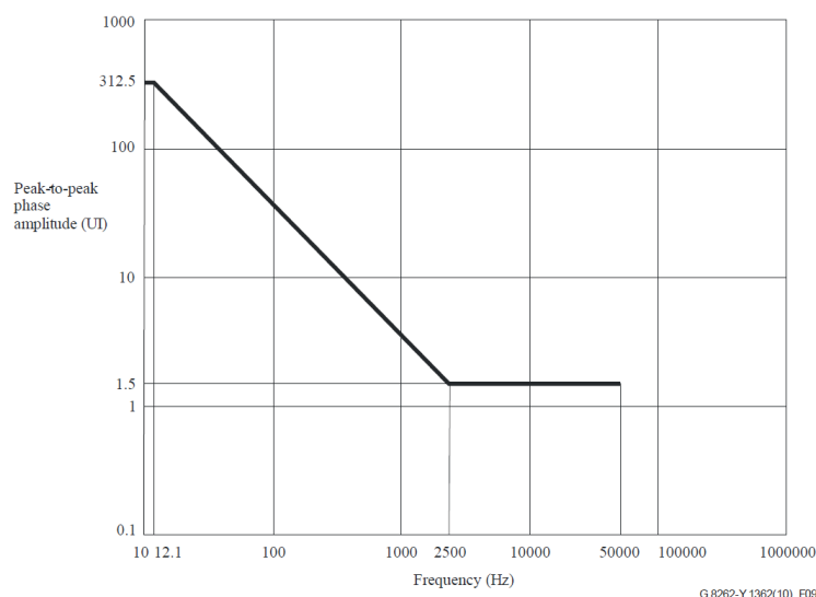
Figure 21. 1G Synchronous Ethernet Wideband Jitter Tolerance for EEC-Option 1 and EEC-Option 2
