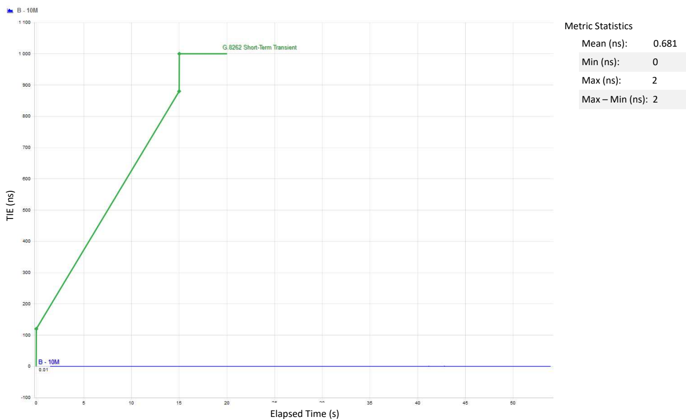
Figure 31. Phase Discontinuity Results
