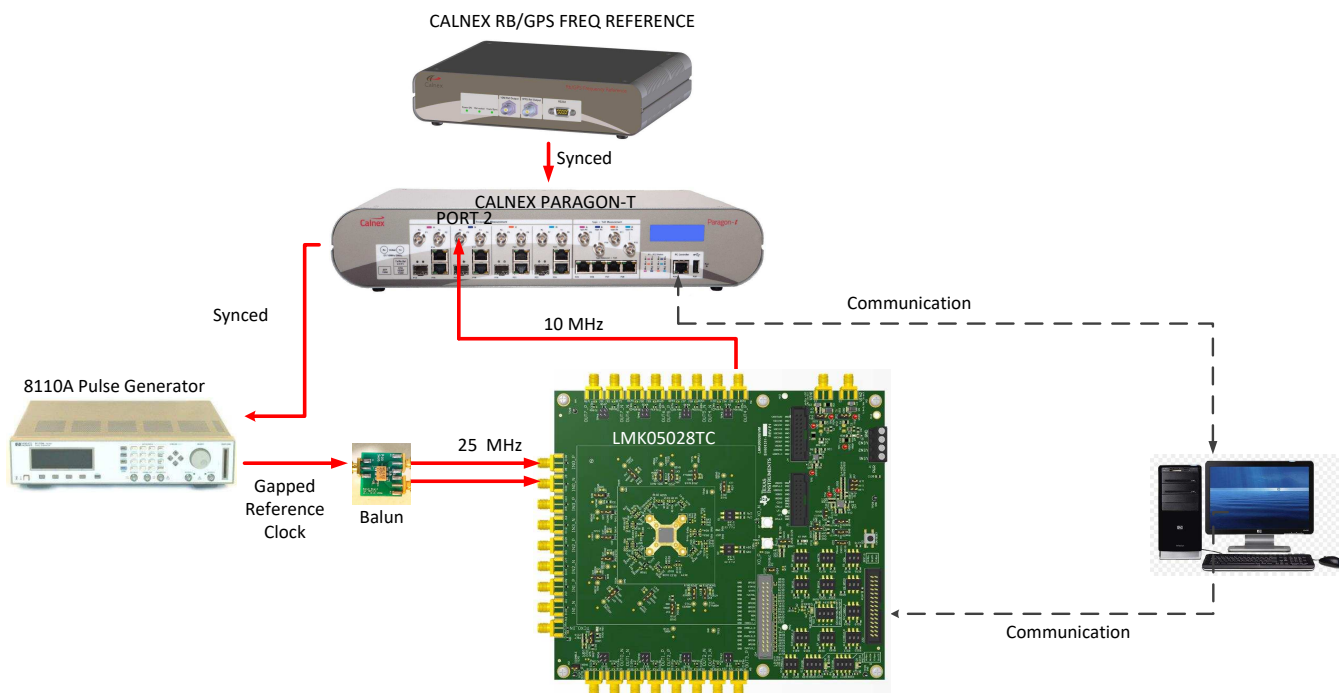
Figure 28. Test Setup for Phase Transient Generation With Signal Interruption
