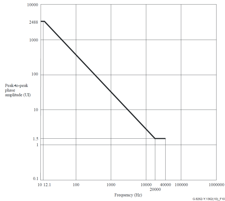
Figure 22. 10G Synchronous Ethernet Wideband Jitter Tolerance for EEC-Option 1 and EEC-Option 2
