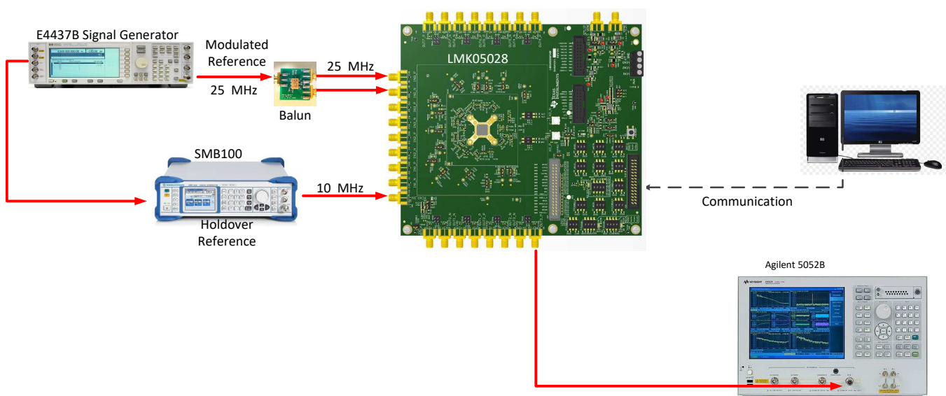
Figure 20. Test Setup for Jitter Tolerance
