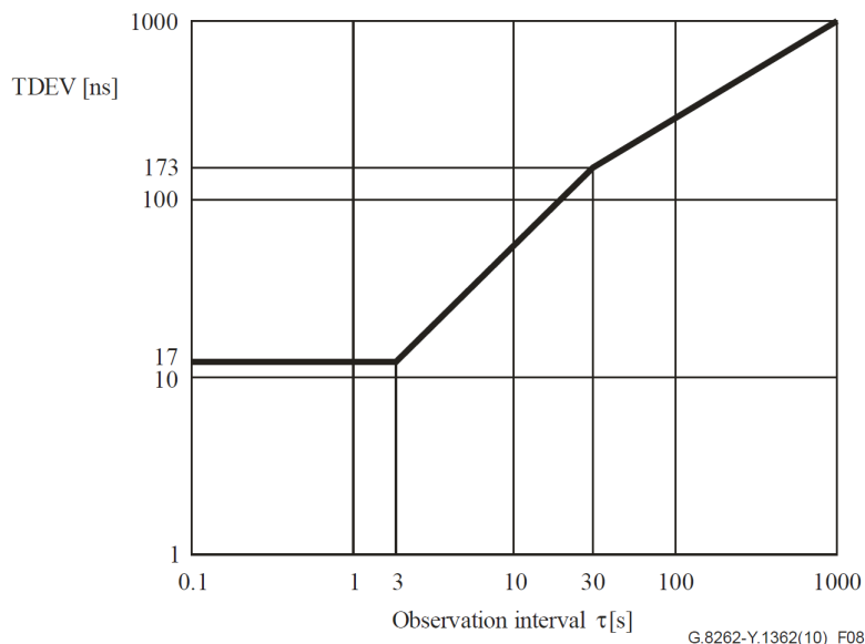
Figure 14. Input Wander Tolerance (TDEV) for EEC-Option 2
