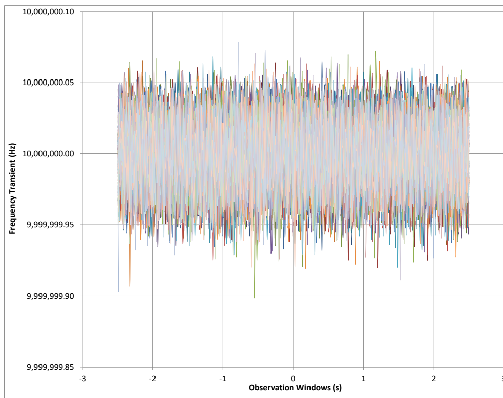
Figure 38. Frequency Transient Result
