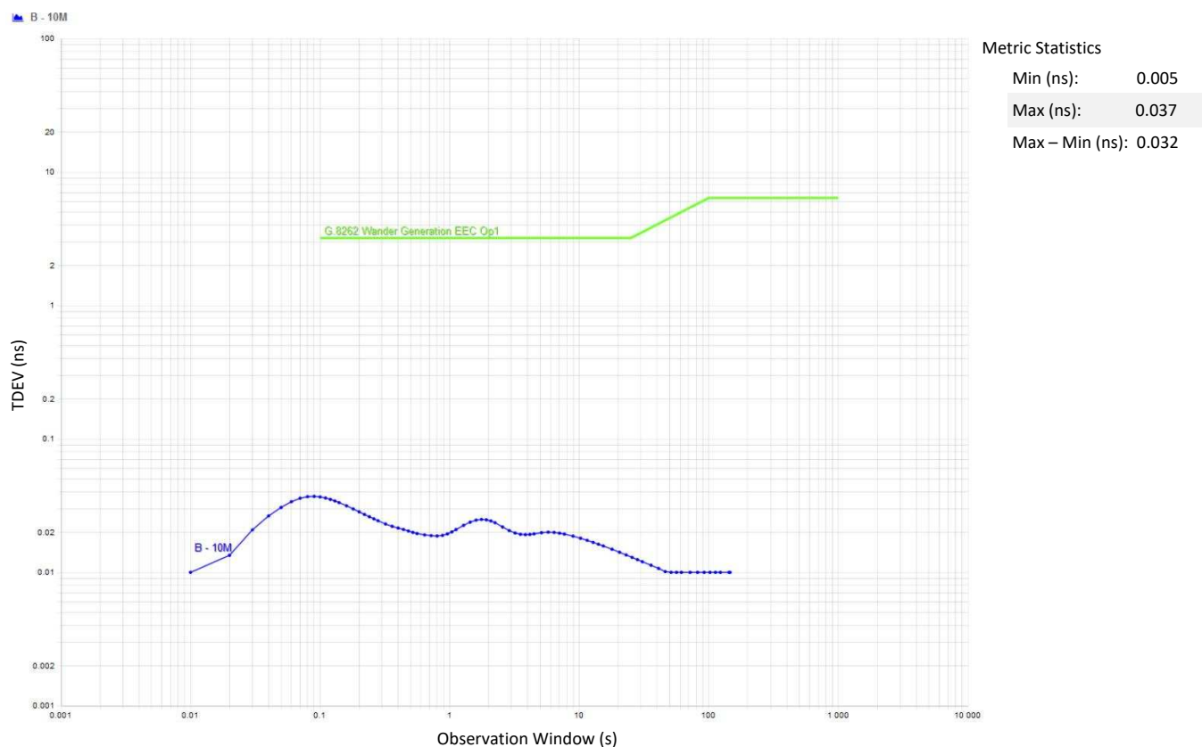
Figure 6. Wander Generation TDEV G.8262 EEC Option 1 Results, Tested at Constant Room Temperature With DPLL Bandwidth of 5 Hz
