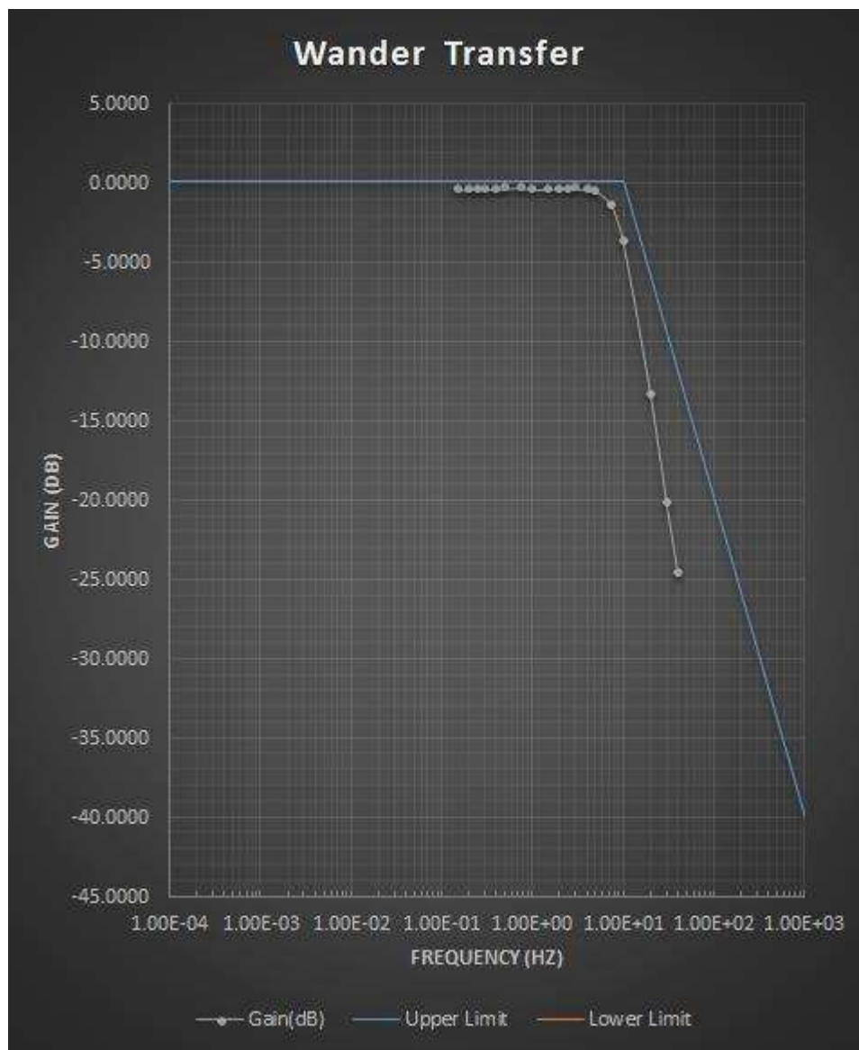
Figure 12. Wander Transfer EEC Option 1 With Max DPLL Bandwidth of 10 Hz
