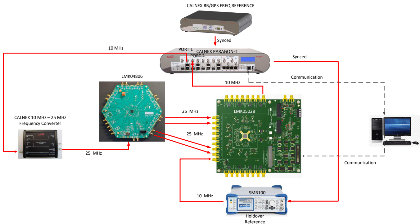
Figure 23. Test Setup for Phase Transient Generation
