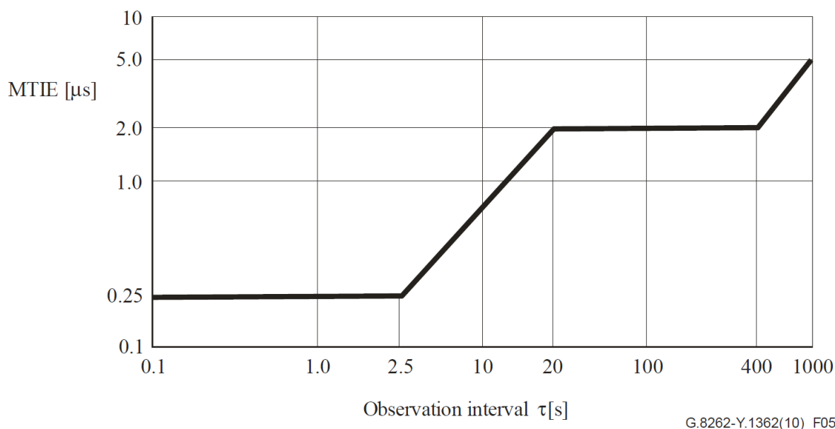
Figure 17. Input Wander Tolerance (MTIE) for EEC-Option 1
