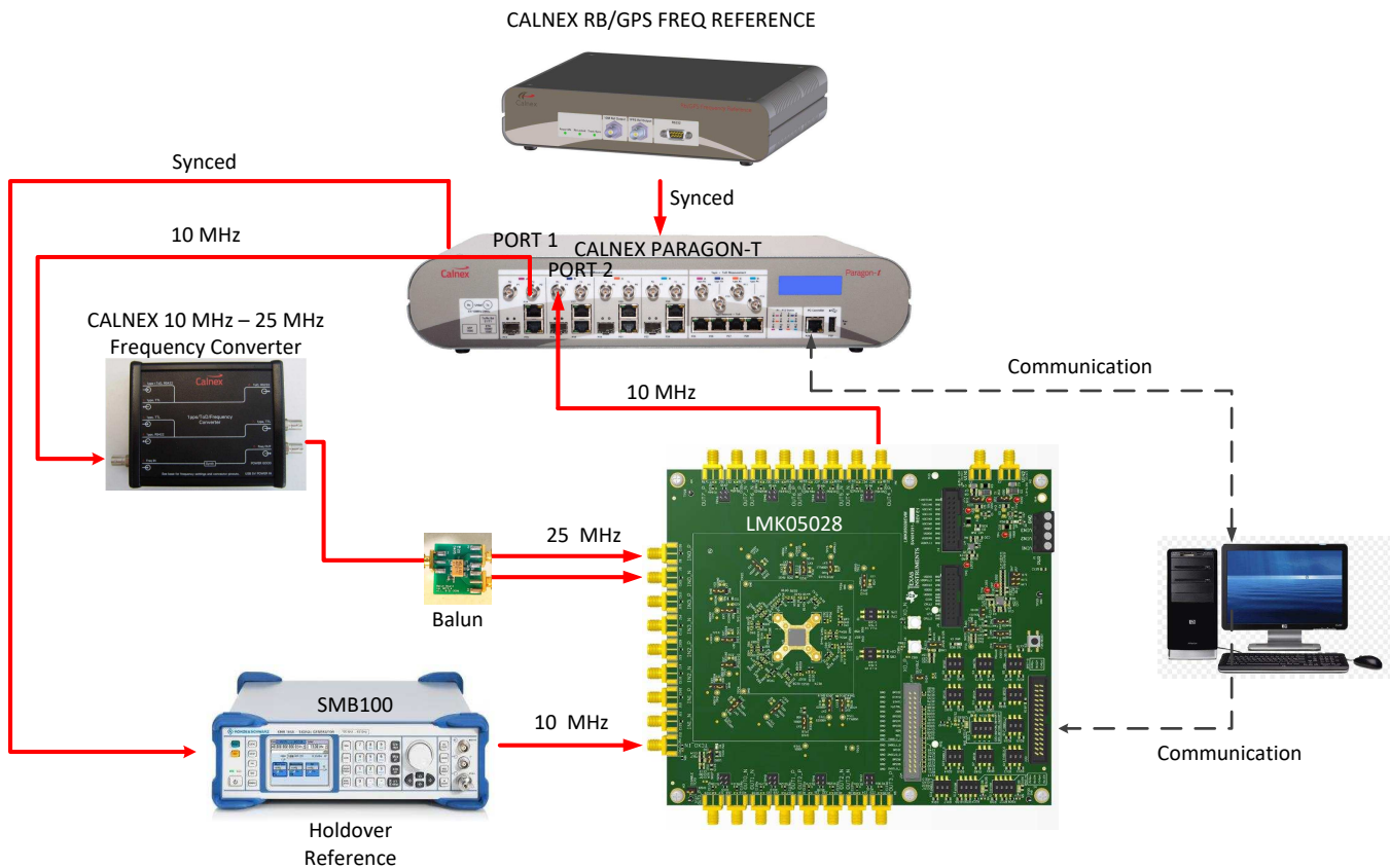
Figure 16. Test Setup for Wander Tolerance
