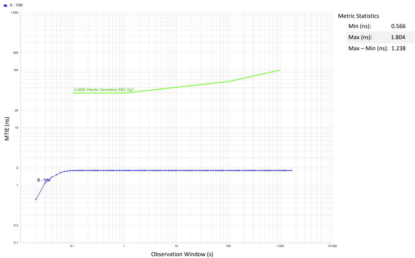
Figure 3. Wander Generation MTIE Option 1, G.8262 EEC Option 1 Results, Tested at Constant Room Temperature With DPLL Bandwidth of 10 Hz
