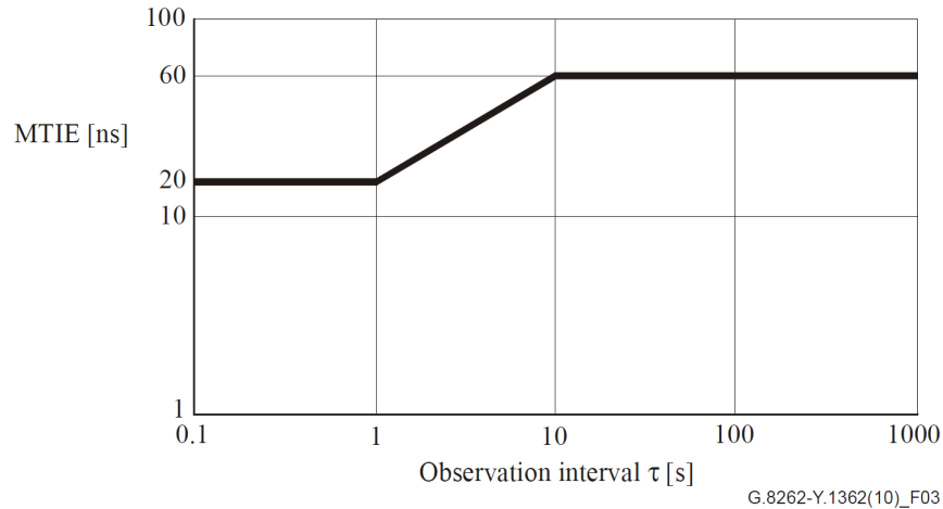
Figure 7. Wander Generation (MTIE) for EEC-Option 2 With Constant Temperature
