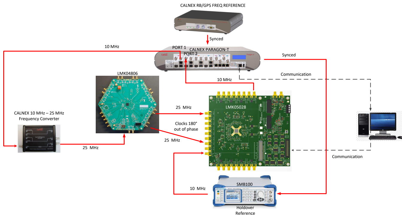
Figure 30. Test Setup for Phase Discontinuity
