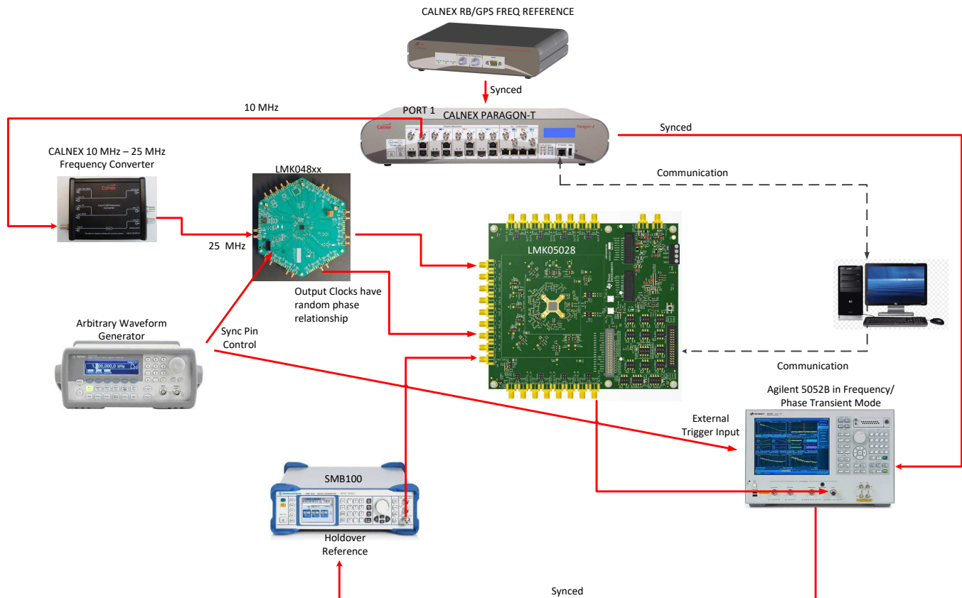
Figure 36. Alternate Test Setup to Measure Phase Transient Response Accurately
