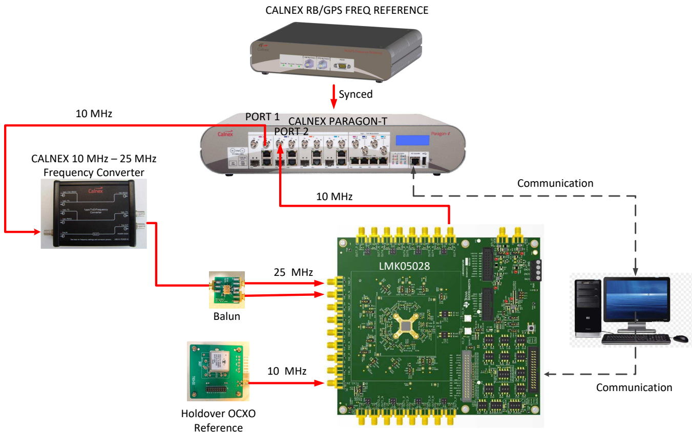
Figure 11. Test Setup for Wander Transfer
