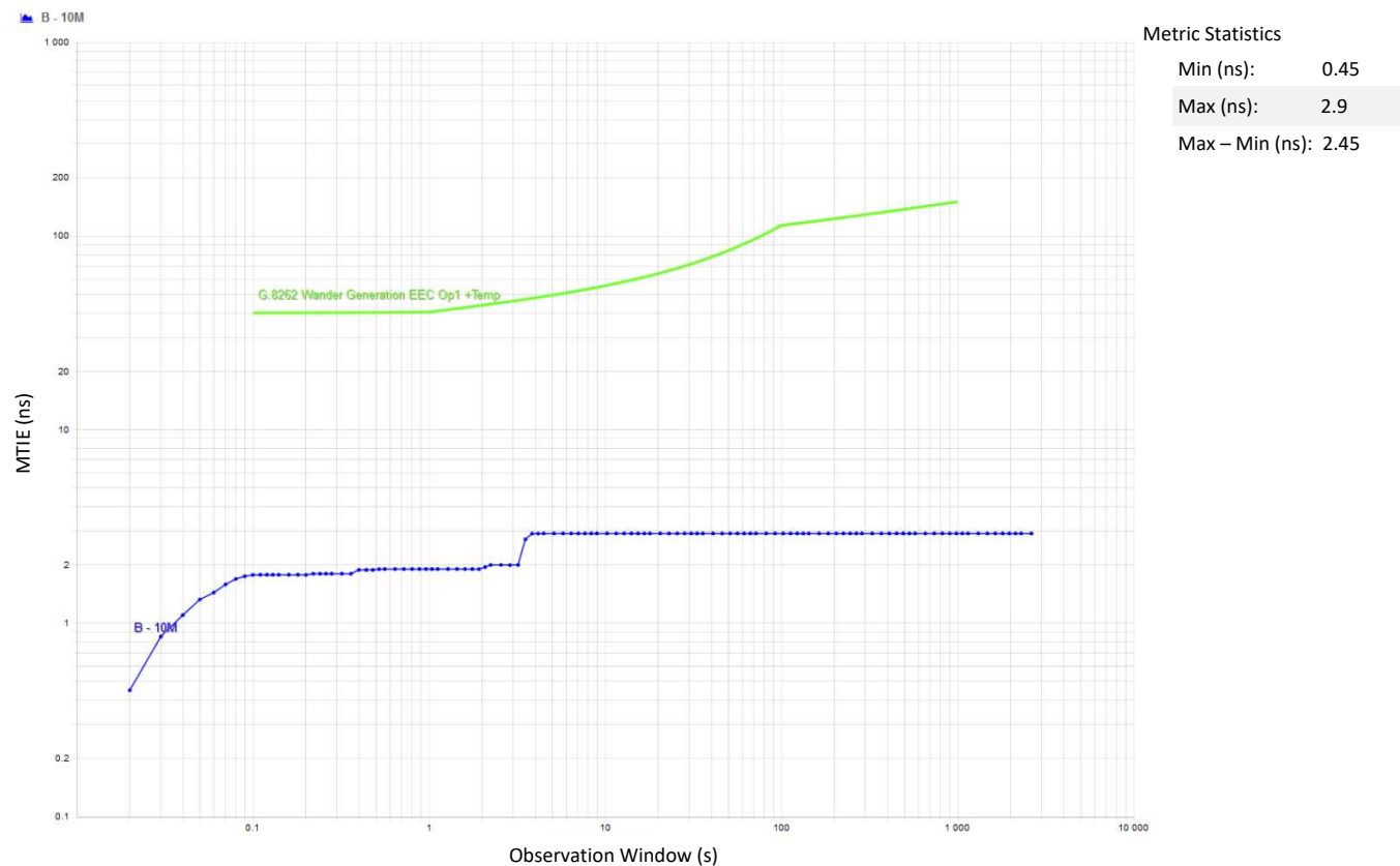
Figure 4. Wander Generation MTIE Option 1, G.8262 EEC Option 1 Results, Tested at Temperature of 85°C With DPLL Bandwidth of 10 Hz
