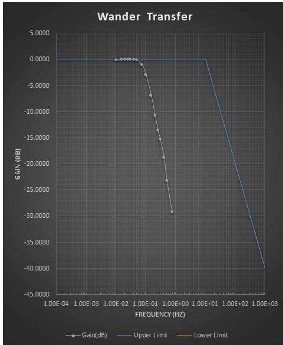
Figure 13. Wander Transfer EEC Option 2 With Max DPLL Bandwidth of 0.1 Hz
