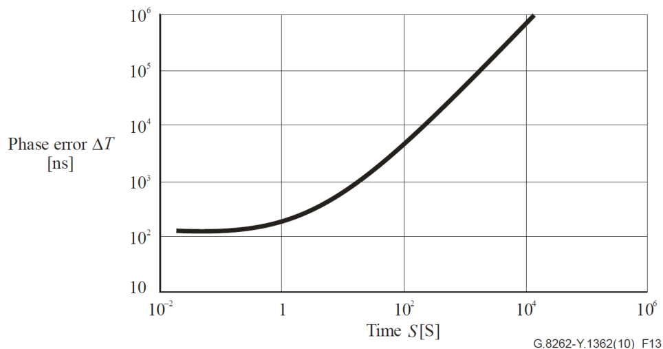
Figure 33. Permissible Phase Error for an EEC-Option 1 Under Holdover Operation at Constant Temperature
