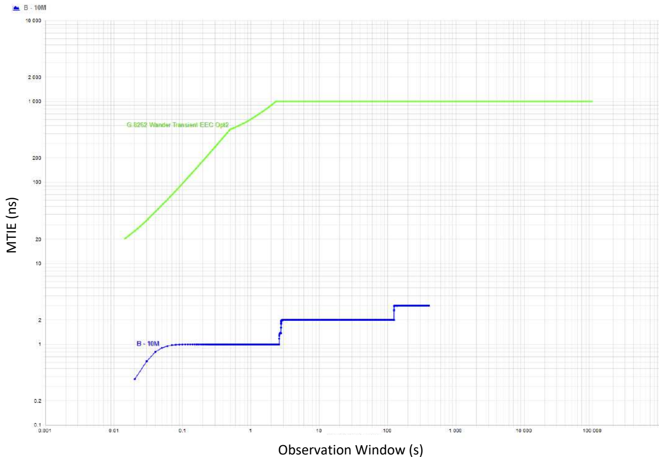
Figure 32. Phase Discontinuity Option 2 Results
