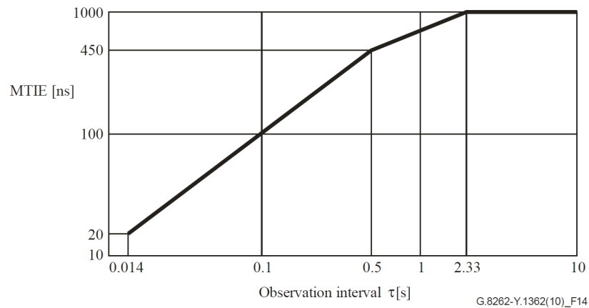
Figure 26. MTIE at the Output Due to Reference Switching/Rearrangement Operations for EEC-Option 2
