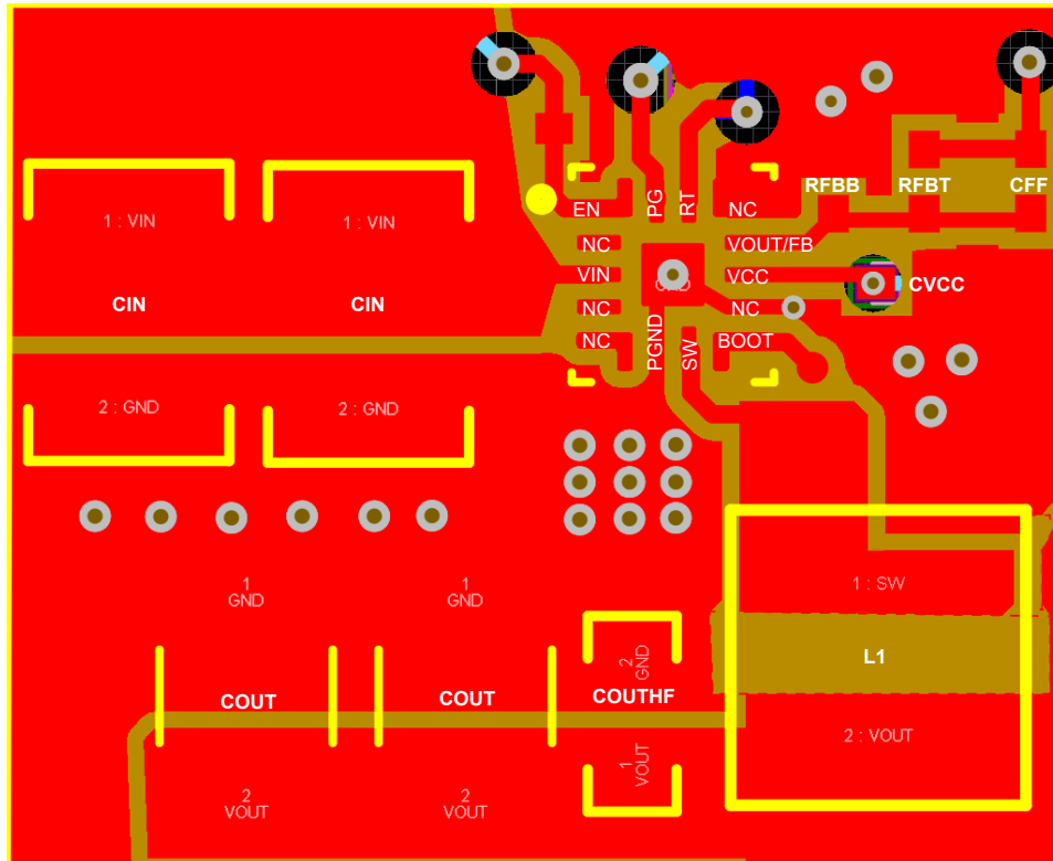
Figure 11-2. Example Layout
