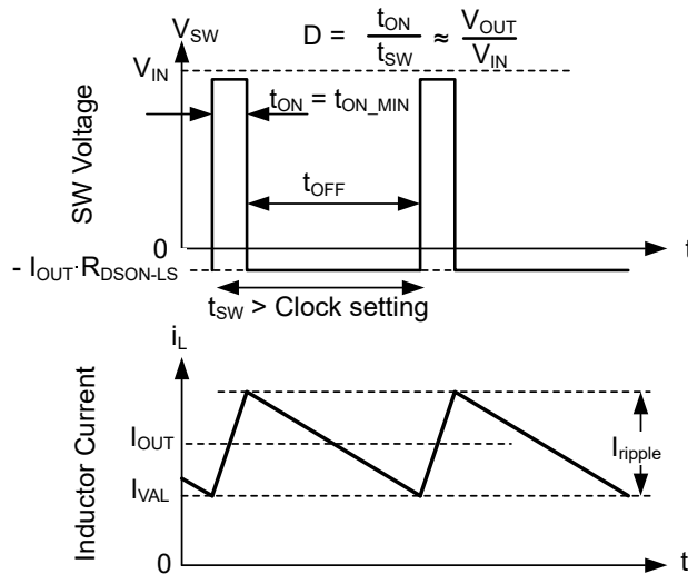
Figure 8-20. Valley Current Mode Operation
