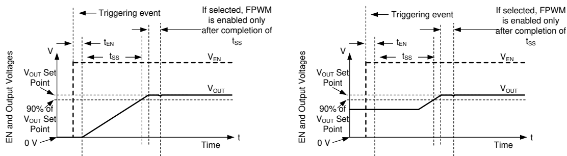
Figure 8-11. Soft Start with and Without Pre-bias Voltage
