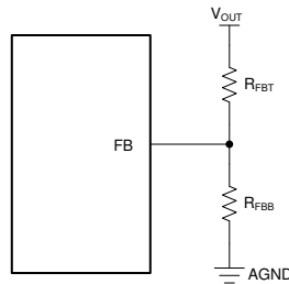
Figure 8-10. Setting Output Voltage for Adjustable Output Variant
