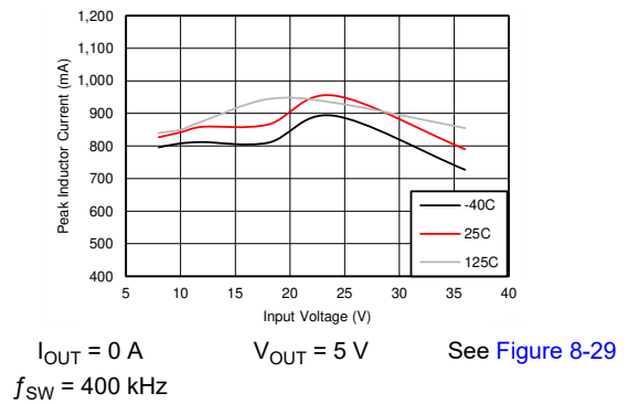
Figure 6-6. I PEAK-MIN
