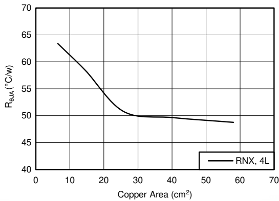
Figure 8-3. R_{\theta JA} versus Copper Board Area for the VQFN (RNX) Package
