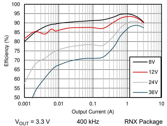
Figure 8-6. Efficiency
