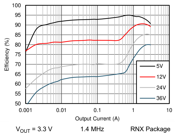
Figure 8-8. Efficiency
