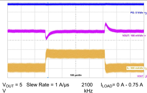
Figure 9-10. Load Transient Waveform
