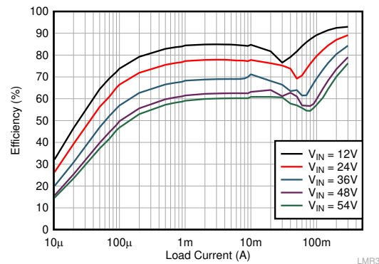
V_{OUT} = 5\text{ V Fixed} F_{SW-NOM} = 1\text{ MHz (Auto)}
