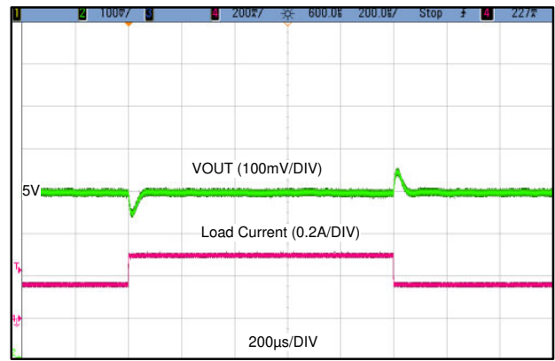
LMR36503R5 V_{OUT} = 5\text{ V Fixed} 400 kHz 0.15 A to 0.3 A, 1 A/µs
