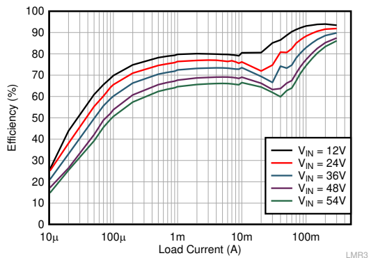
V_{OUT} = 5\text{ V Fixed} F_{SW} = 400\text{ kHz (Auto)}
