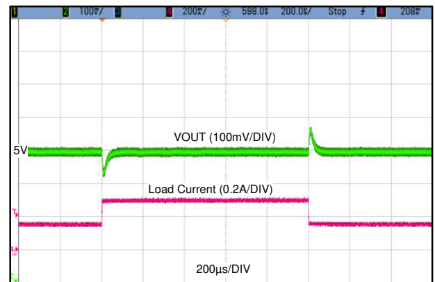
LMR36503R5 V_{OUT} = 5\text{ V Fixed} 1 MHz 0.15 A to 0.3 A, 1 A/µs
