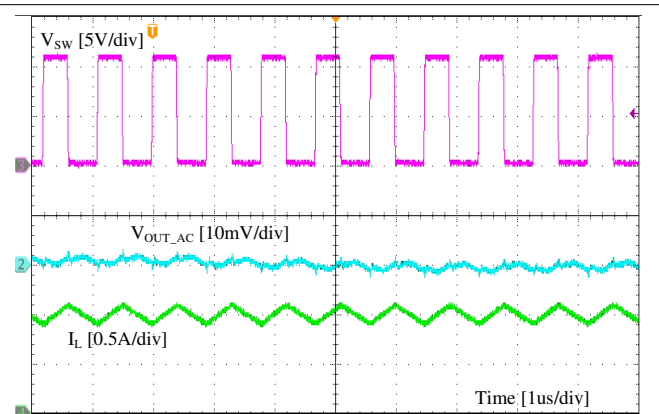
Figure 9-4. Ripple at Full Load
