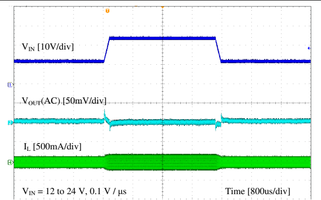
Figure 9-8. Line Transient
