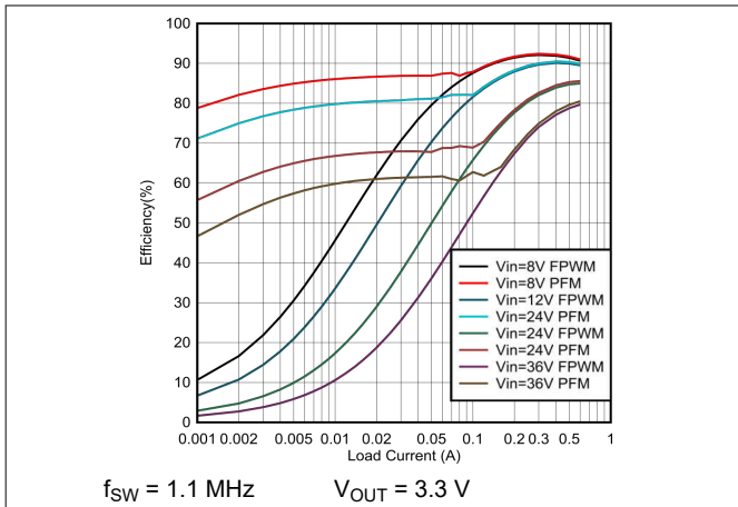
Figure 7-1. 3.3-V Efficiency Versus Load Current - LMR54406
