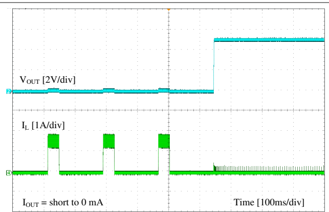
Figure 9-10. Short Recovery
