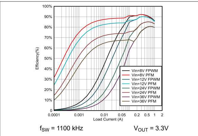
Figure 7-2. 3.3-V Efficiency Versus Load Current - LMR54410
