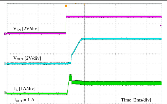
Figure 9-6. Start-Up by EN
