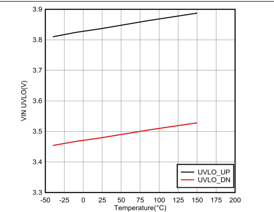
Figure 7-11. V_{IN} UVLO Versus Temperature
