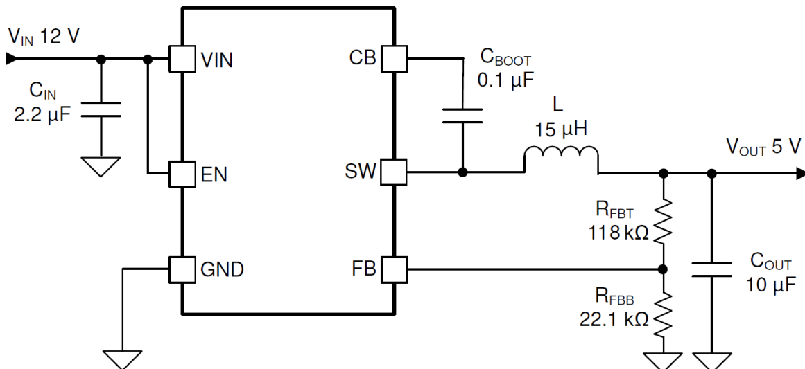
Figure 9-1. Application Circuit
