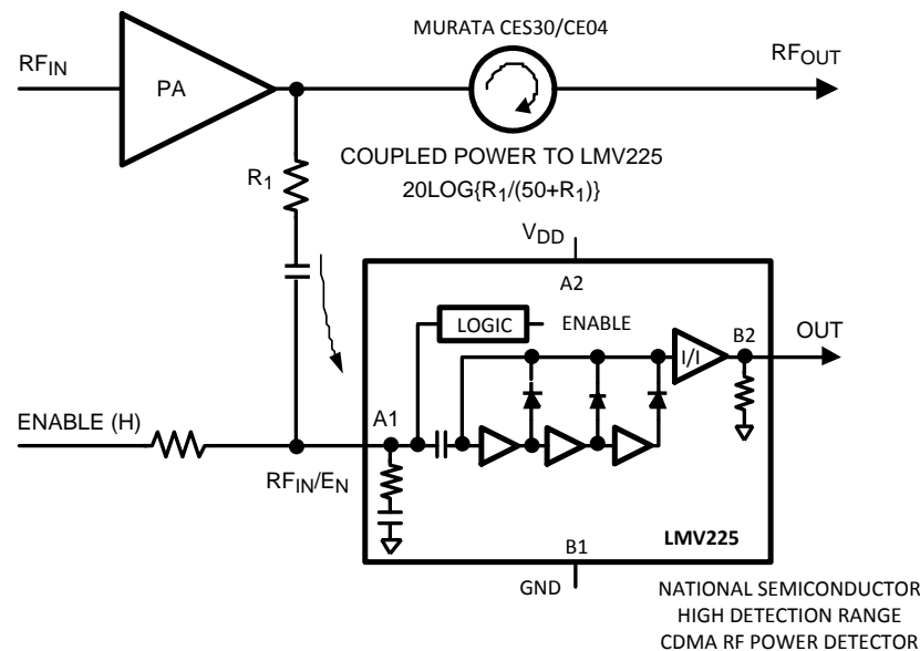
Figure 2. Transmit Radio Architecture
