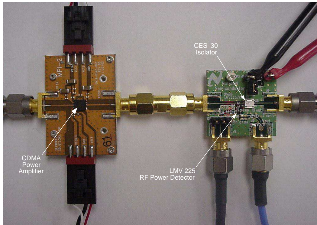
Figure 4. LMV225 Eval Board + CDMA PA's Module
