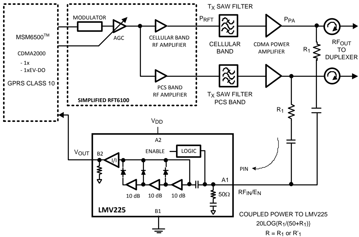
Figure 8. Dual-Band CDMA2000 Transmit Architecture
