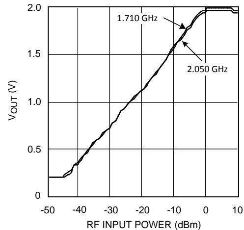
Figure 7. Typical Performance at DCS/PCS/W-DCMA Bands
