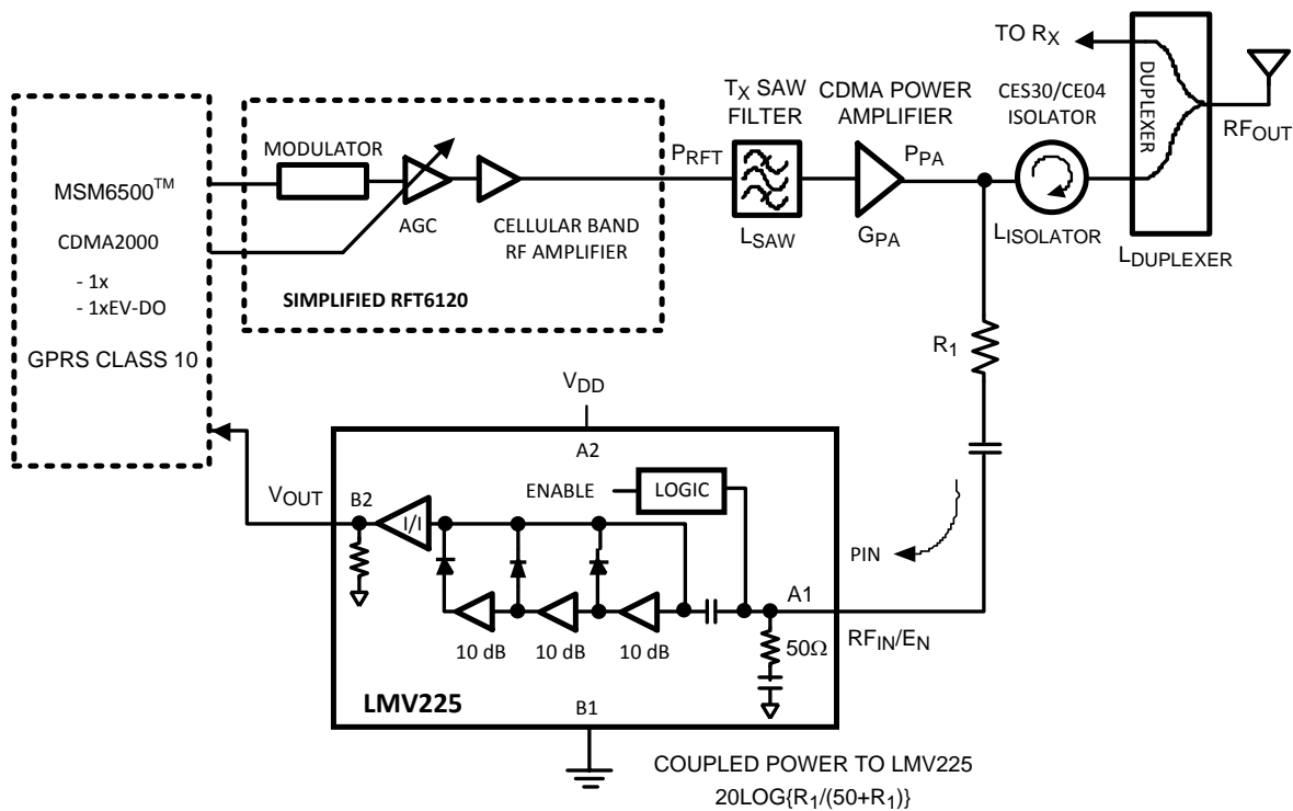
Figure 5. Single-Band CDMA2000 T x Architecture
