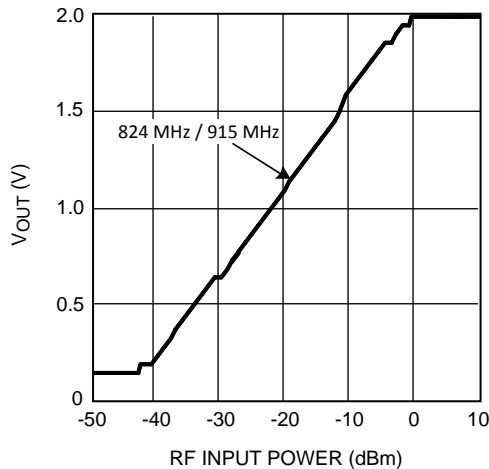
Figure 6. Typical Performance at Cellular Bands
