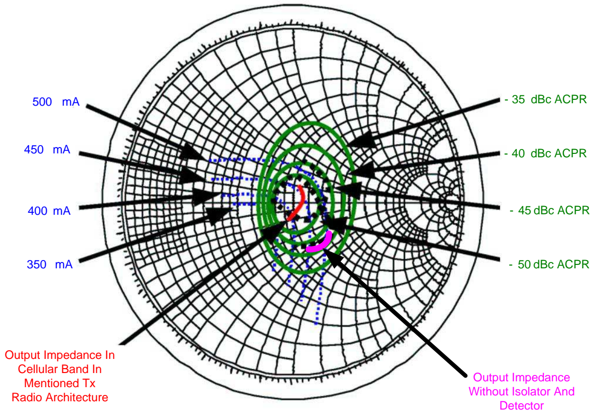
Figure 3. Output Impedance Smith Chart
