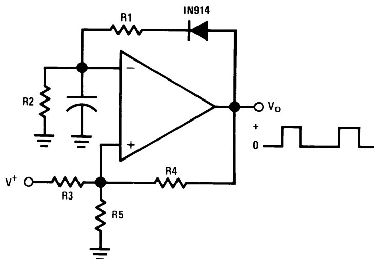
Figure 9-13. Pulse Generator
