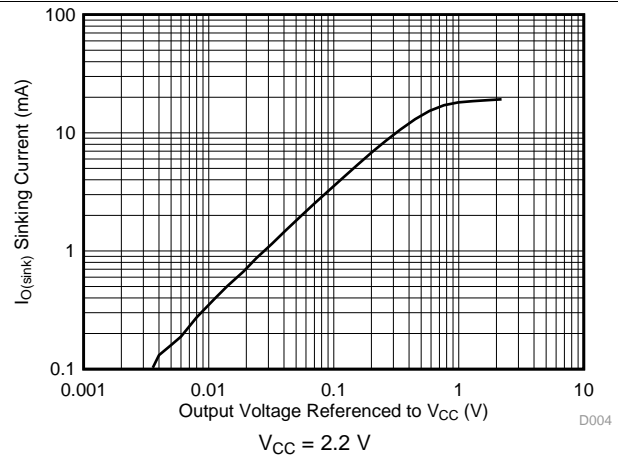
Figure 4. Sinking Current vs Output Voltage
