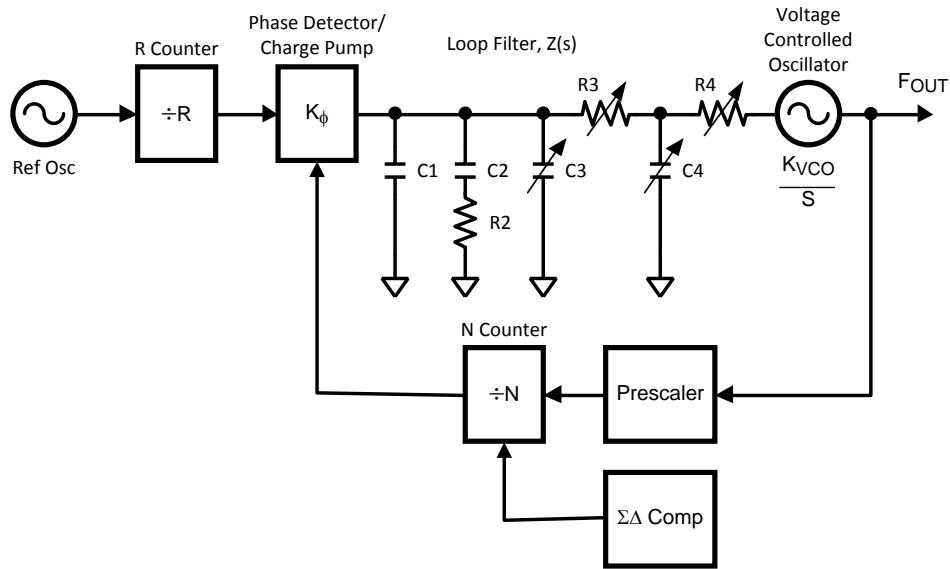
Figure 1. LMX2531LQ1500E Block Diagram
