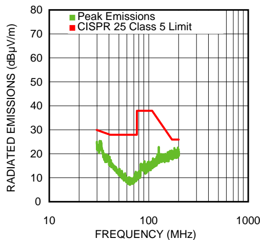
Figure 16. 30 MHz-200 MHz Horizontal 1A Load
