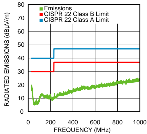
Figure 11. Radiated EMI With the LC Input Filter 1A Load
