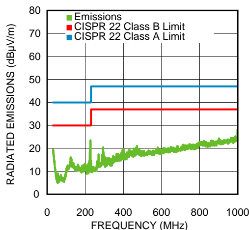
Figure 1. CISPR 22 Radiated EMI 1A Load Default Evaluation Board BOM
