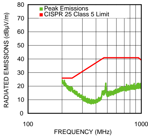
Figure 20. 200 MHz-1000 MHz Horizontal 1A Load
