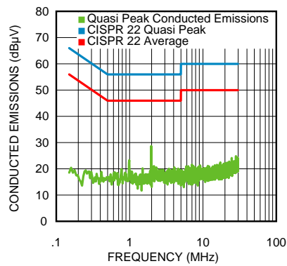
Figure 9. Conducted EMI with the LC Input Filter 1A Load
