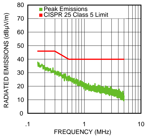
Figure 13. 0.15 MHz-5 MHz 650 mA Load
