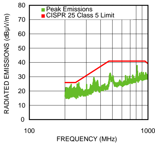
Figure 22. 200 MHz-1000 MHz Vertical 1A Load
