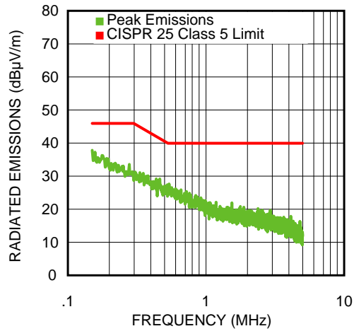
Figure 12. 0.15 MHz-5 MHz 1A Load
