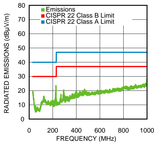
Figure 6. Radiated EMI 1A Load
