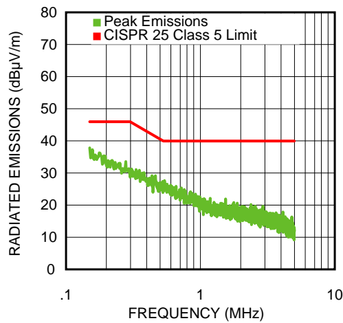
Figure 4. CISPR 25 Class 5 Radiated EMI 1A Load 2 x 0.1µF Additional Input Capacitance
