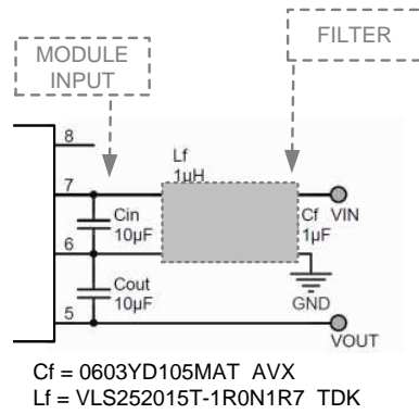
Figure 8. LC Input Filter for Conducted EMI
