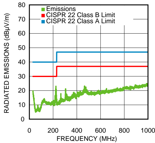
Figure 7. Radiated EMI 650mA Load
