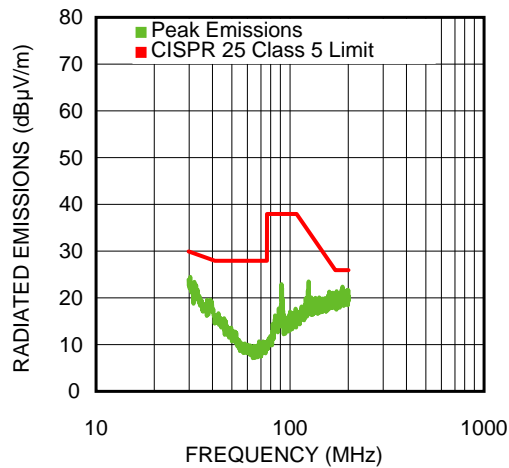
Figure 19. 30 MHz-200 MHz Vertical 650 mA Load
