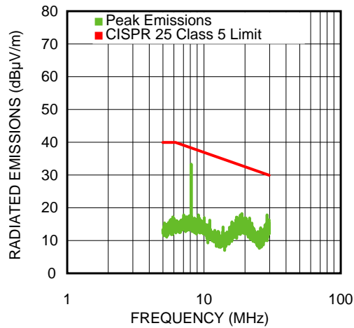
Figure 14. 5 MHz-30 MHz 1A Load
