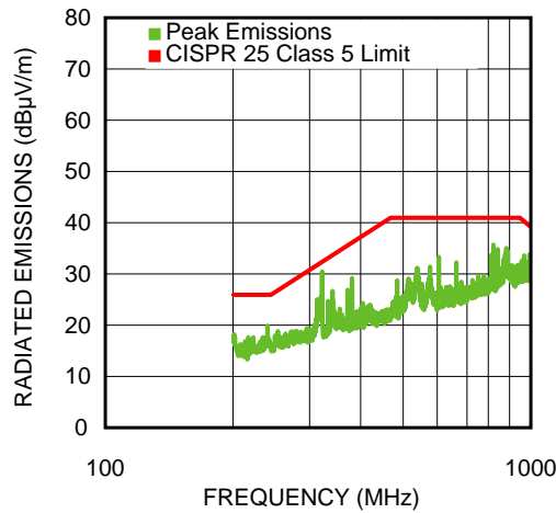
Figure 21. 200 MHz-1000 MHz Horizontal 650 mA Load
