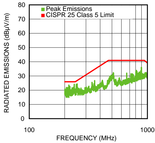
Figure 23. 200 MHz-1000 MHz Vertical 650 mA Load
