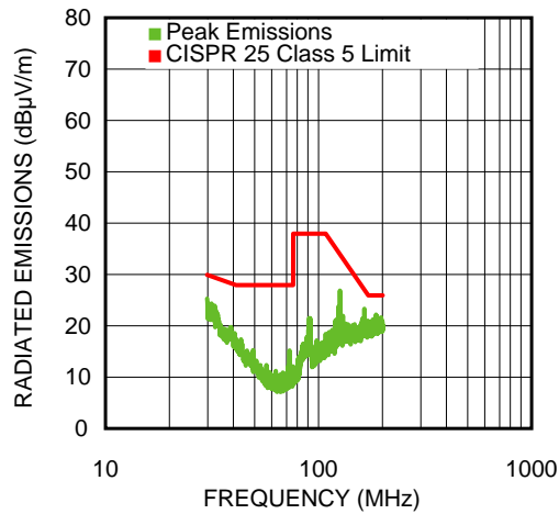
Figure 18. 30 MHz-200 MHz Vertical 1A Load
