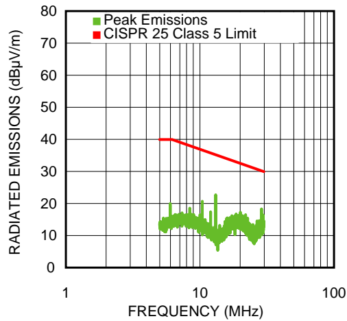
Figure 15. 5 MHz-30 MHz 650 mA Load
