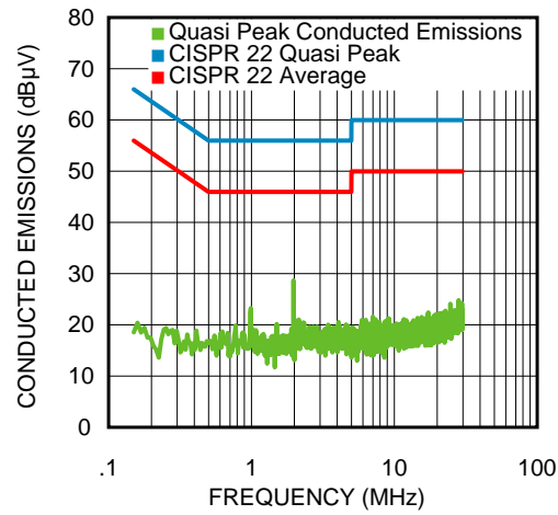
Figure 2. CISPR 22 Conducted EMI 1A Load 1µH 1µF Additional LC Input Filter
