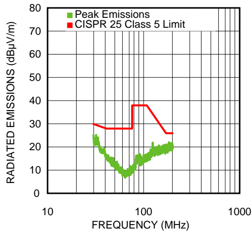
Figure 17. 30 MHz-200 MHz Horizontal 650 mA Load
