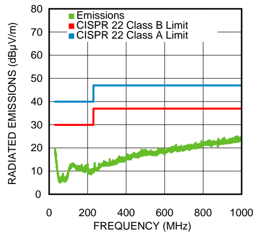
Figure 3. CISPR 22 Radiated EMI 1A Load 1µH 1µF Additional LC Input Filter
