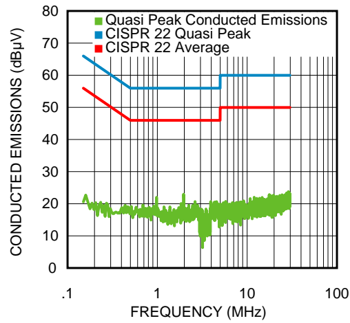
Figure 10. Conducted EMI With the LC Input Filter 650mA Load
