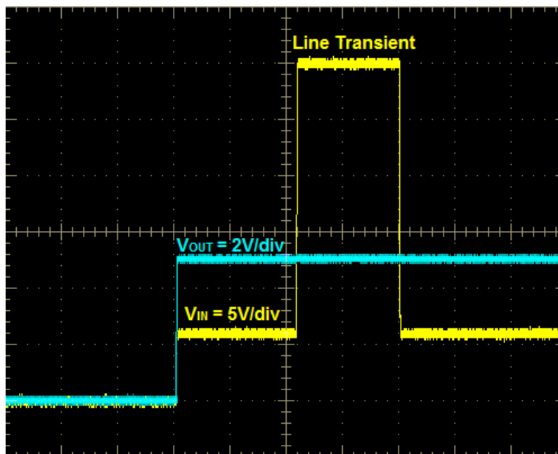
Figure 1. Line Transient Waveform
