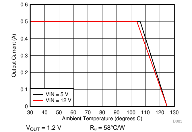
Figure 16. Ambient Temperature vs Output Current
