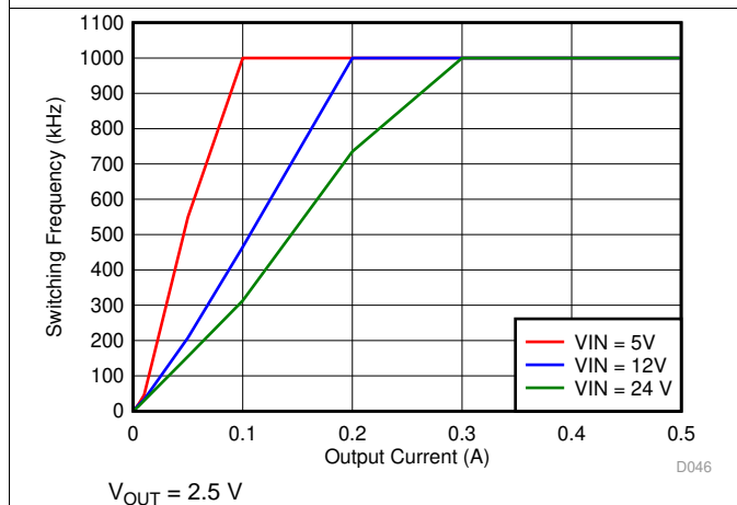
Figure 23. Auto PFM Mode Switching Frequency vs Output Current
