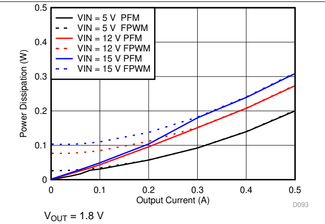
Figure 14. Power Dissipation
