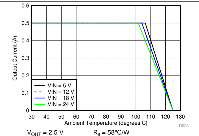
Figure 18. Ambient Temperature vs Output Current
