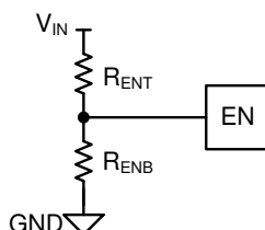
Figure 38. Enable Divider to Set External UVLO Threshold
