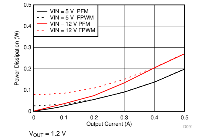
Figure 15. Power Dissipation
