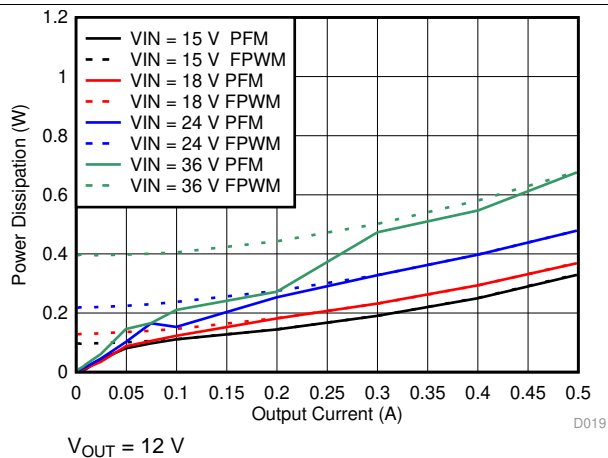
Figure 10. Power Dissipation
