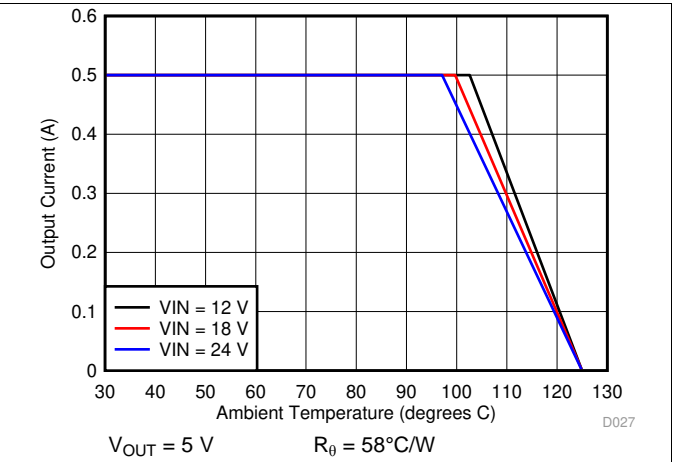
Figure 20. Ambient Temperature vs Output Current
