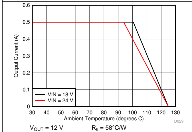
Figure 21. Ambient Temperature vs Output Current
