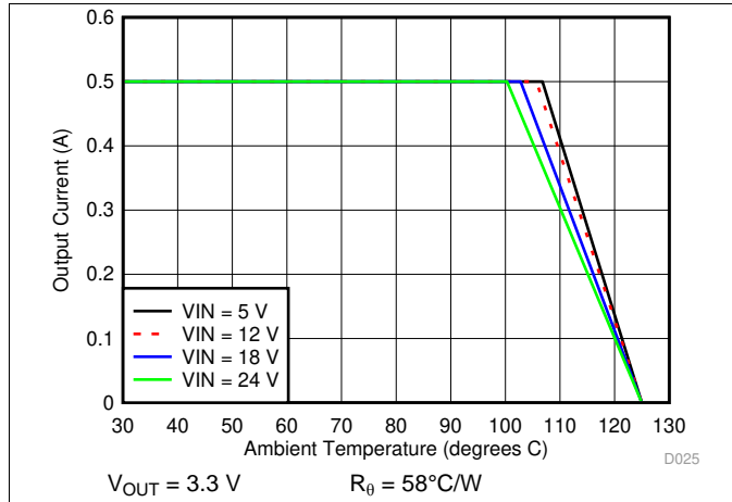
Figure 19. Ambient Temperature vs Output Current
