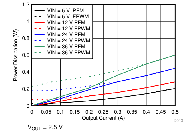
Figure 13. Power Dissipation
