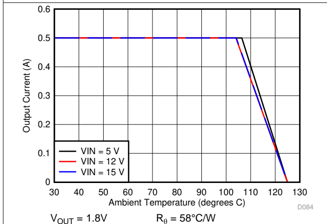
Figure 17. Ambient Temperature vs Output Current
