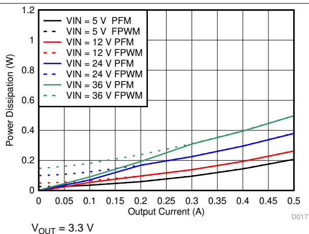
Figure 12. Power Dissipation
