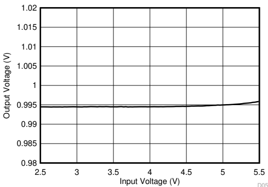
Figure 8-22. LDO Output Voltage vs Input Voltage V_{OUT} = 1\text{ V} Load = 200 mA
