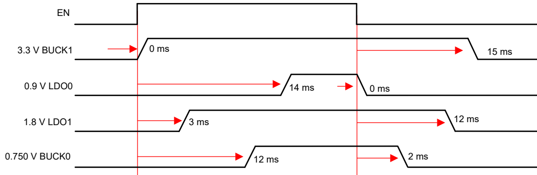
Figure 3-1. LP873345 Power-up and Power Down Sequence
