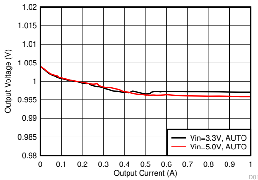
V_{OUT} = 1\text{ V} Figure 8-6. Buck Output Voltage vs Load Current in PFM/PWM Mode
