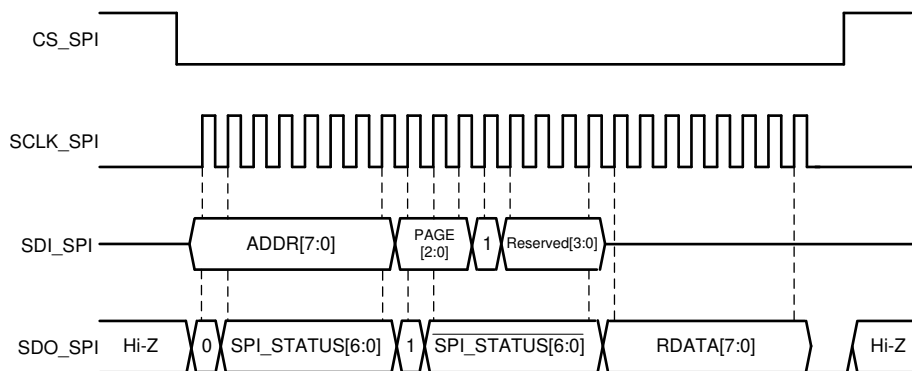
Figure 8-34. SPI Read Cycle
