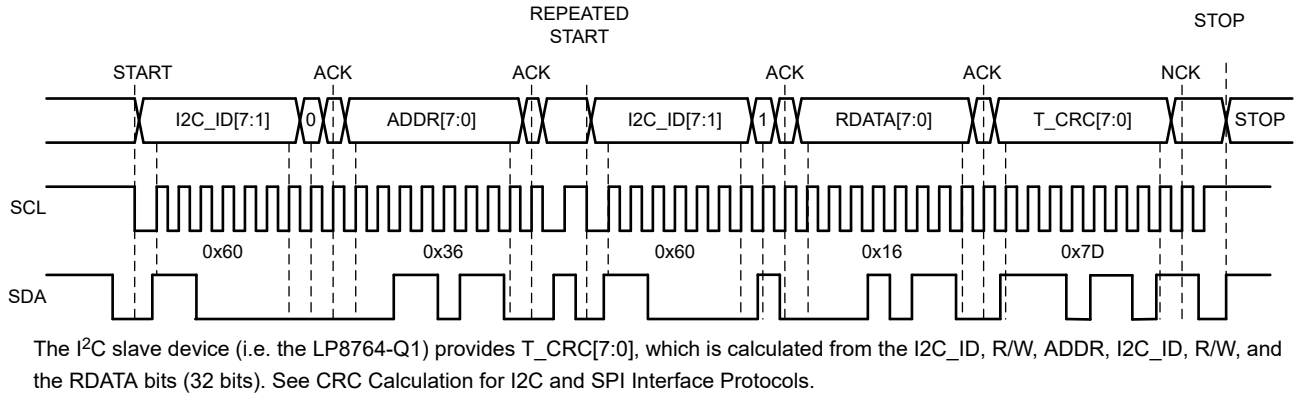
Figure 8-31. I²C READ Cycle with CRC
