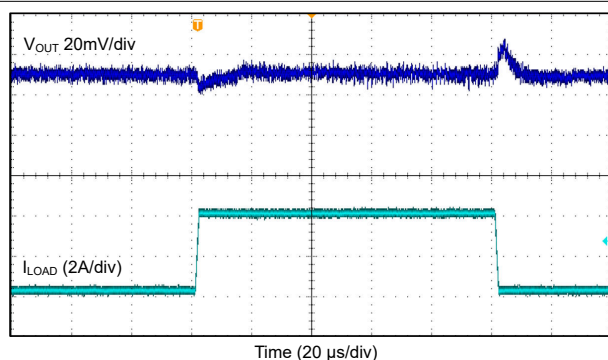
Figure 9-52. Load Transient Response, Auto Mode. 2.2 MHz Single Phase.
