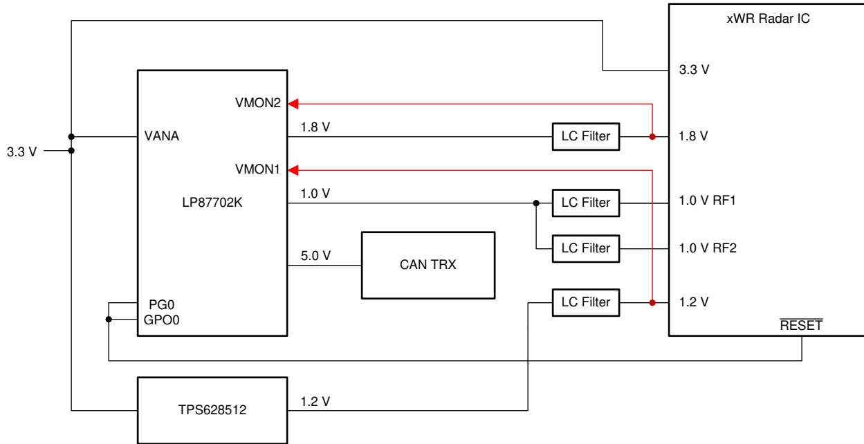
Figure 1. Typical Connection to LP87702K
