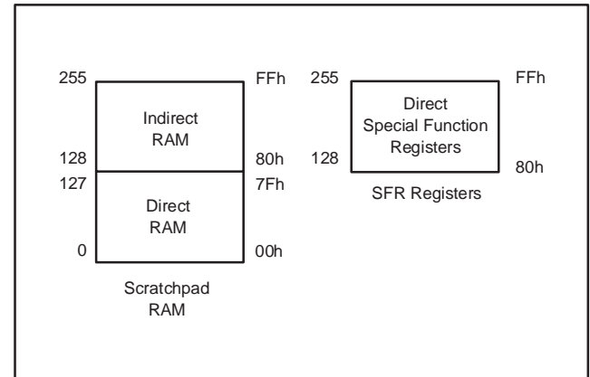
Figure 22. Register Map
