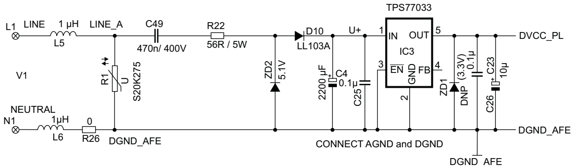
Figure 3. A Simple Capacitive Power Supply for the MSP430 Energy Meter
