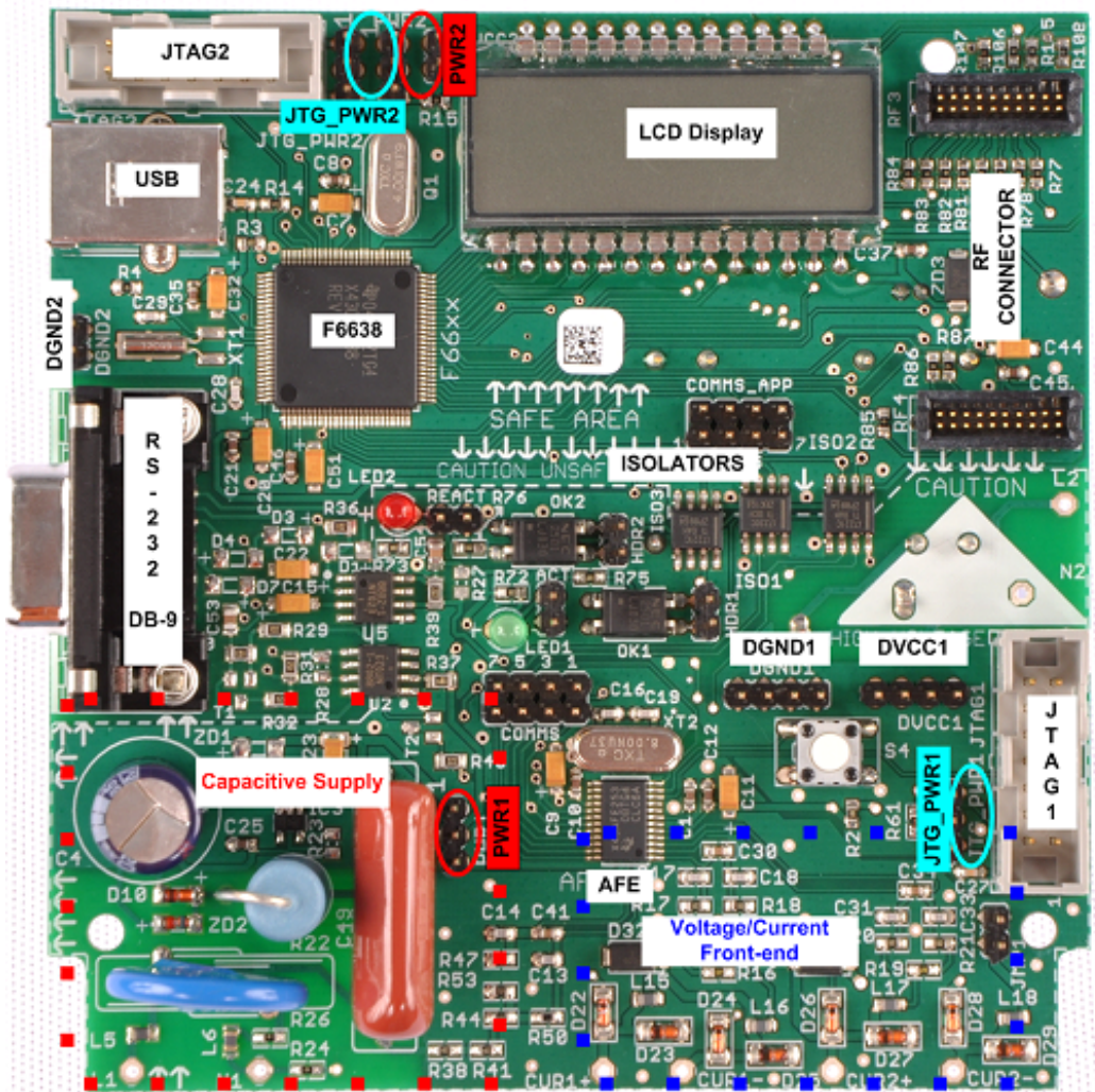
Figure 13. Top View of the EVM With Blocks and Jumpers
