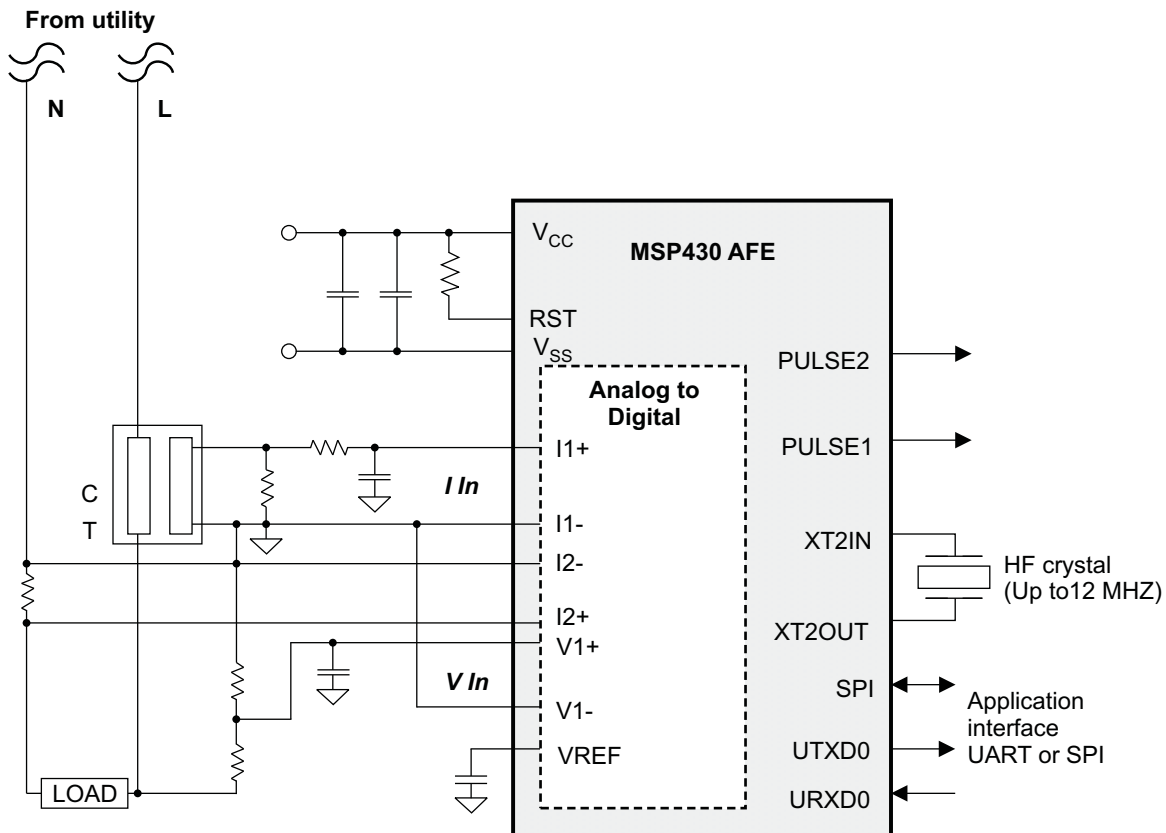
Figure 2. One-Phase Two-Wire Star Connection Using MSP430AFE2x3
