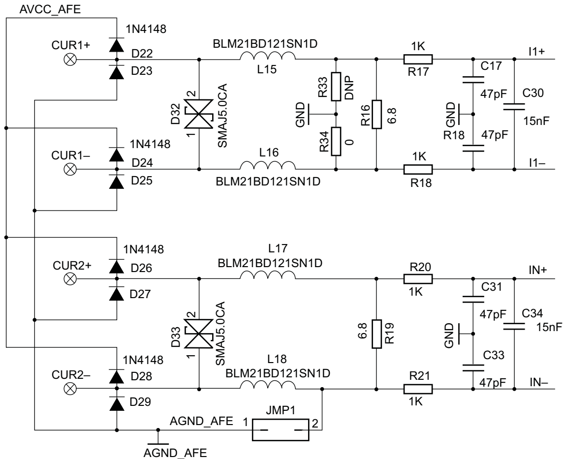
Figure 6. Analog Front End for Current Inputs
