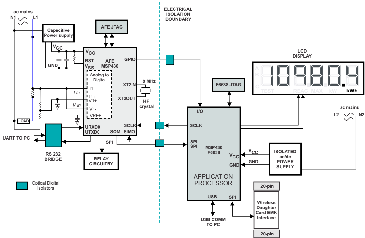
Figure 1. Energy Meter EVM System Block Diagram
