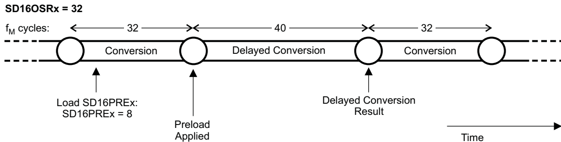
Figure 9. Phase Compensation Using PRELOAD Register
