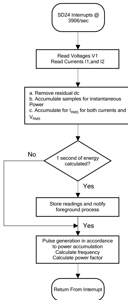
Figure 8. Background Process
