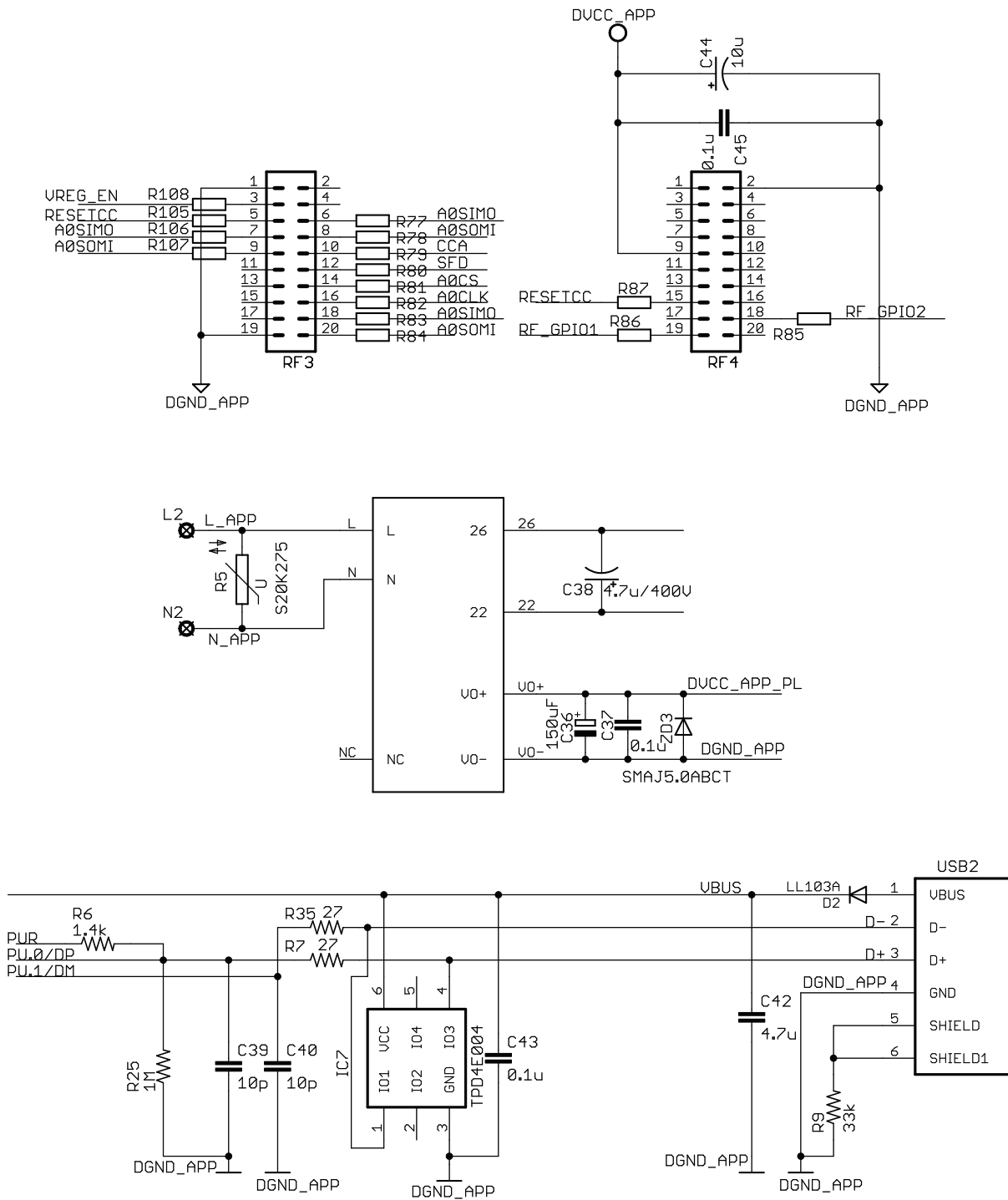
Figure 21. Schematic 3
