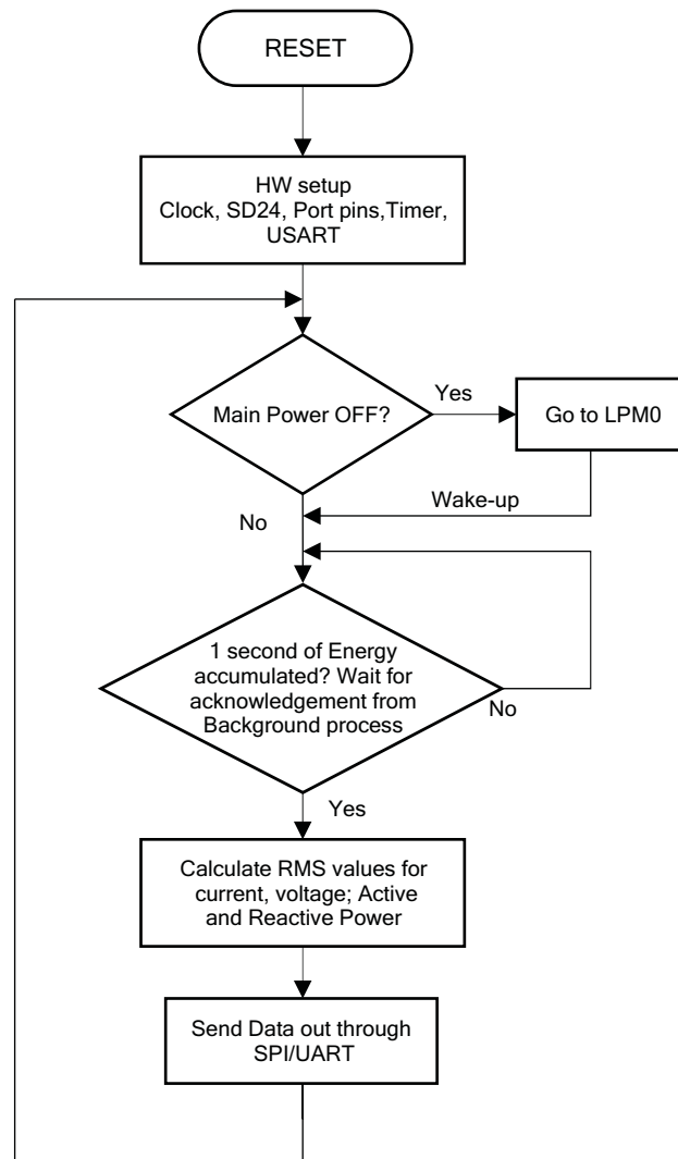
Figure 7. Foreground Process
