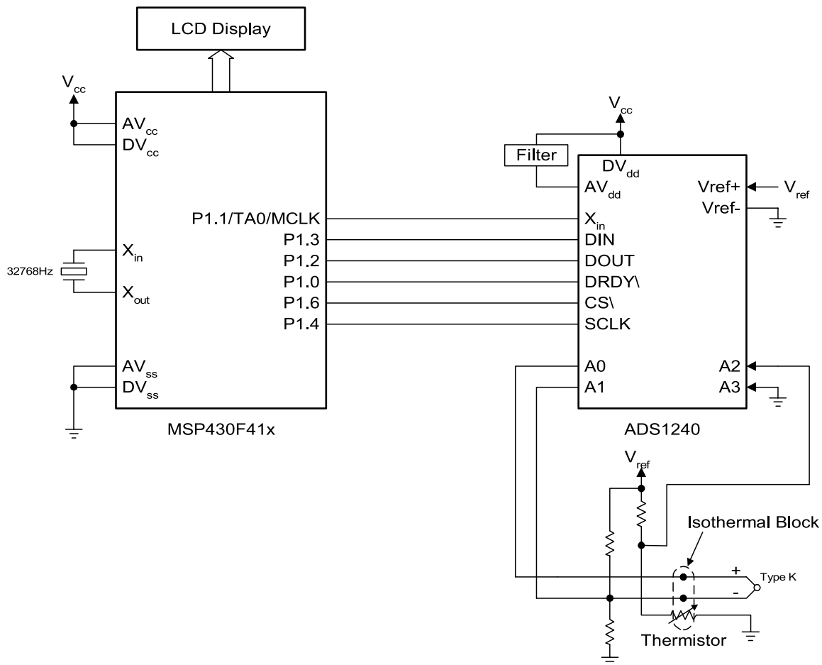
Figure 1. Circuit Diagram
