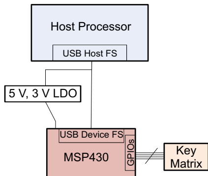
Figure 3. HID USB Keyboard Block Diagram
