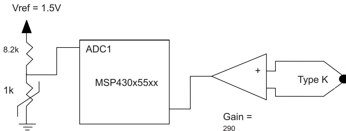
Figure 4. Hardware Block Diagram
