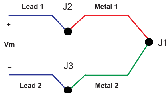
Figure 2. Measuring Thermocouple Voltage with a Voltmeter
