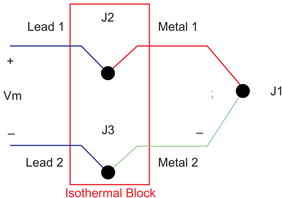
Figure 3. Isothermal Block for Absolute Temperature Measurement
