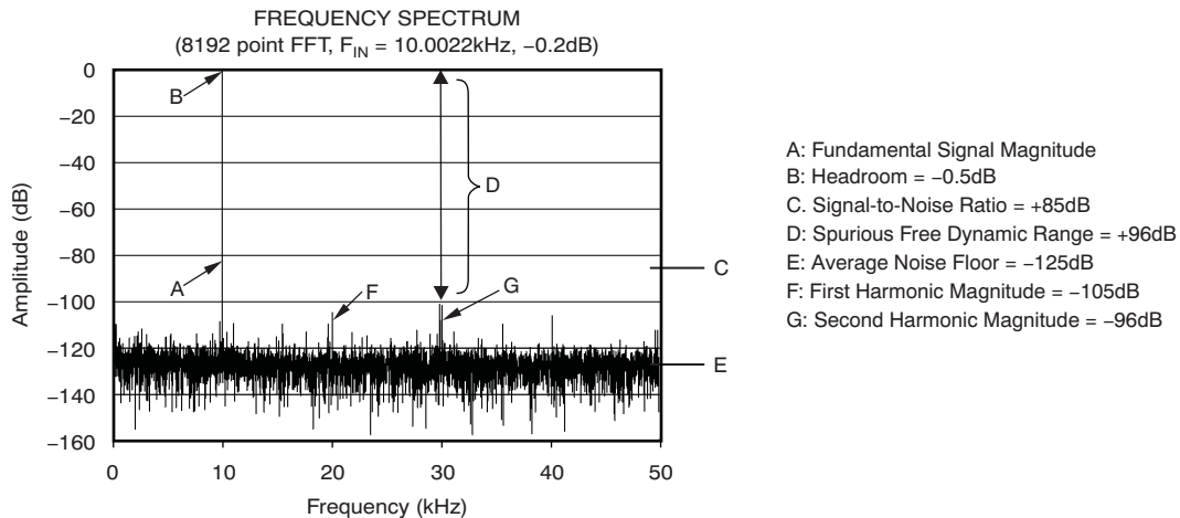
Figure 11. Dynamic Specifications (FFT Plot)
