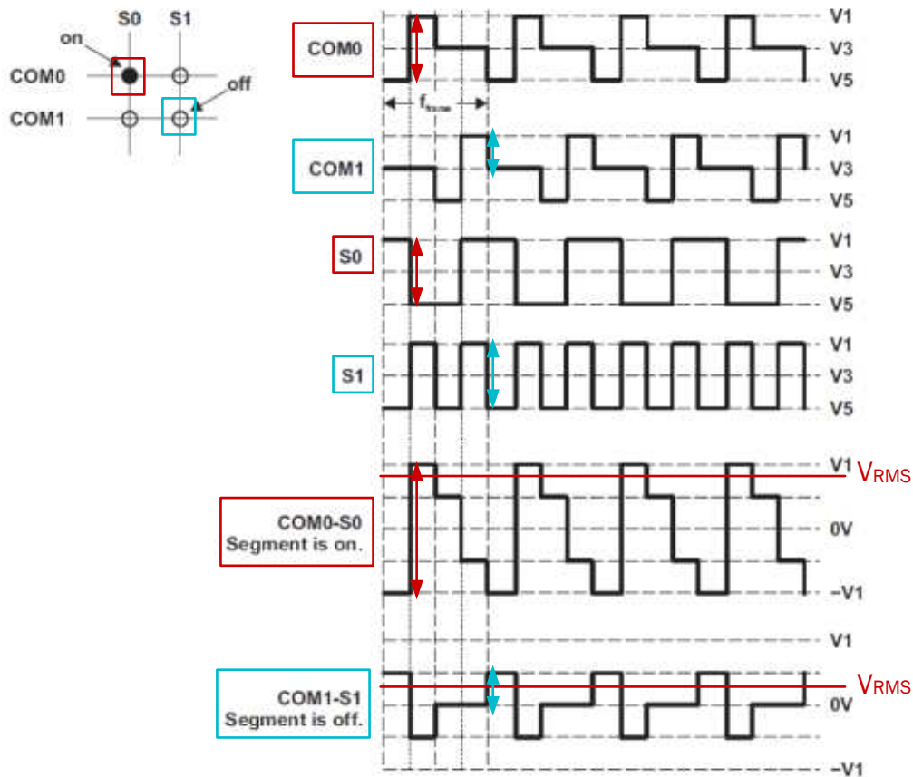
Figure 4. 2-Mux Example
