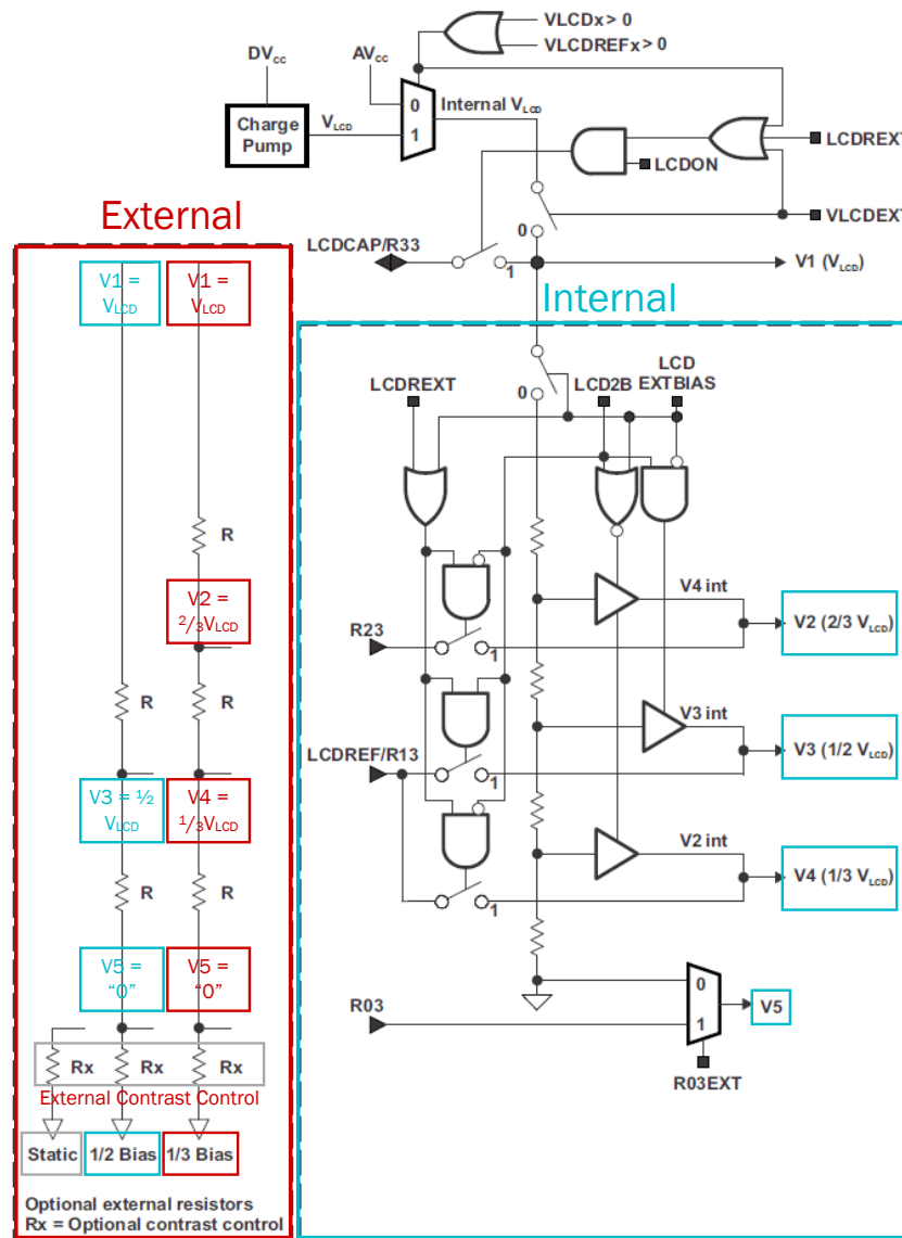
Figure 6. Bias Configurations
