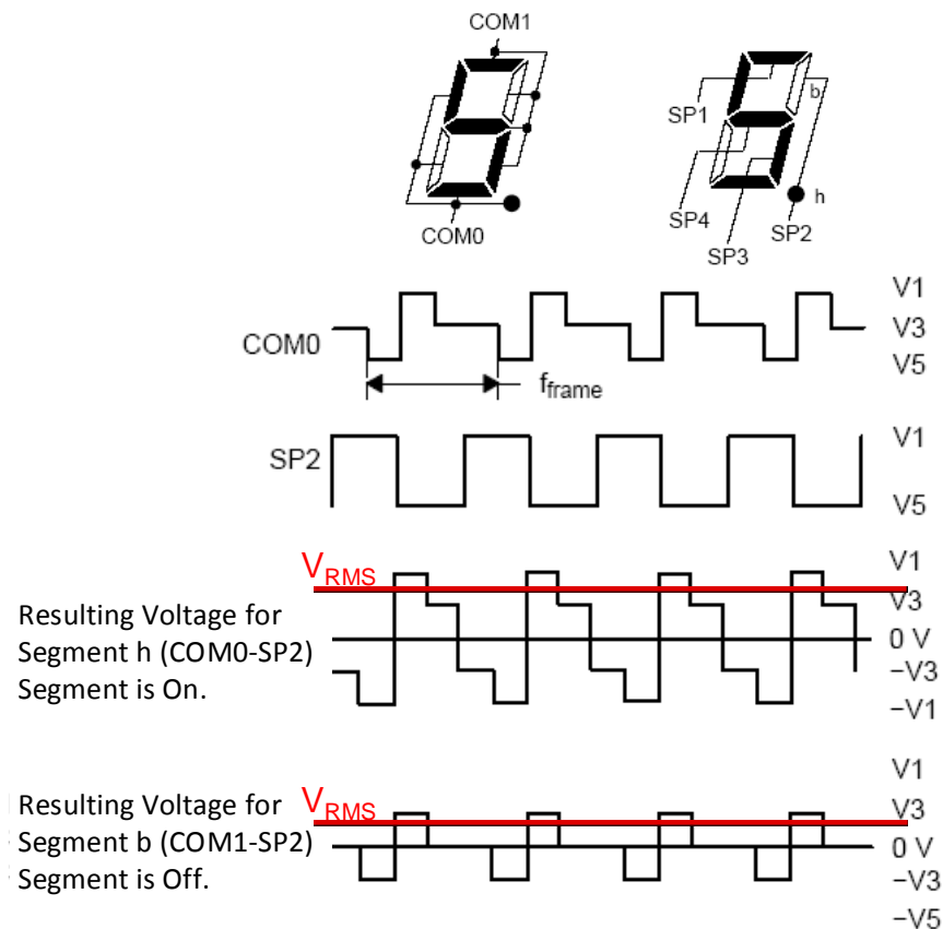
Figure 2. Example LCD AC Waveforms
