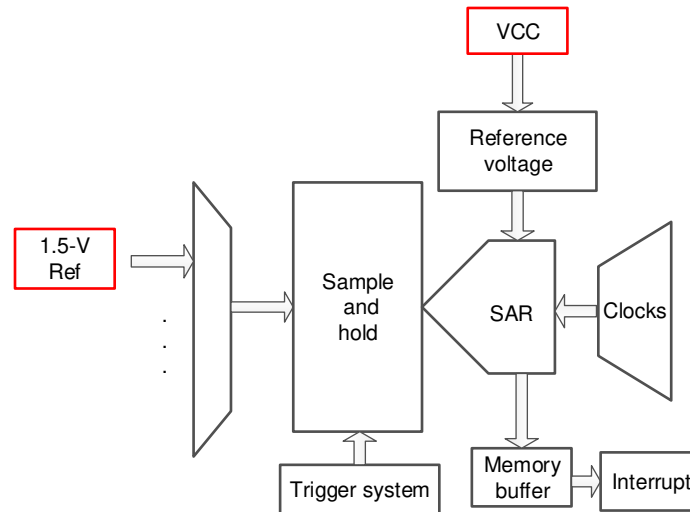
Figure 1-1. On-Chip Measurement of Battery Voltage Diagram
