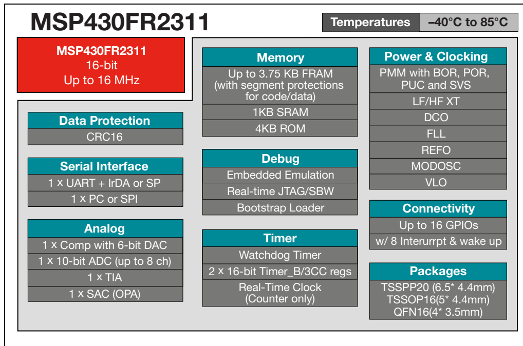
Figure 1. MSP430FR2311 MCU block diagram
